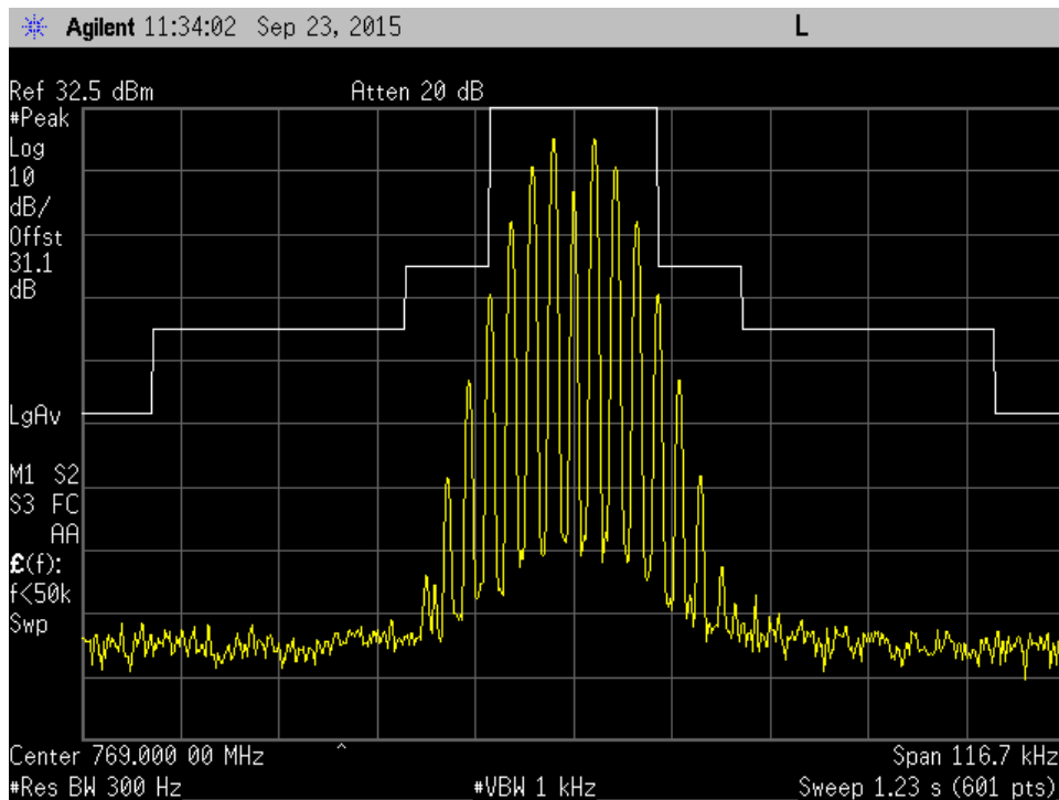
25KHz 769MHz Mod out Mask B
