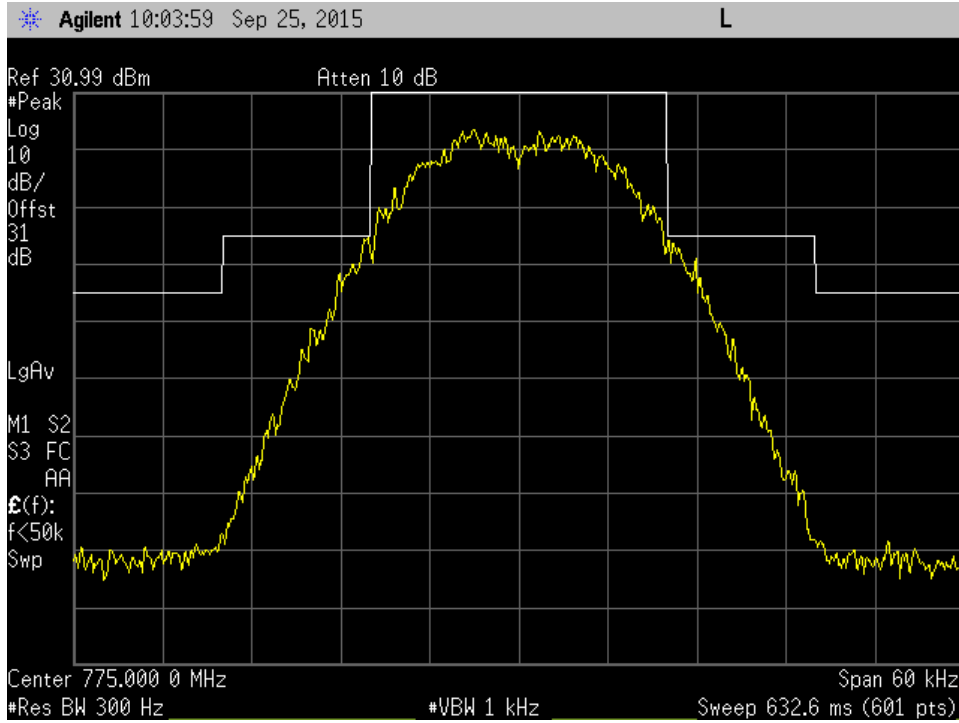
C4FM 775MHz Mod out mask C +3dB
