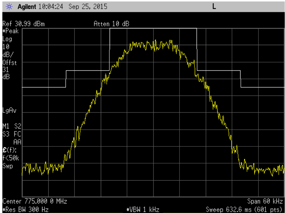
C4FM 775MHz Mod out mask B +3dB
