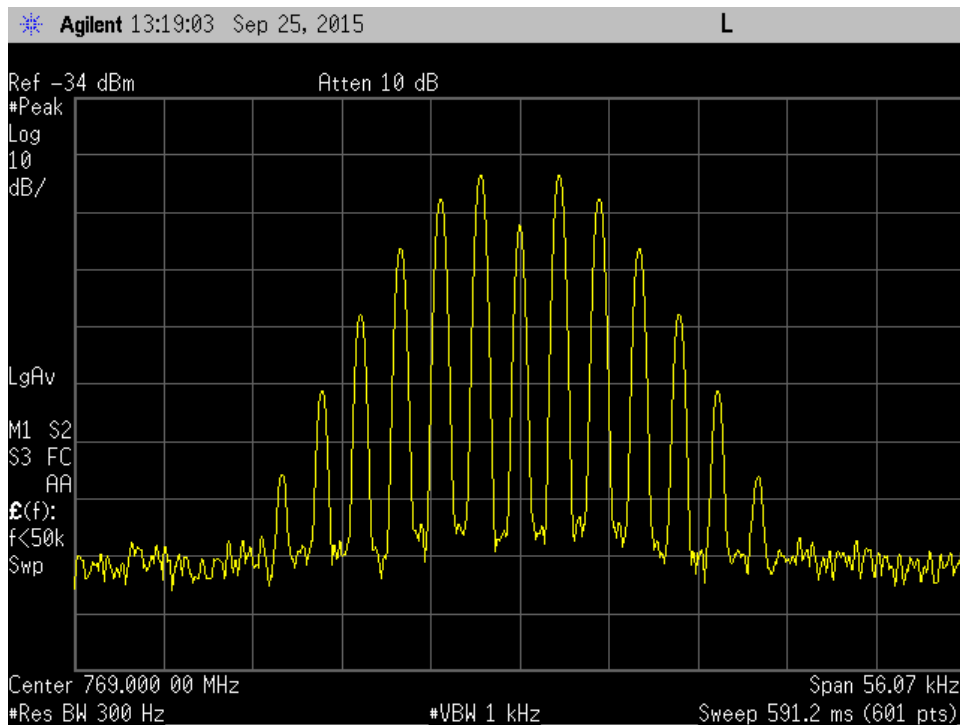
25kHz 769MHz Mod in
