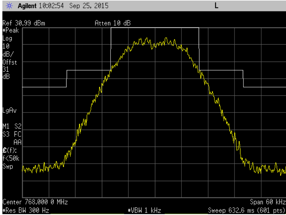
C4FM 768MHz Mod out mask B
