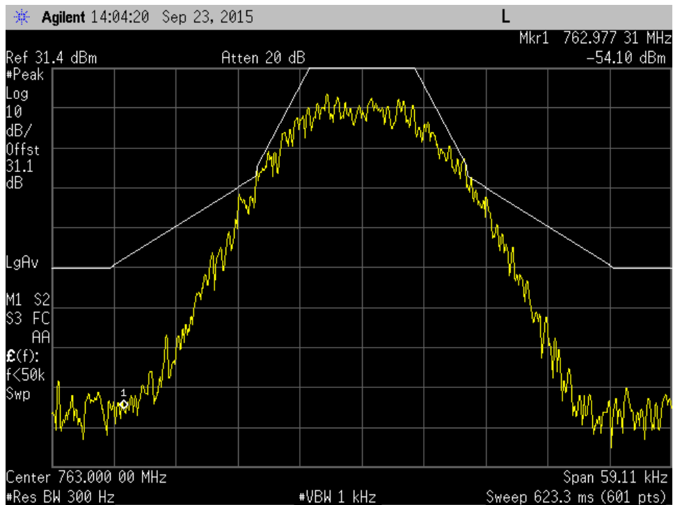
C4FM 763MHz Mod out mask C +3dB
