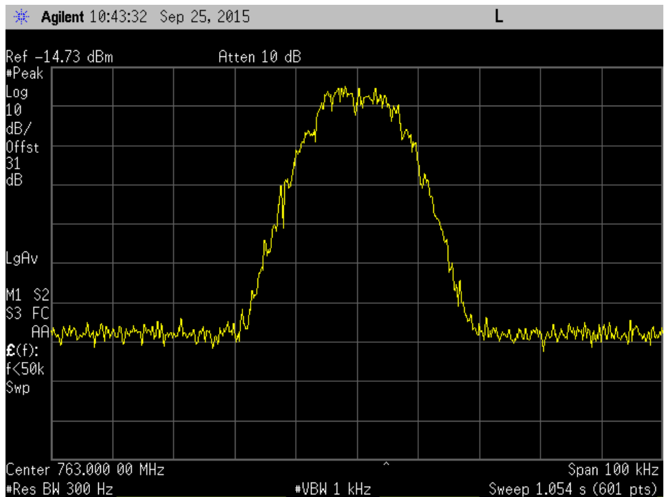
C4FM 763MHz wide band Mod in
