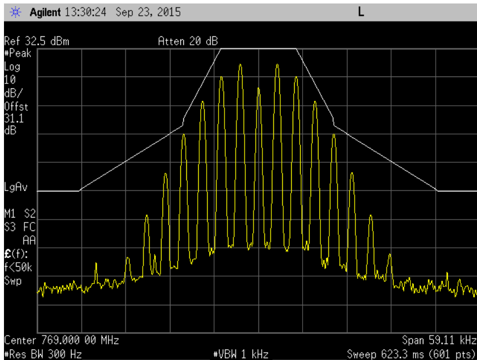
25KHz 769MHz Mod out mask C
