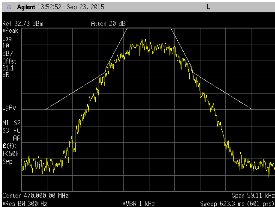
C4FM 470MHz Mod out mask C +3dB
