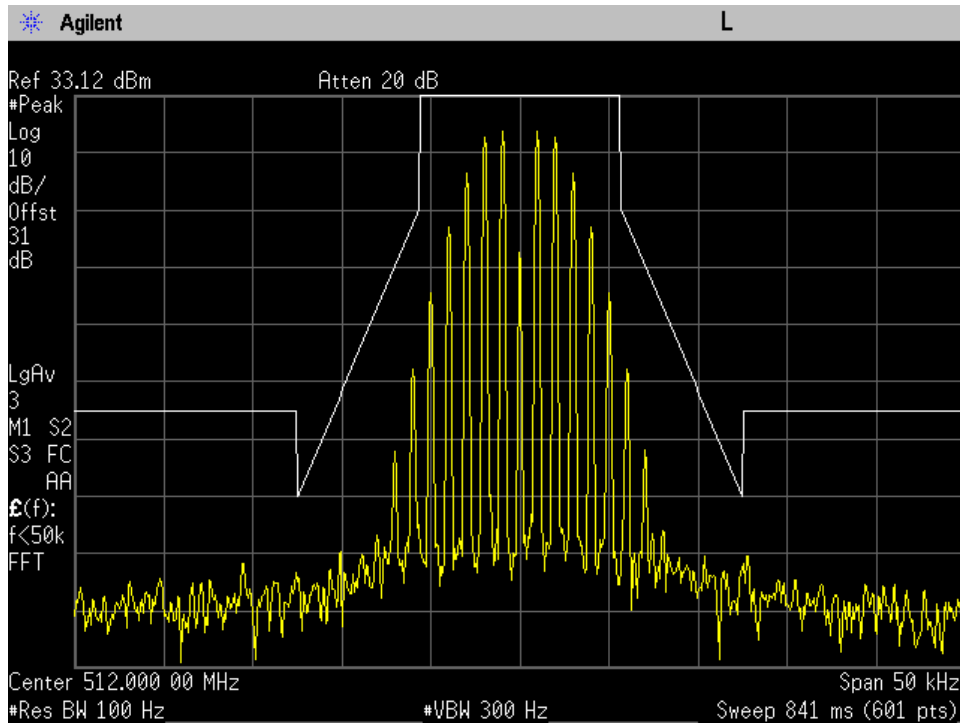
12.5KHz 512MHz Mod outMask D
