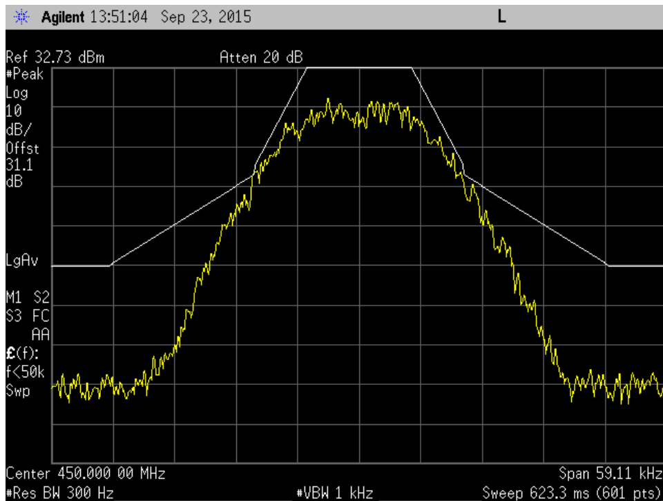
C4FM 450MHz Mod out mask C
