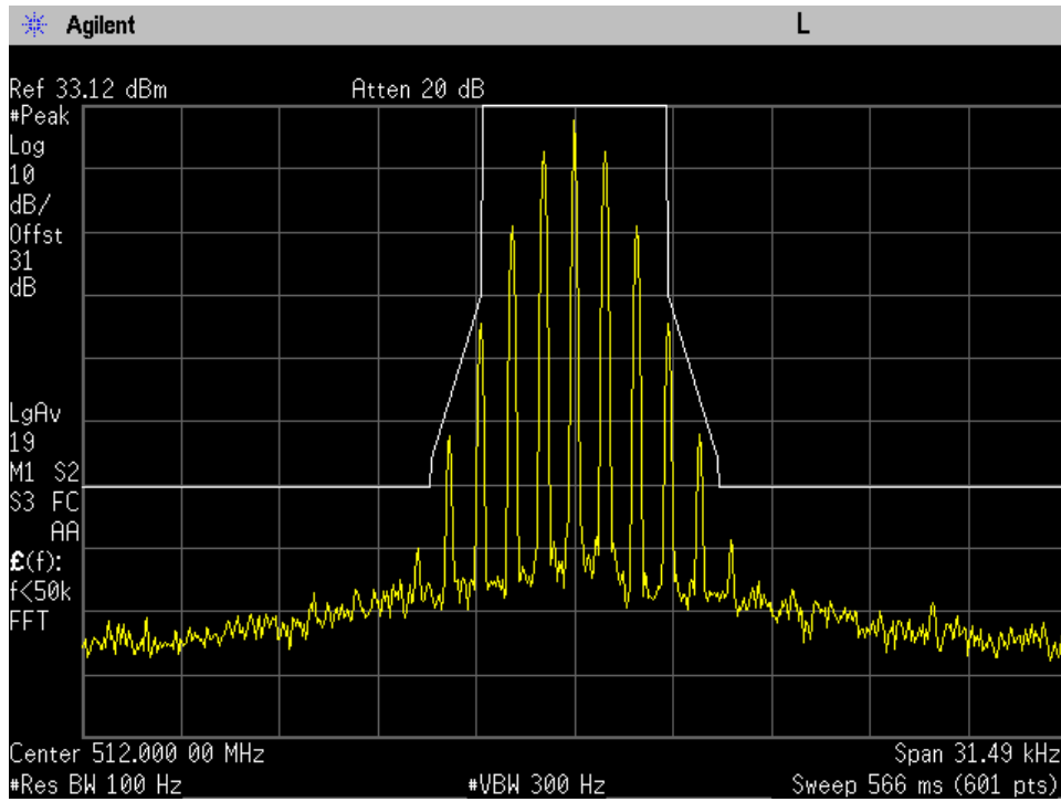
6.25KHz 512MHz Mod outMask E
