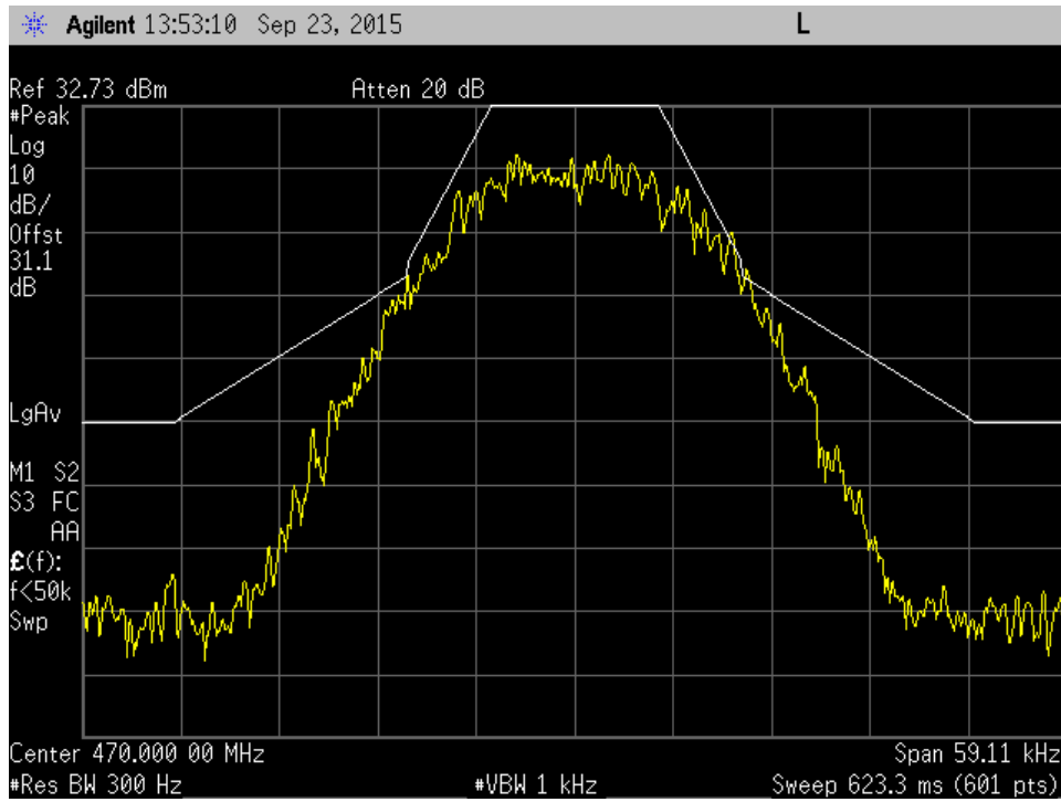
C4FM 470MHz wide band Mod in
