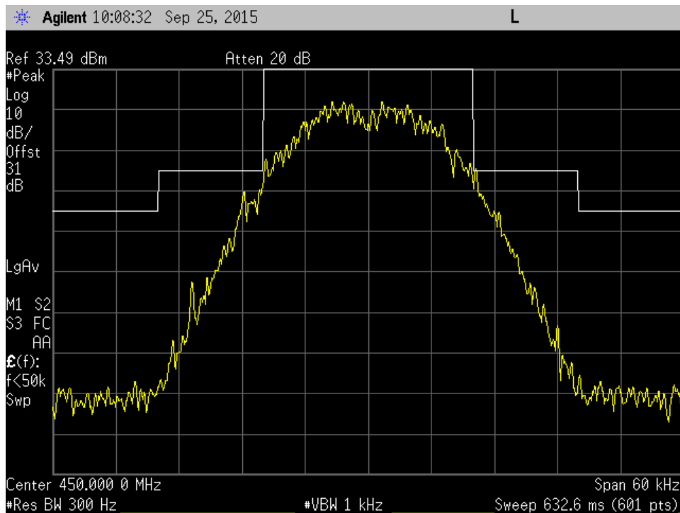
C4FM 450MHz Mod out mask B
