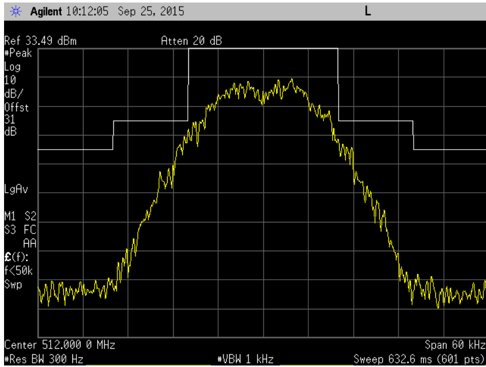
C4FM 512MHz Mod out mask C +3dB
