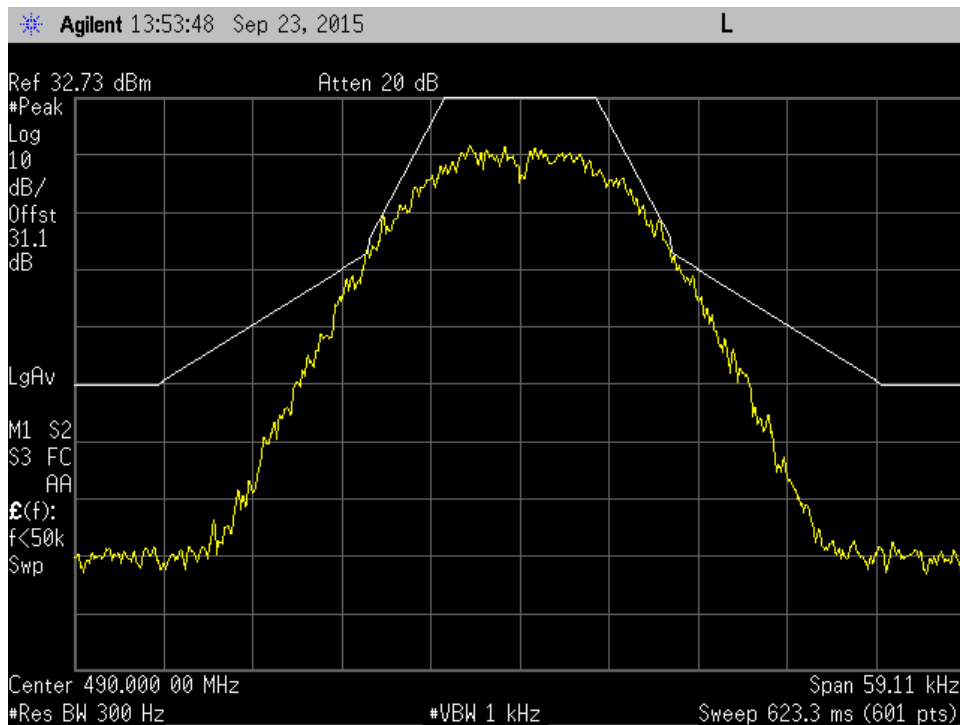
C4FM 490MHz Mod out mask C
