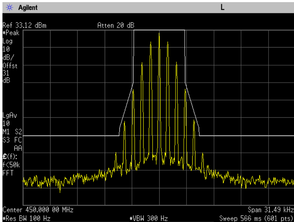
6.25KHz 450MHz Mod out Mask E +3dB
