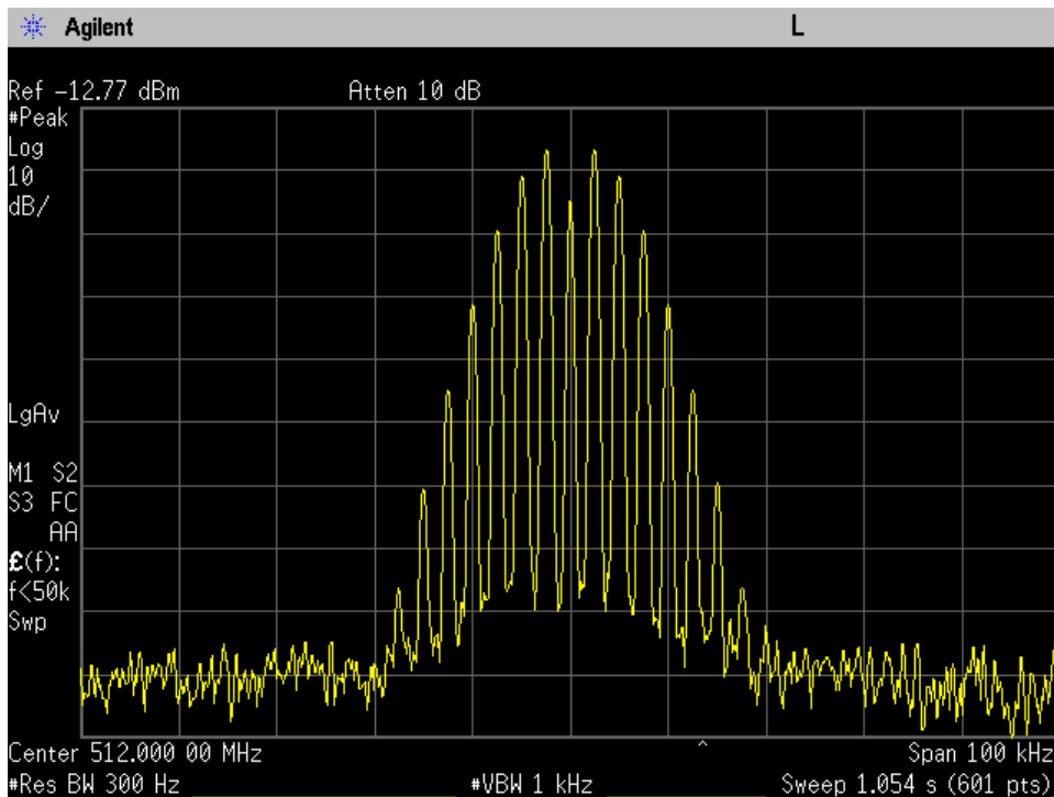
25KHz 512MHz Mod in
