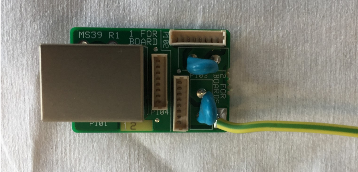
Eth top
