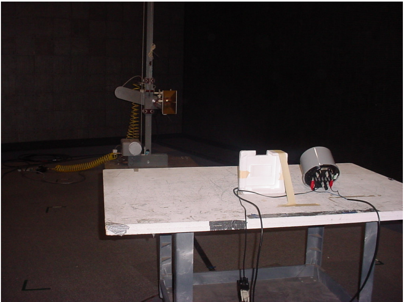
Figure 5: Test Setup Radiated Emissions – Intentional
