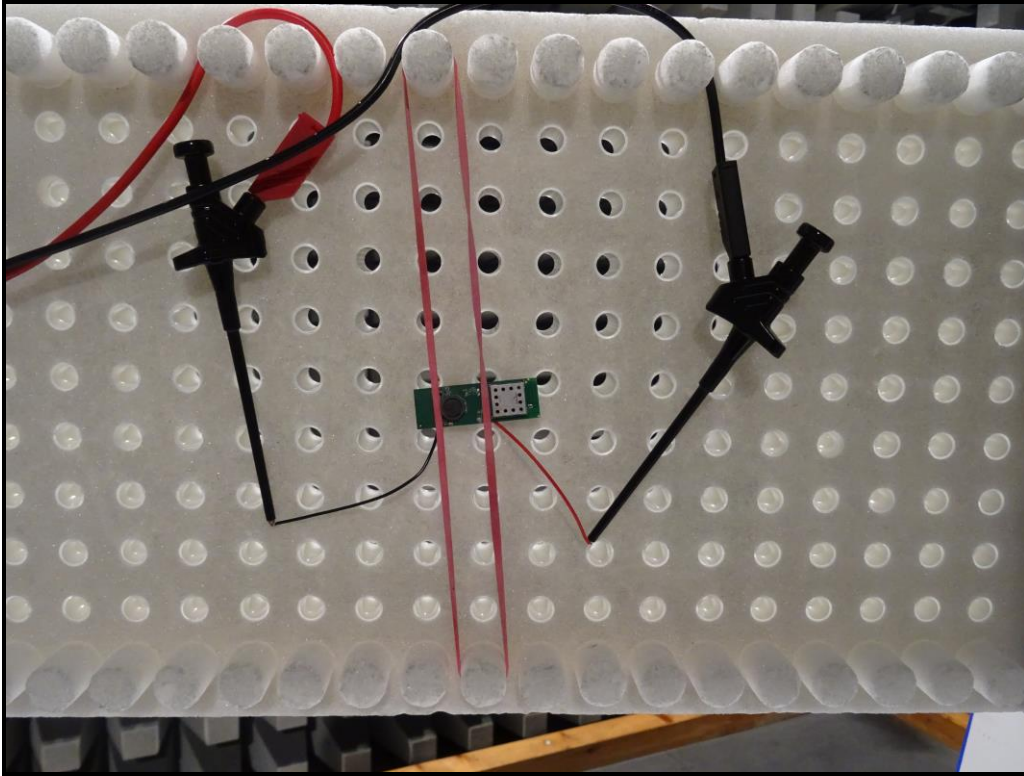
Photo 3: Radiated Test Sample-Close view- NOXBLEMOD Module (with Shielding)
