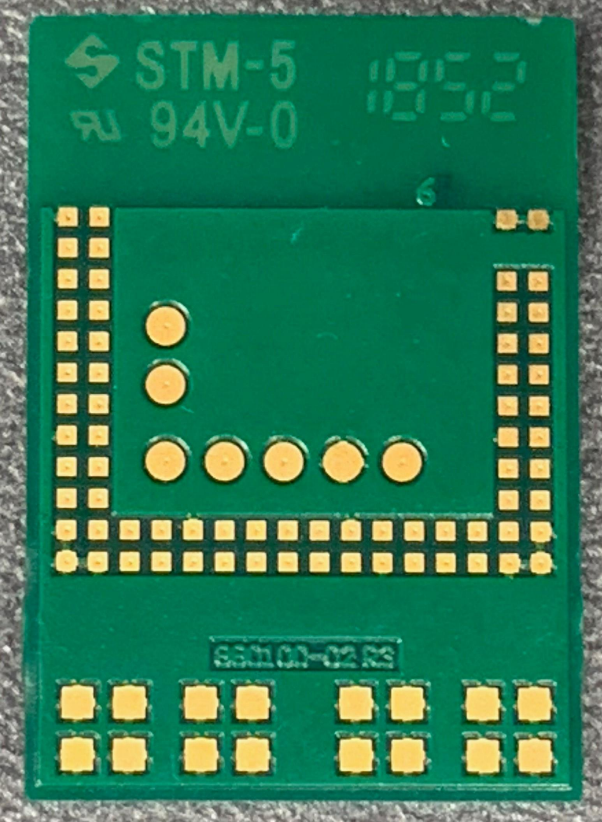
Figure 2 – Bottom of Nox Bluetooth Module
