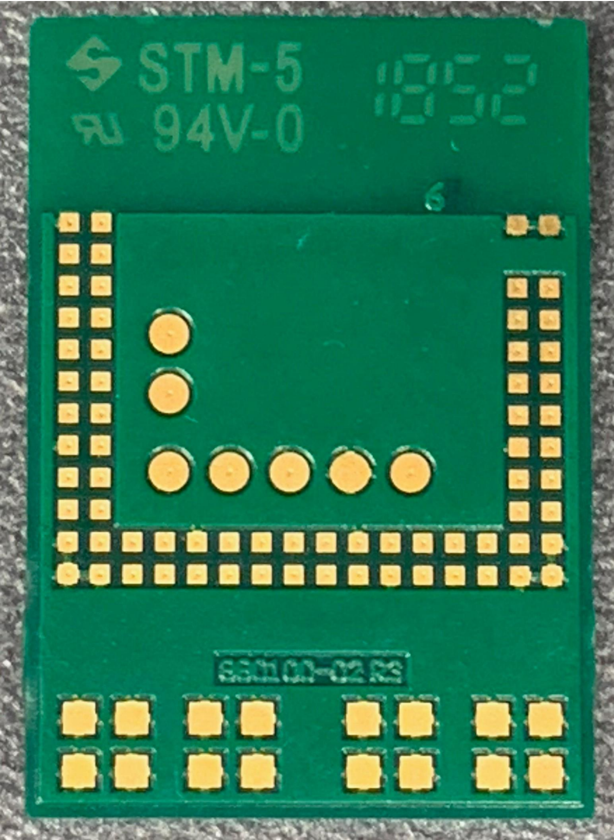
Figure 2 – Bottom of Nox Bluetooth LE Module
