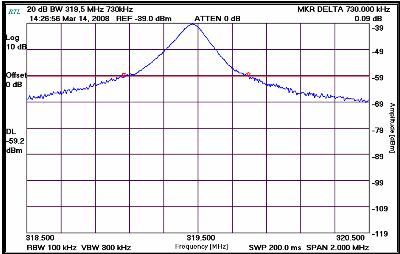
Plot 6-1: Modulated Bandwidth – 319.5 MHz
