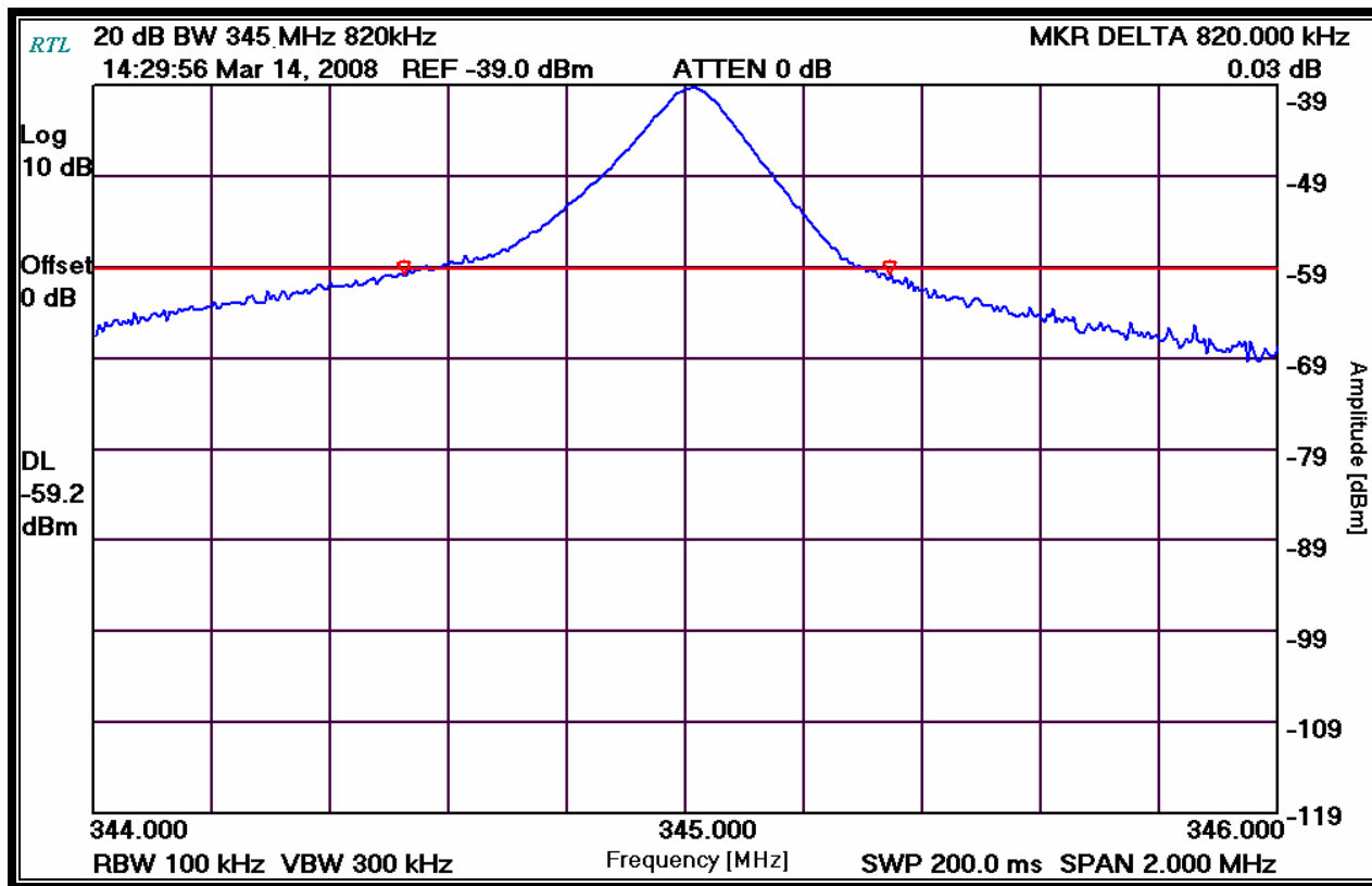
Plot 6-2: Modulated Bandwidth – 345.0 MHz
