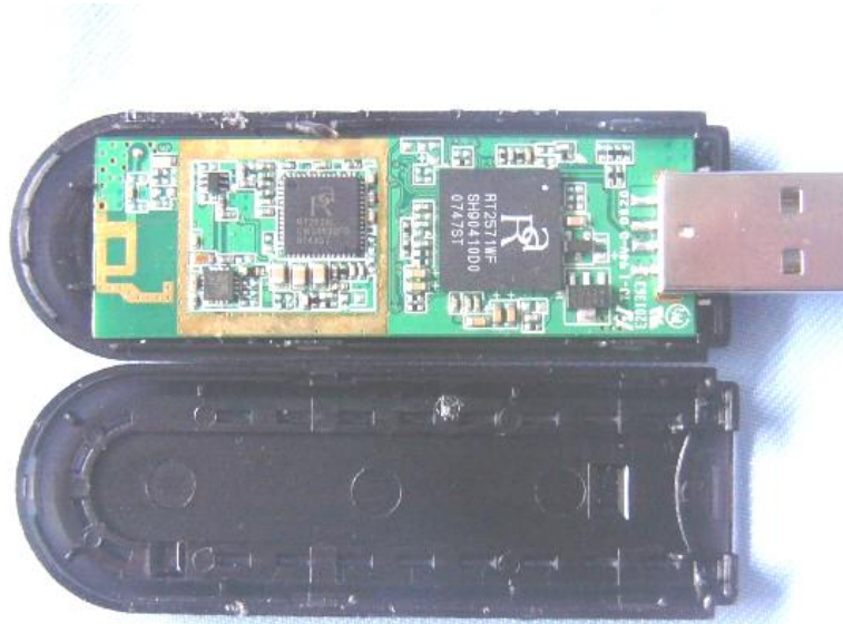
EUT inside whole view
