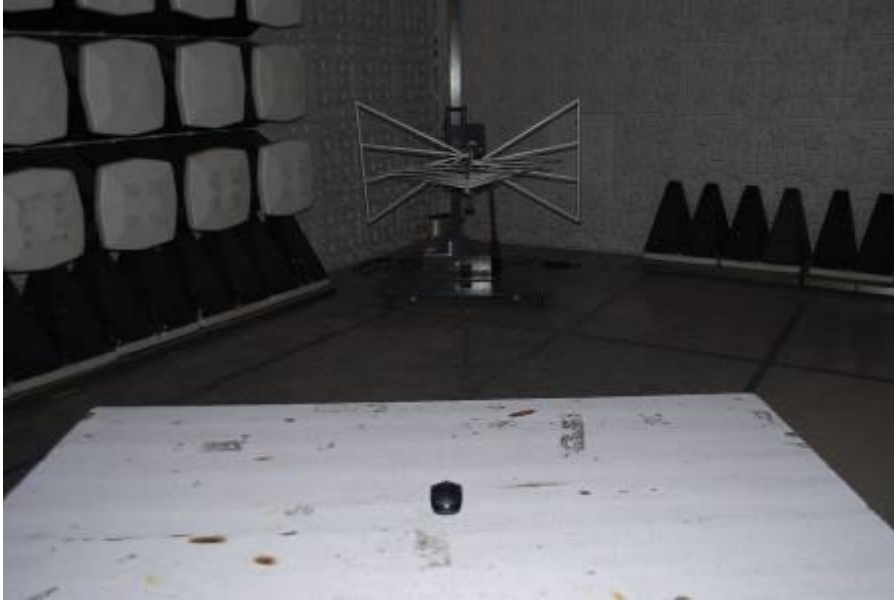
Radiated Emission
