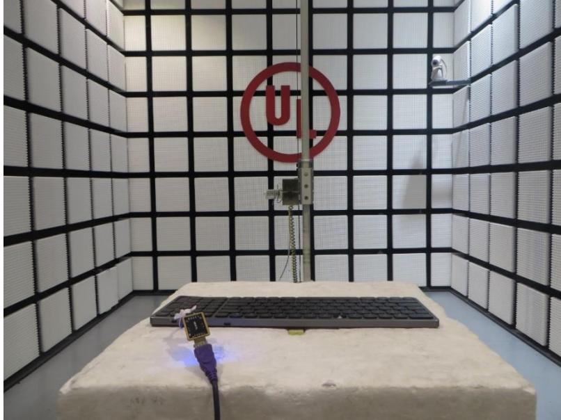
MEASUREMENT POSITION for BT/BLE
