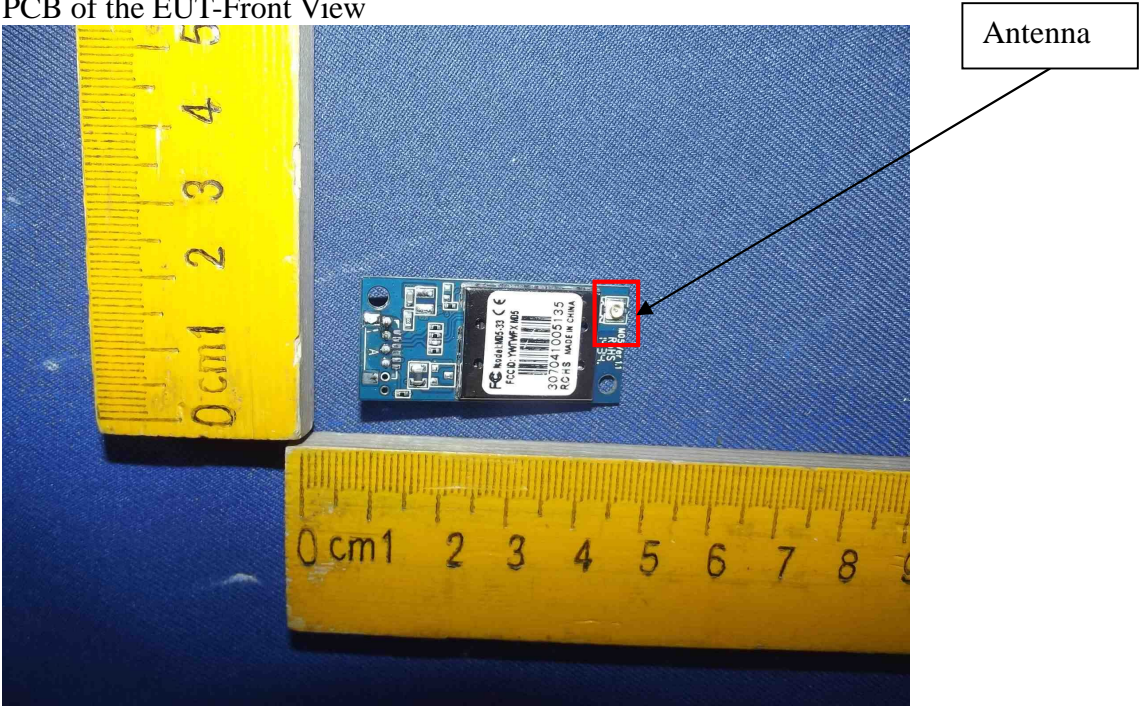
Figure 15 PCB of the EUT-Front View
