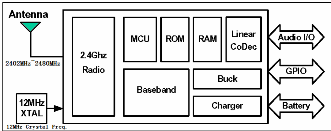
H201 Block Diagram
