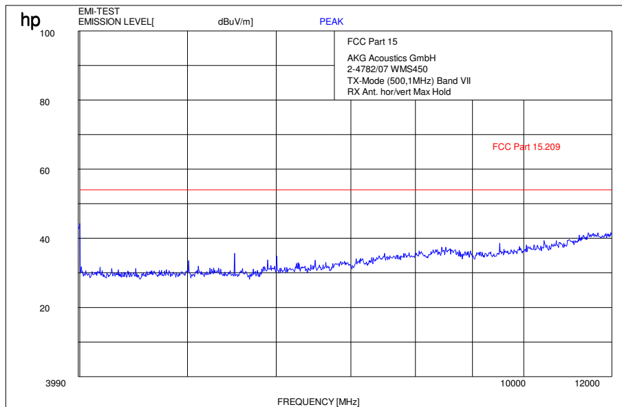
Plot 3: 4 GHz – 12 GHz, Band VII, low channel 500.10 MHz
