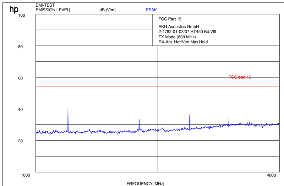
Plot 17: 1 GHz – 4GHz, Band VIII, high channel 600.00 MHz
