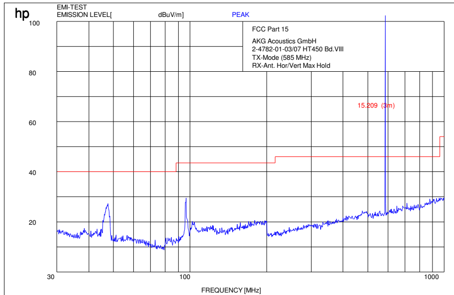
Plot 13: 30 MHz – 1GHz, Band VIII, mid channel 585.00 MHz
