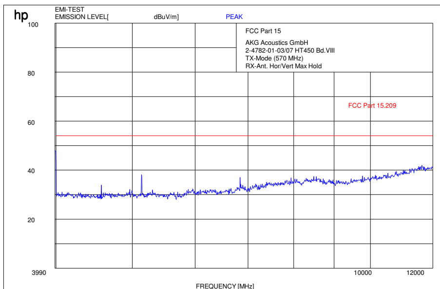
Plot 12: 4 GHz – 12 GHz, Band VIII, low channel 570.00 MHz
