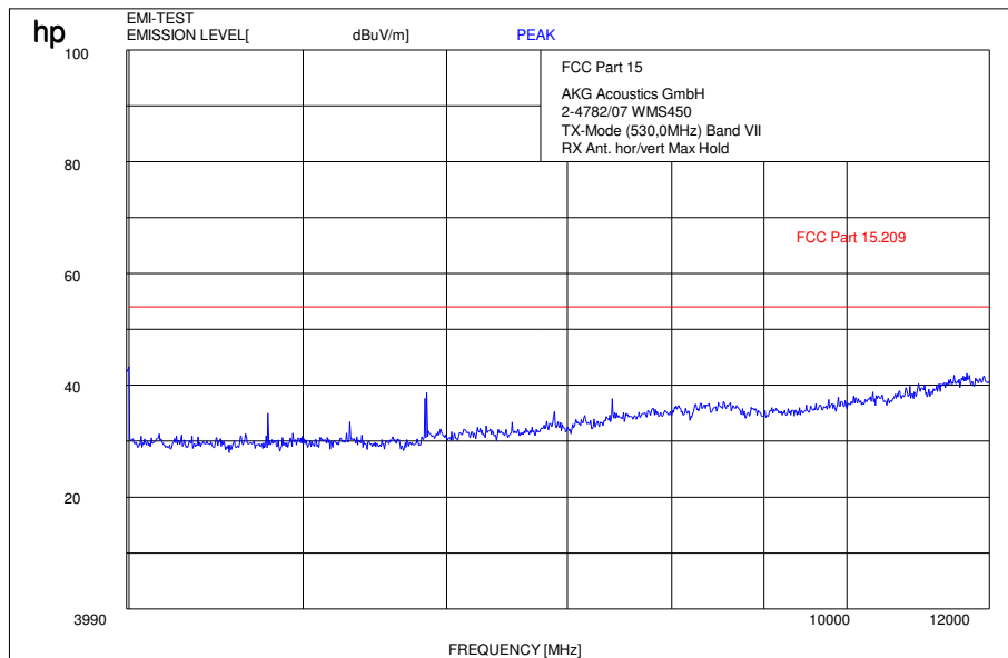
Plot 9: 4 GHz – 12 GHz, Band VII, high channel 530.00 MHz
