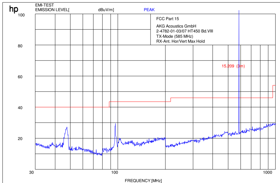
Plot 13: 30 MHz – 1GHz, Band VIII, mid channel 585.00 MHz
