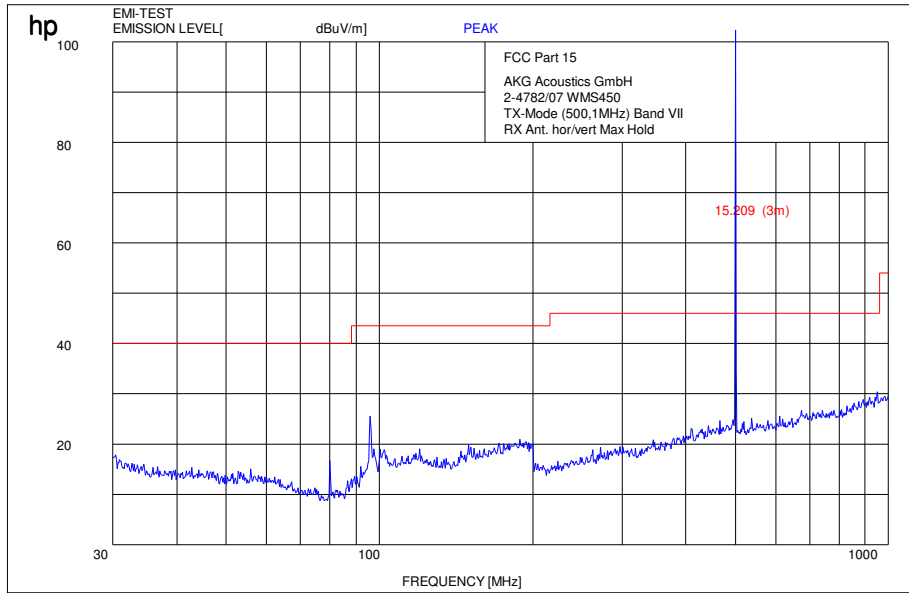
Plot 1: 30 MHz – 1GHz, Band VII, low channel 500.10 MHz
