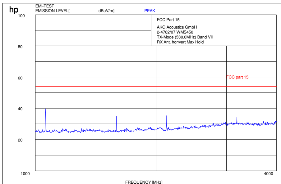
Plot 8: 1 GHz – 4GHz, Band VII, high channel 530.00 MHz
