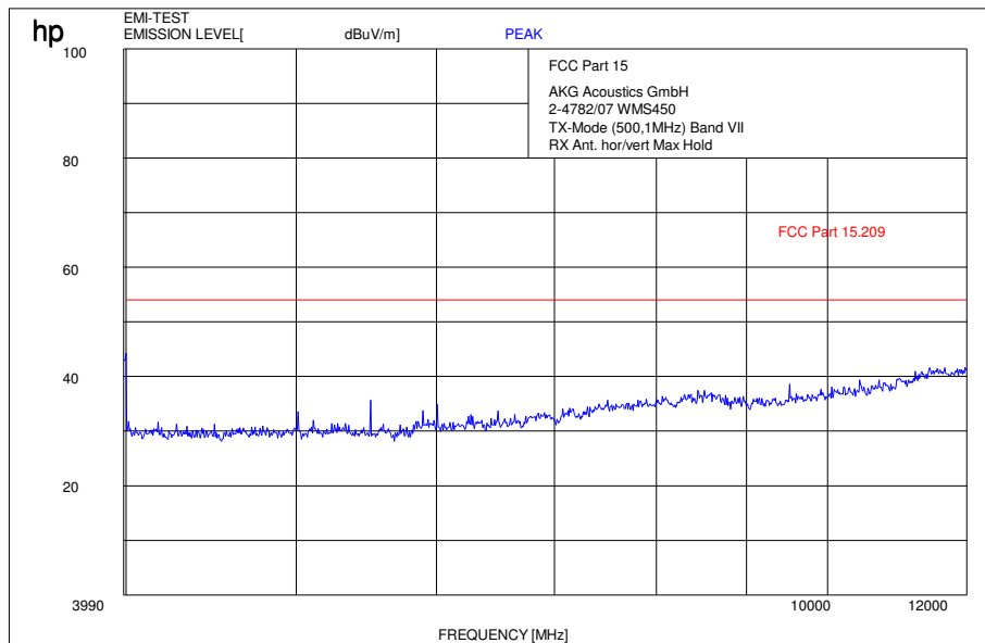
Plot 3: 4 GHz – 12 GHz, Band VII, low channel 500.10 MHz
