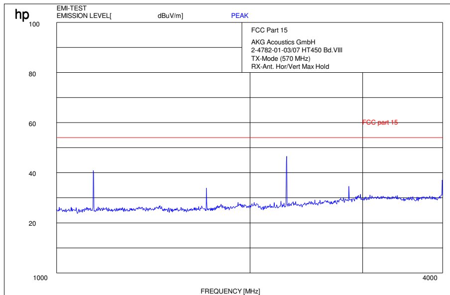
Plot 11: 1 GHz – 4GHz, Band VIII, low channel 570.00 MHz
