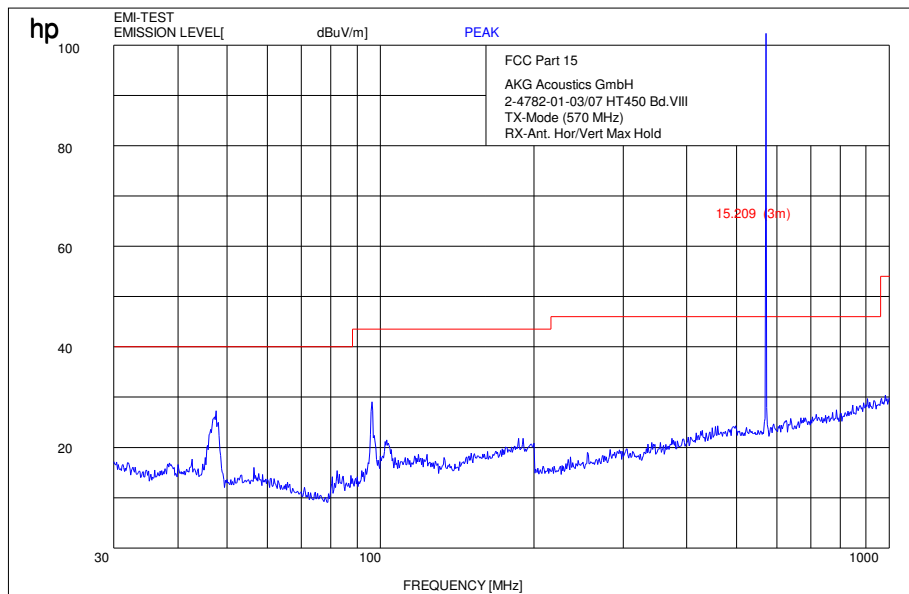
Plot 10: 30 MHz – 1GHz, Band VIII, low channel 570.00 MHz
