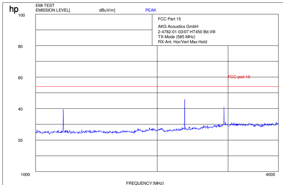
Plot 14: 1 GHz – 4GHz, Band VIII, mid channel 585.00 MHz
