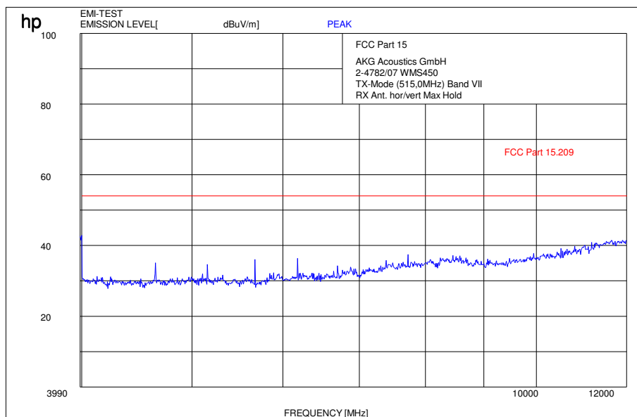
Plot 6: 4 GHz – 12 GHz, Band VII, mid channel 515.00 MHz
