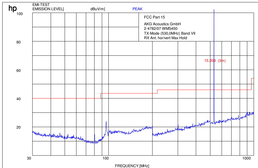
Plot 7: 30 MHz – 1GHz, Band VII, high channel 530.00 MHz
