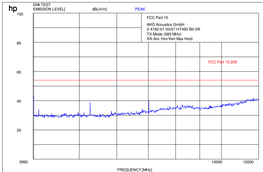
Plot 15: 4 GHz – 12 GHz, Band VIII, mid channel 585.00 MHz
