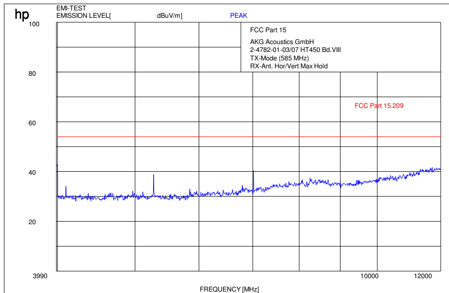
Plot 15: 4 GHz – 12 GHz, Band VIII, mid channel 585.00 MHz
