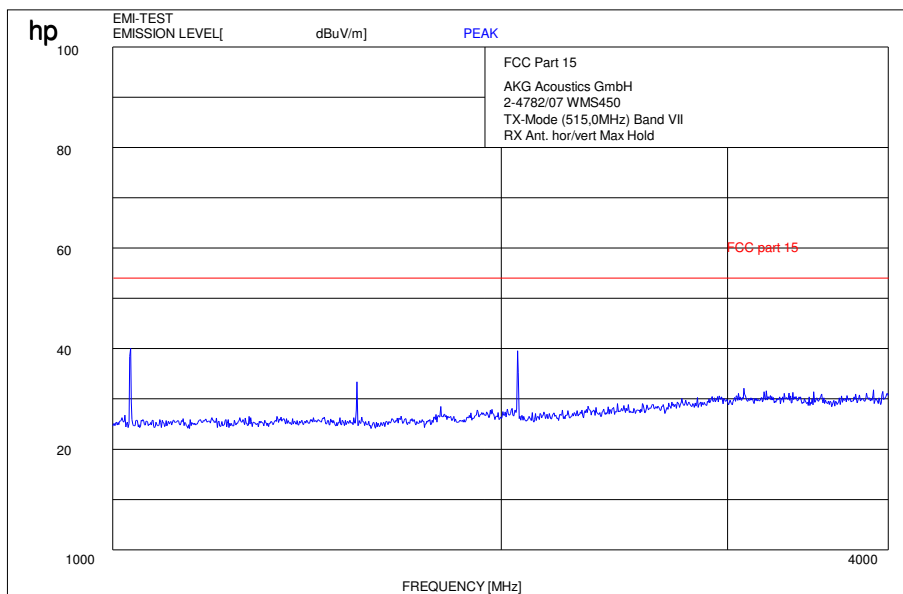
Plot 5: 1 GHz – 4GHz, Band VII, mid channel 515.00 MHz
