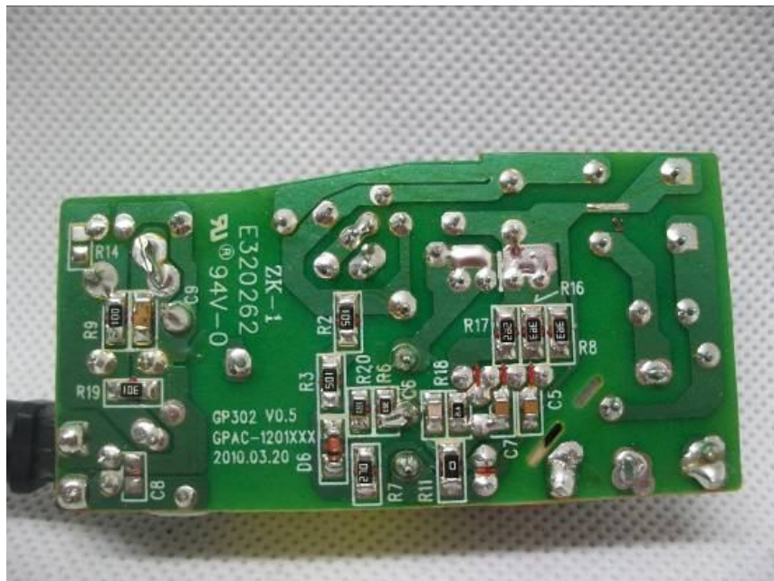
INTERNAL PHOTO OF POWER SUPPLY1 - 2
