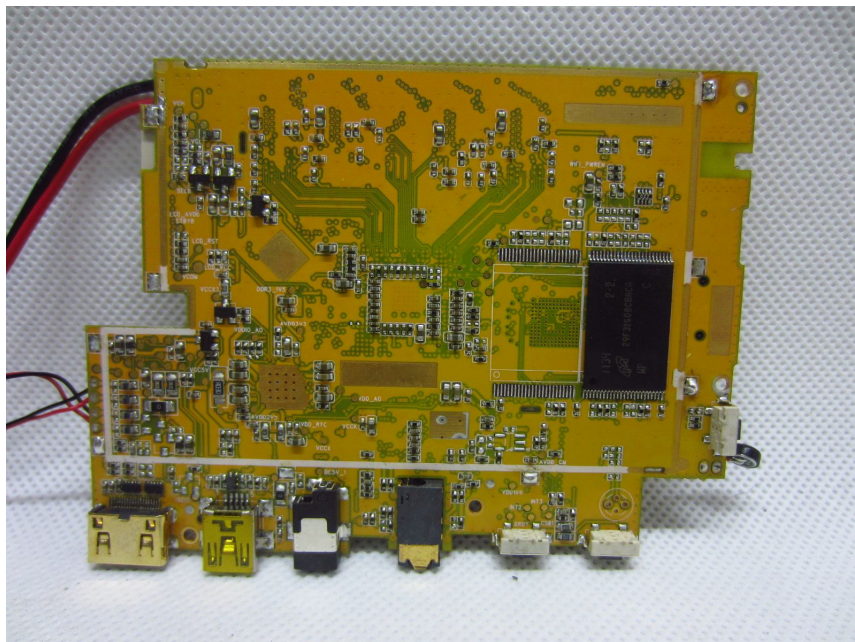
INTERNAL PHOTO OF SAMPLE - 13
