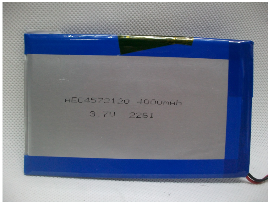
INTERNAL PHOTO OF SAMPLE - 15
