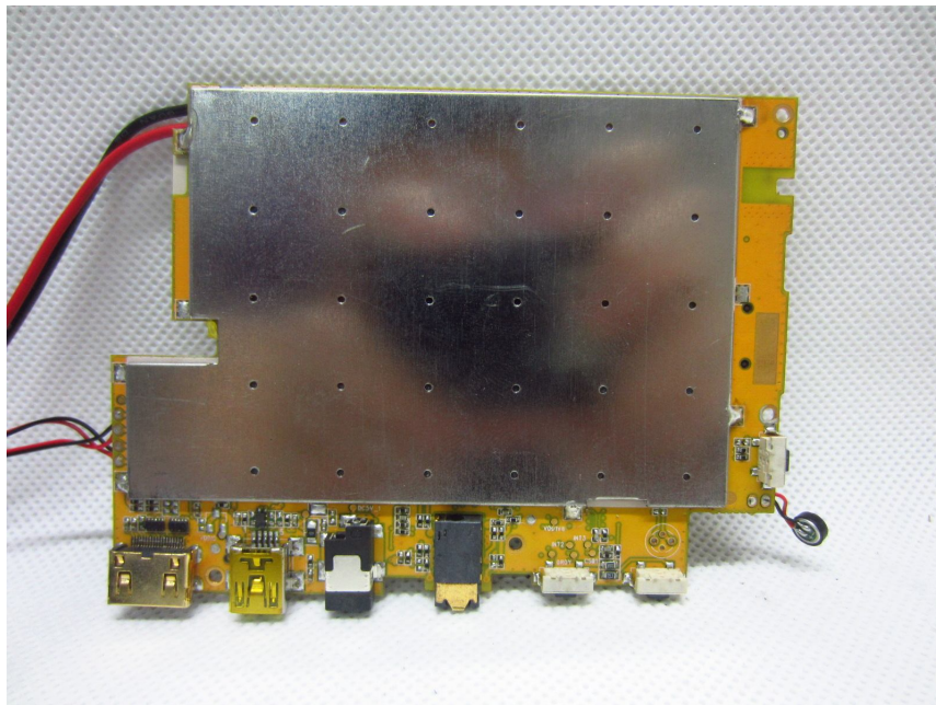
INTERNAL PHOTO OF SAMPLE - 11
