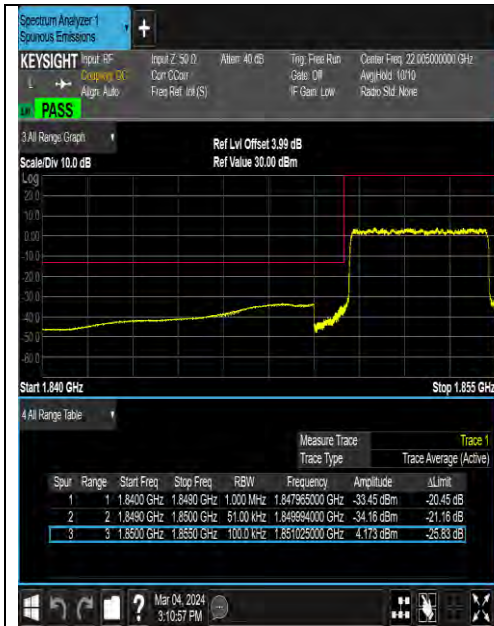
NTNV-N25-PC3-15-5-L-DFT-QPSK-Outer_Full-Ant0-PASS
