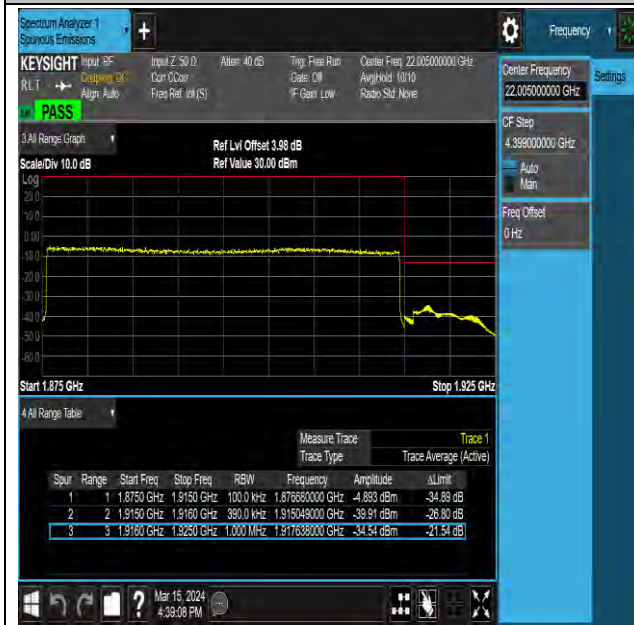
NTVN-N25-PC3-15-40-H-DFT-QPSK-Outter_Full-Ant0-PASS
