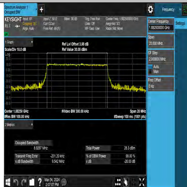
NTNV-N25-PC3-15-10-M-DFT-16QAM-Outer_Full-Ant0- PASS
