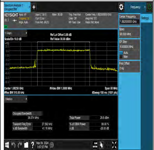
NTNV-N25-PC3-15-40-M-DFT-QPSK-Outer_Full-Ant0- PASS
