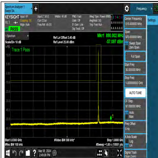
NTNV-N13-PC3-15-5-H-DFT-QPSK-Edge_1RB_Left- Ant0-PASS
