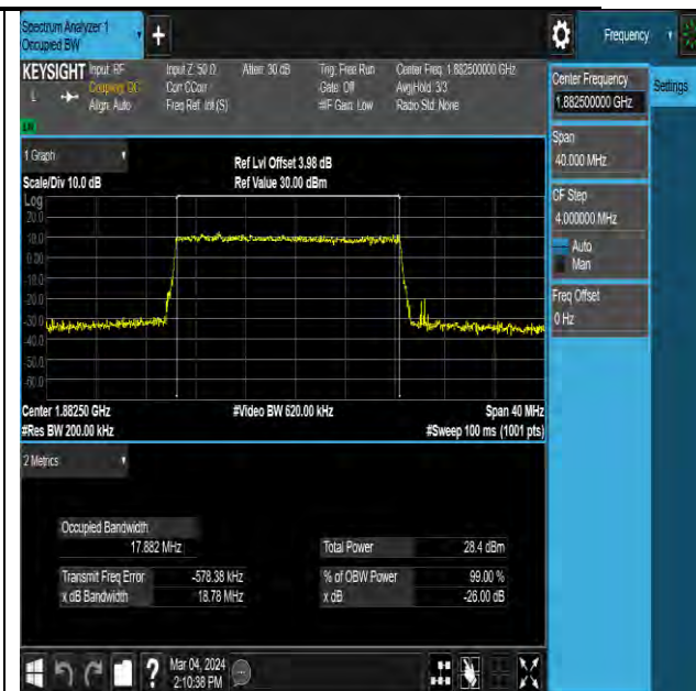
NTNV-N25-PC3-15-20-M-DFT-16QAM-Outer_Full-Ant0-PASS
