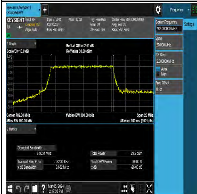
NTNV-N13-PC3-15-10-M-DFT-QPSK-Outer_Full-Ant0- PASS
