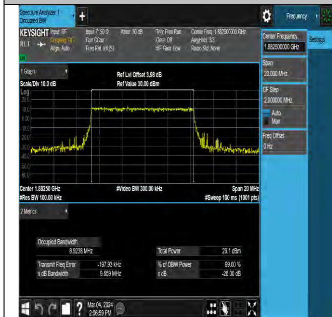
NTNV-N25-PC3-15-10-M-DFT-QPSK-Outer_Full-Ant0-PASS
