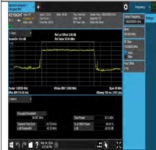
NTNV-N25-PC3-15-40-M-DFT-PI2BPSK-Outer_Full-Ant0- PASS
