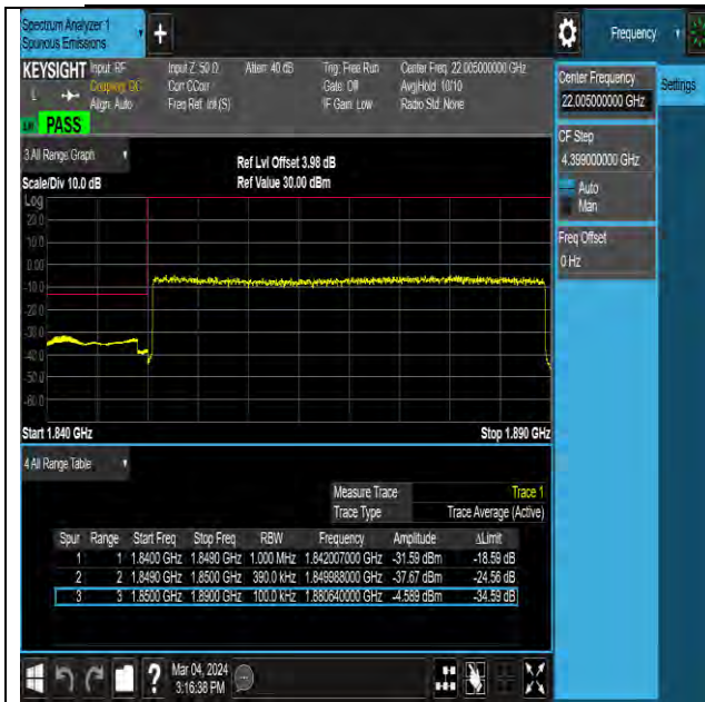
NTVN-N25-PC3-15-40-L-DFT-QPSK-Outter_Full-Ant0-PASS
