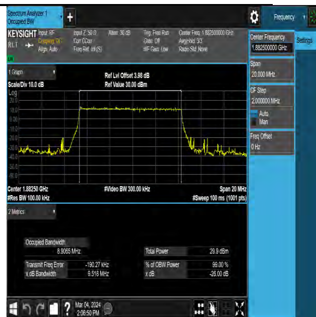
NTNV-N25-PC3-15-10-M-DFT-PI2BPSK-Outer_Full- Ant0-PASS
