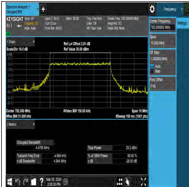
NTNV-N13-PC3-15-5-M-DFT-PI2BPSK-Outter_Full-Ant0- PASS
