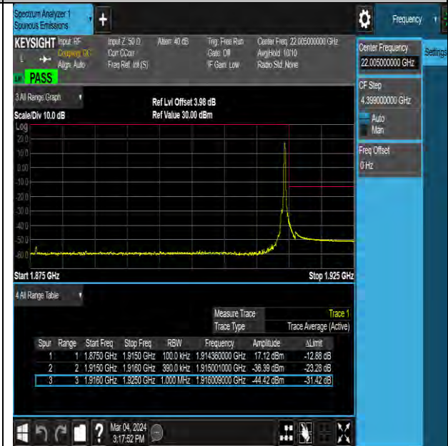
NTVN-N25-PC3-15-40-H-DFT-QPSK-Edge_1RB_Right-Ant0-PASS
