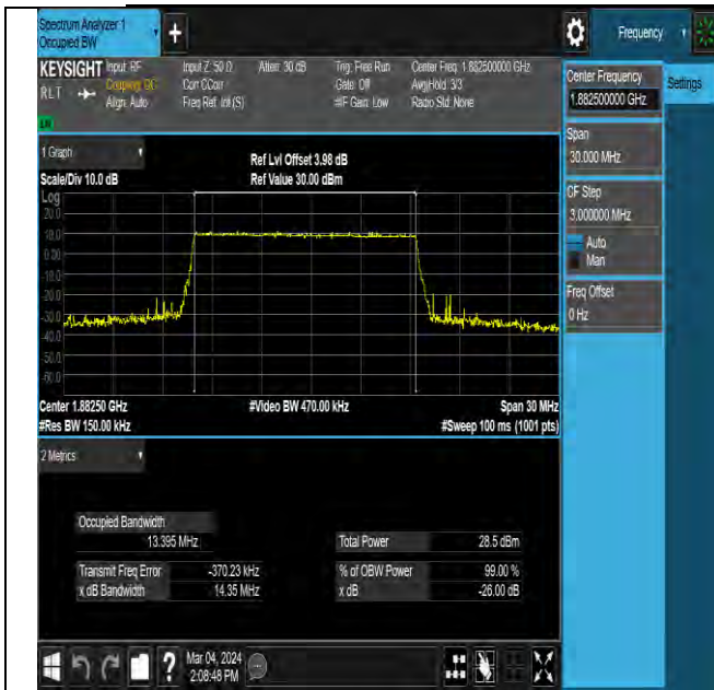
NTNV-N25-PC3-15-15-M-DFT-16QAM-Outer_Full-Ant0- PASS
