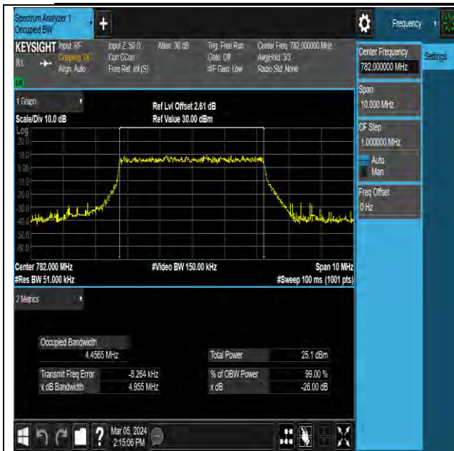
NTNV-N13-PC3-15-5-M-DFT-256QAM-Outer_Full-Ant0- PASS
