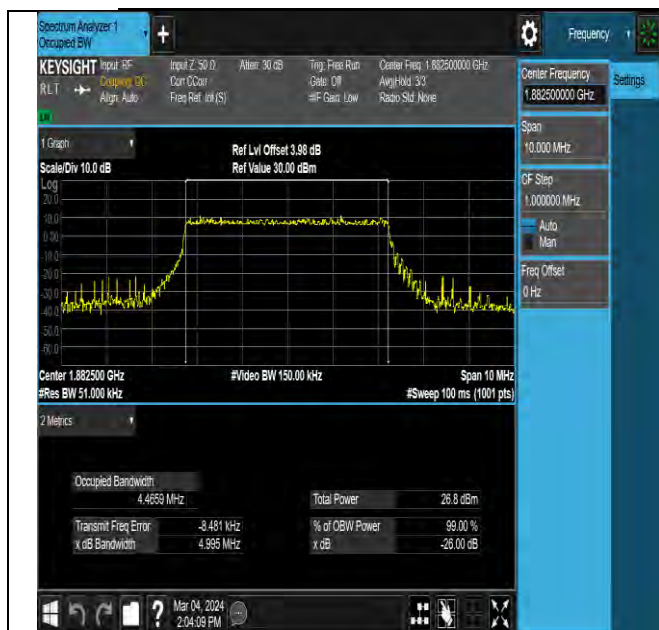
NTNV-N25-PC3-15-5-M-DFT-256QAM-Outer_Full-Ant0- PASS
