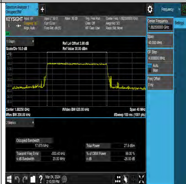
NTNV-N25-PC3-15-20-M-DFT-256QAM-Outer_Full-Ant0-PASS
