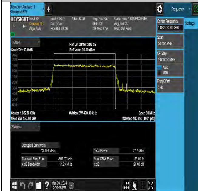
NTNV-N25-PC3-15-15-M-DFT-256QAM-Outer_Full-Ant0- PASS
