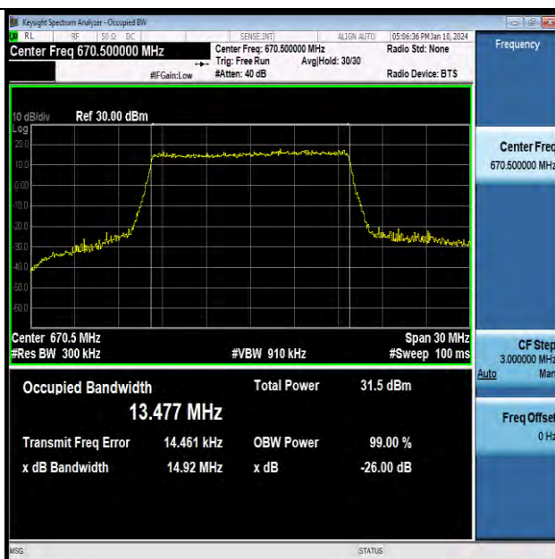
Band71-15MHz-QPSK-133197-75RB#0-PASS
