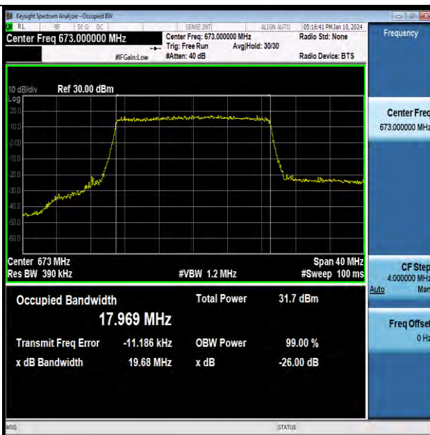
Band71-20MHz-QPSK-133222-100RB#0-PASS
