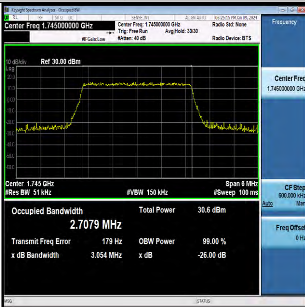
Band66-3MHz-QPSK-132322-15RB#0-PASS
