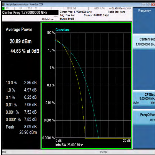
Band66-20MHz-16QAM-132572-100RB#0-PASS
