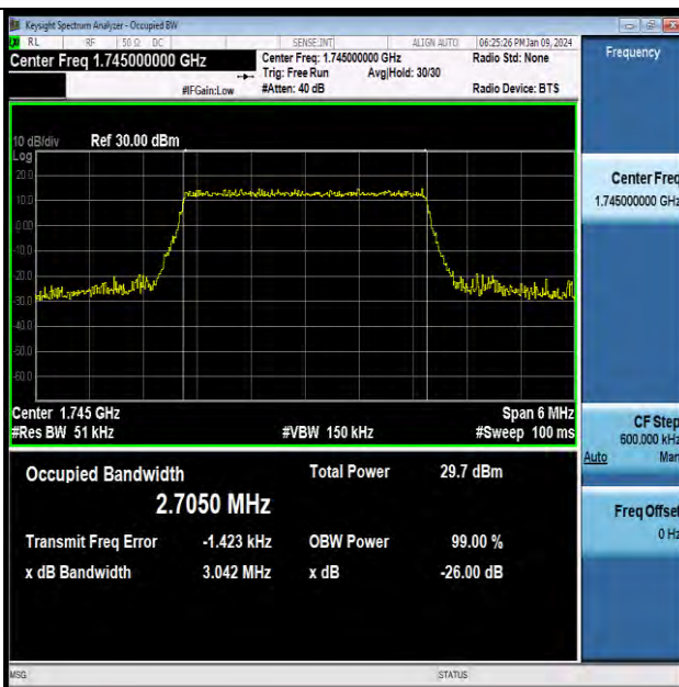
Band66-3MHz-16QAM-132322-15RB#0-PASS
