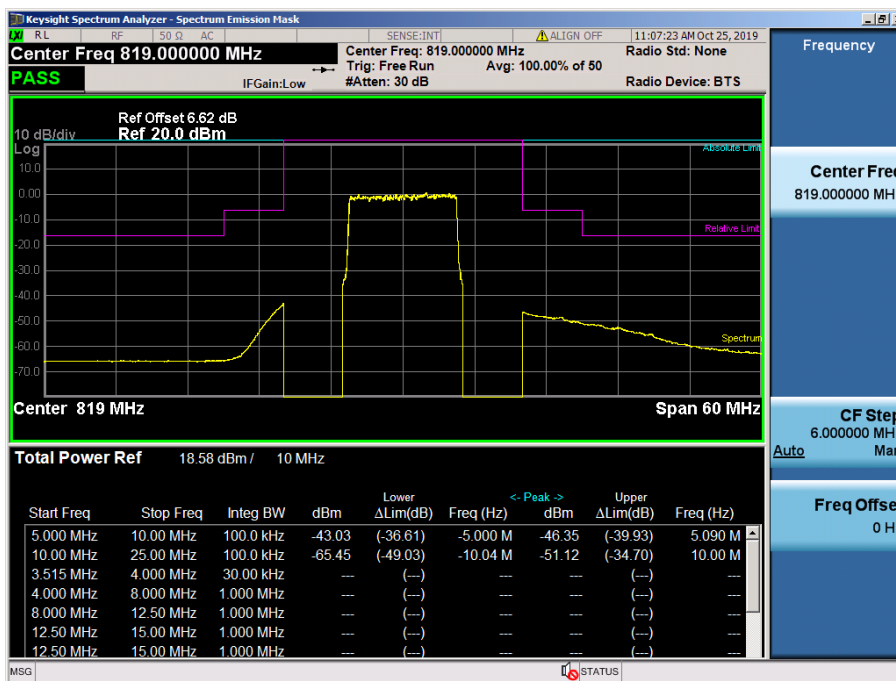
LTE Band 26 / 10MHz / 16QAM - RB Size/Offset (50/0) - Low Channel
