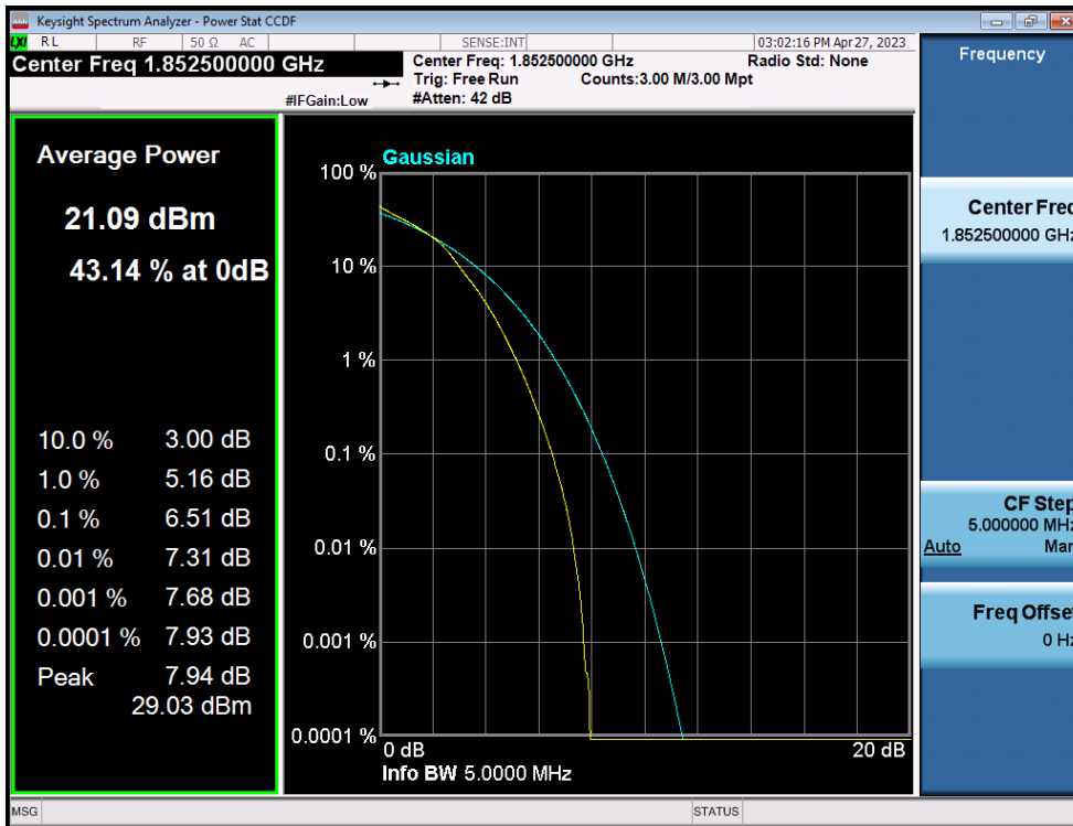
LTE Band 25(2) / 5MHz / 16QAM - RB Size 25
