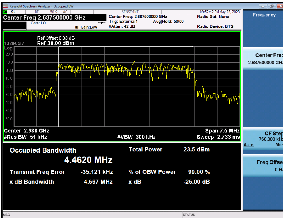
LTE Band 41 / 5MHz / QPSK - RB Size 25
