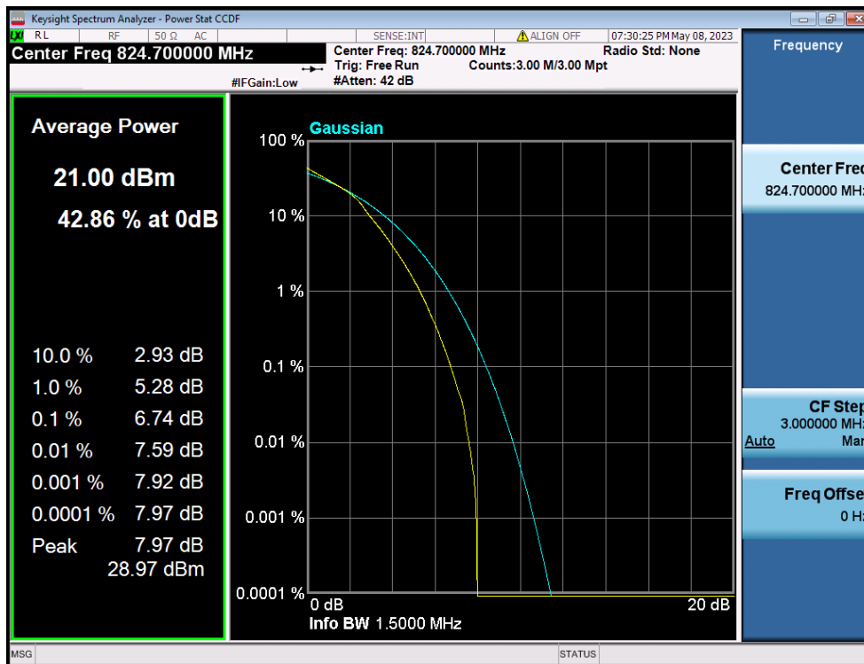
LTE Band 26(5) / 1.4MHz / 16QAM - RB Size 6
