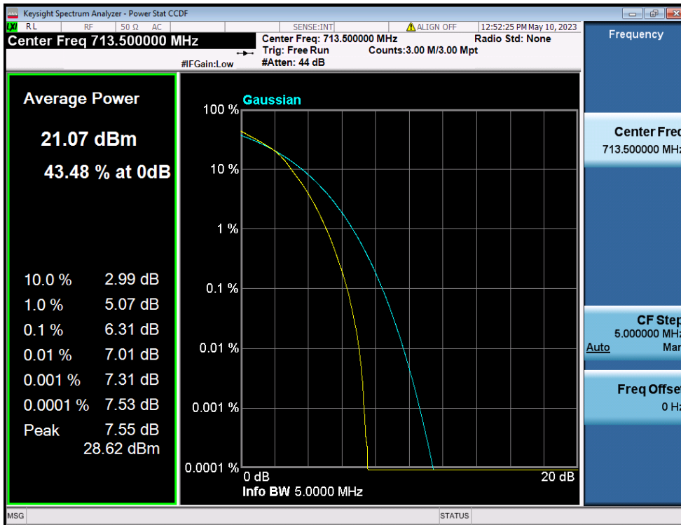
LTE Band 12(17) / 5MHz / 16QAM - RB Size 25
