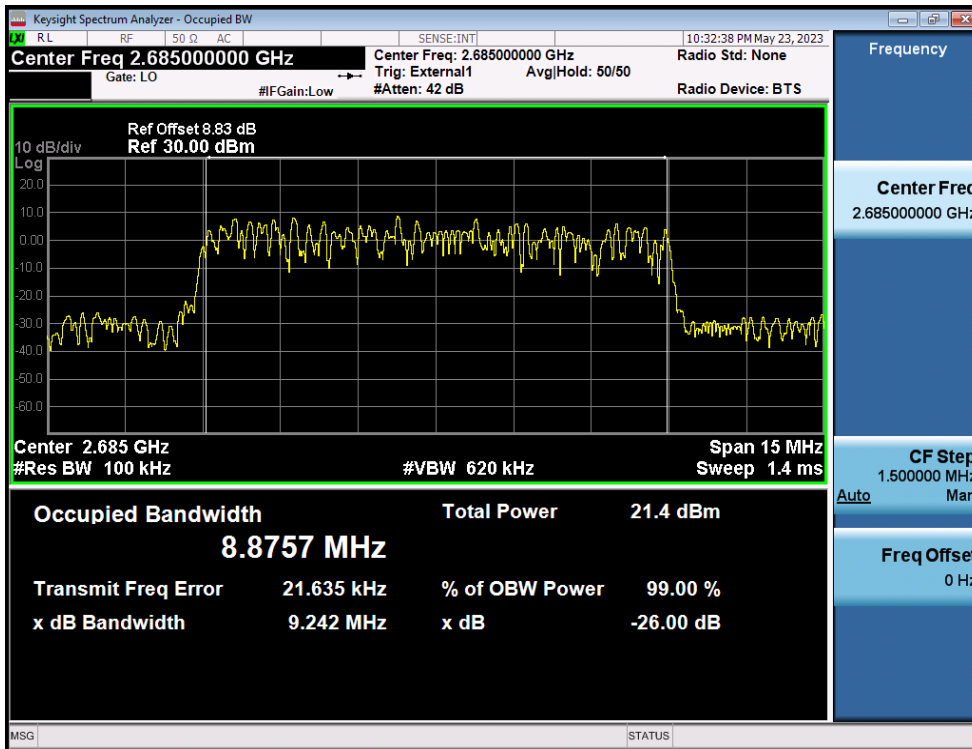
LTE Band 41 / 10MHz / 64QAM - RB Size 50
