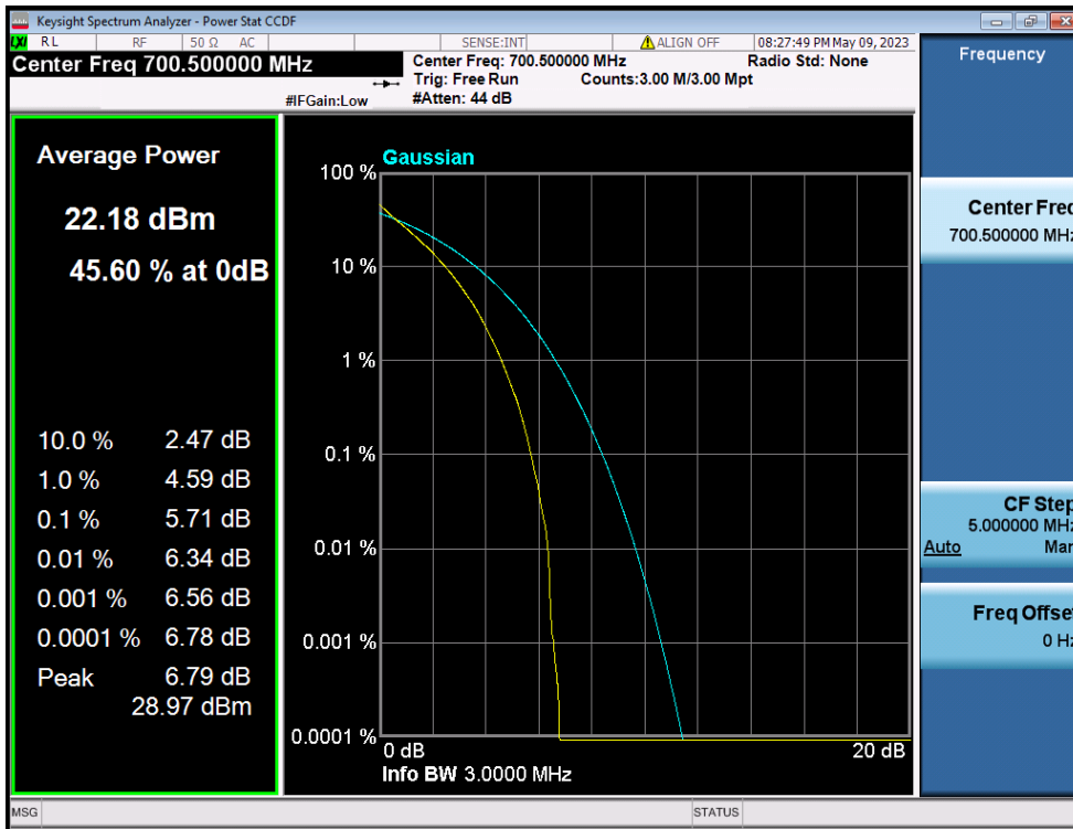
LTE Band 12 / 3MHz / QPSK - RB Size 15
