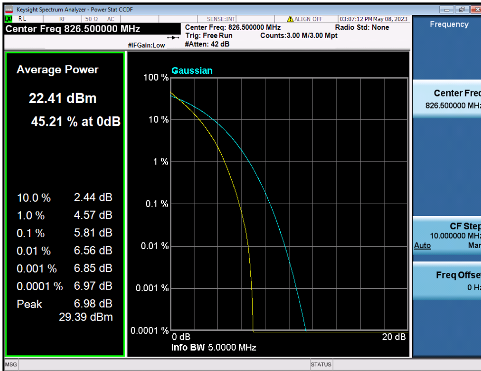
LTE Band 26(5) / 5MHz / QPSK - RB Size 25
