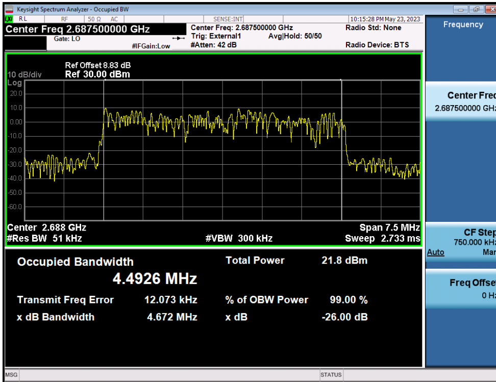
LTE Band 41 / 5MHz / 16QAM - RB Size 25
