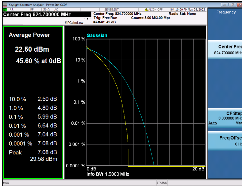
LTE Band 26(5) / 1.4MHz / QPSK - RB Size 6
