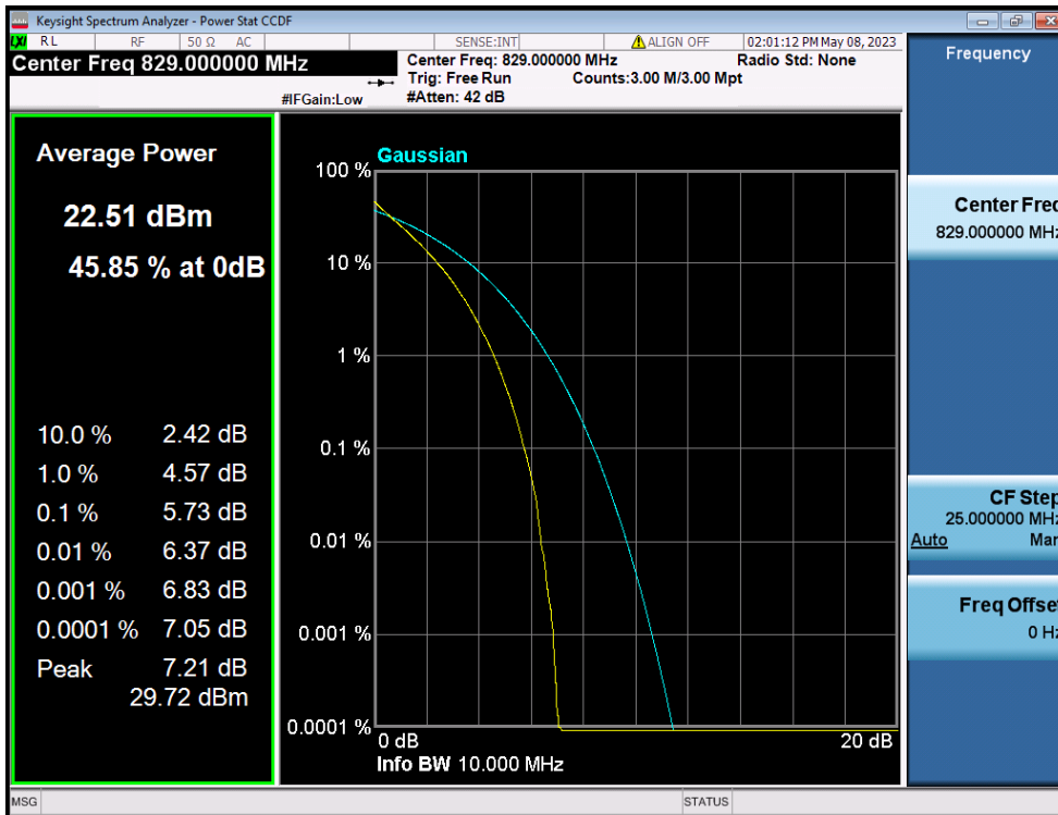
LTE Band 26(5) / 10MHz / QPSK - RB Size 50
