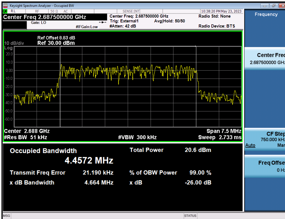
LTE Band 41 / 5MHz / 64QAM - RB Size 25
