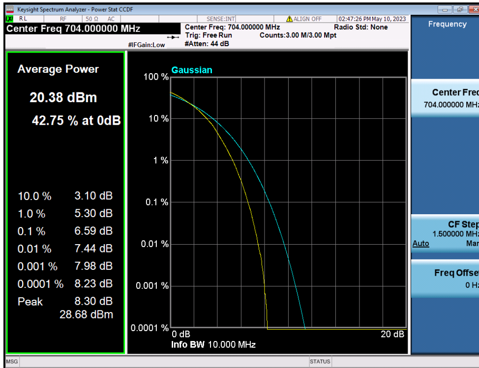
LTE Band 12(17) / 10MHz / 64QAM - RB Size 50
