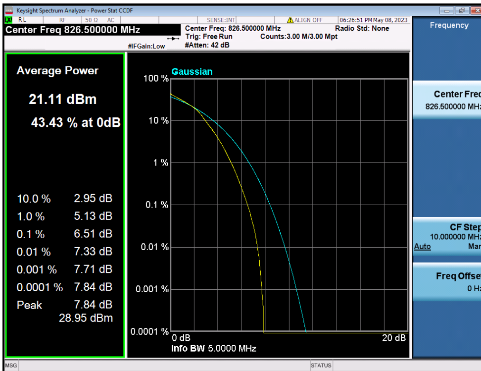
LTE Band 26(5) / 5MHz / 16QAM - RB Size 25
