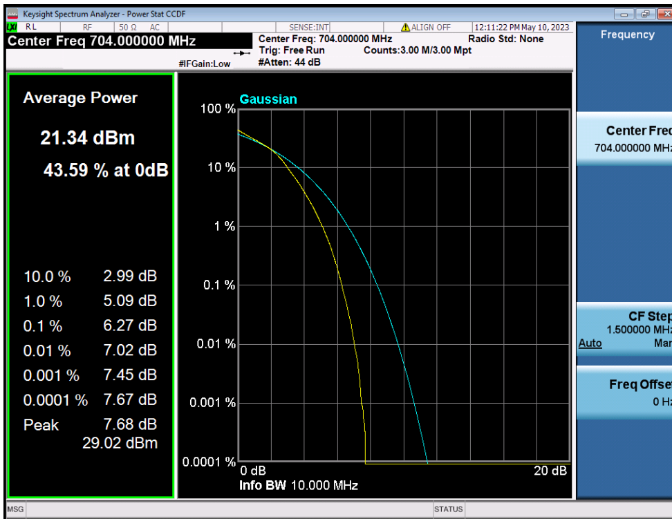
LTE Band 12(17) / 10MHz / 16QAM - RB Size 50
