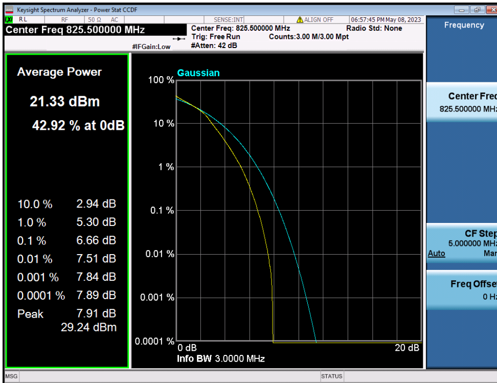
LTE Band 26(5) / 3MHz / 16QAM - RB Size 15
