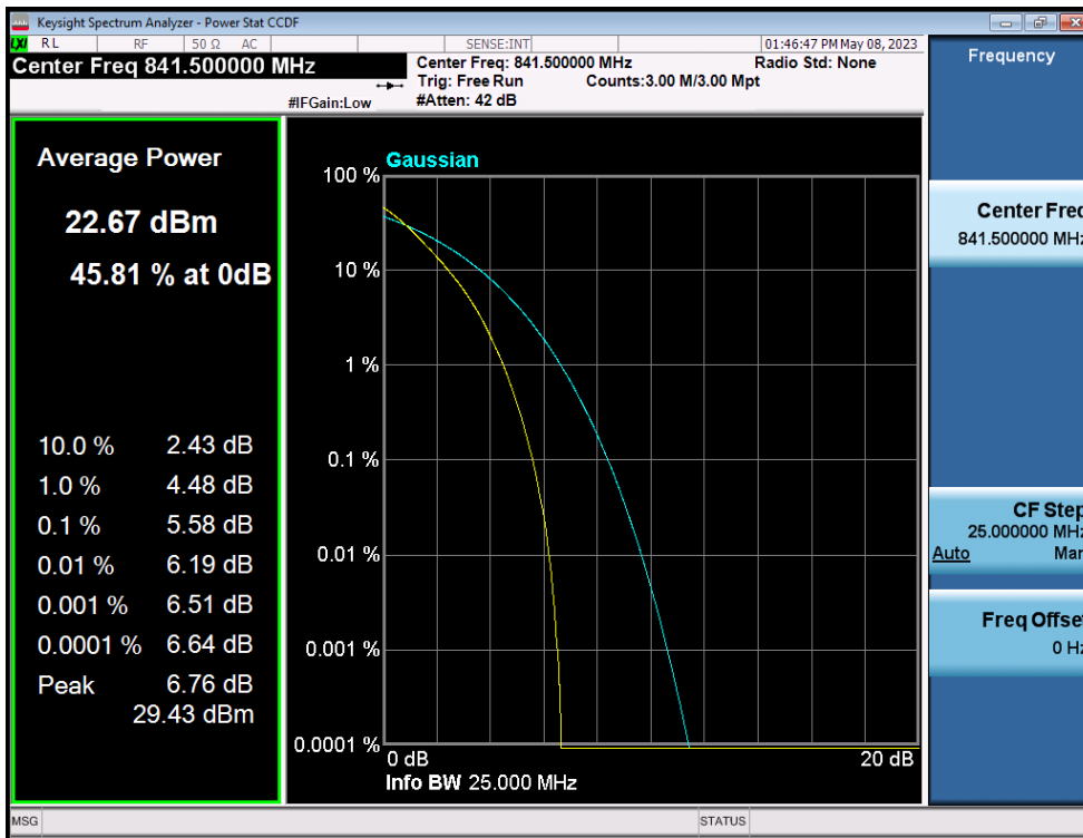
LTE Band 26 / 15MHz / QPSK - RB Size 75
