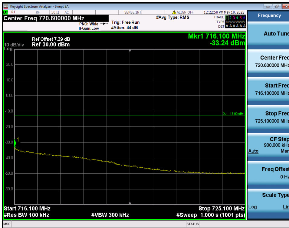
LTE Band 12(17) / 10MHz / 16QAM - RB Size/Offset (25/25)
