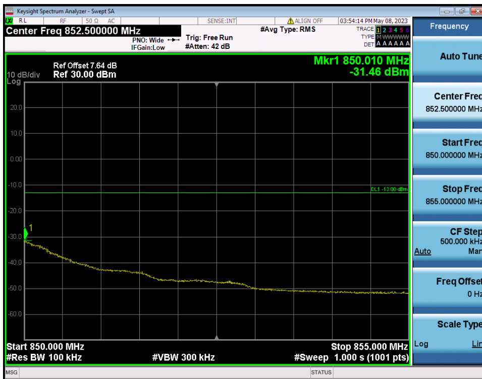
LTE Band 26(5) / 3MHz / QPSK - RB Size/Offset (8/7)
