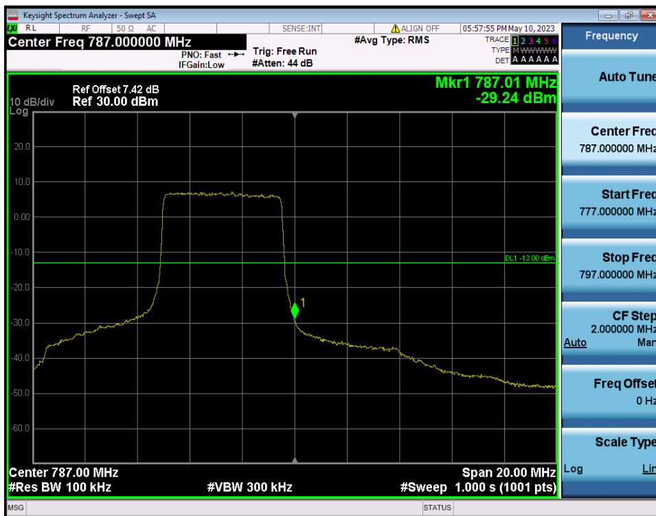
LTE Band 13 / 10MHz / QPSK - RB Size/Offset (25/25)
