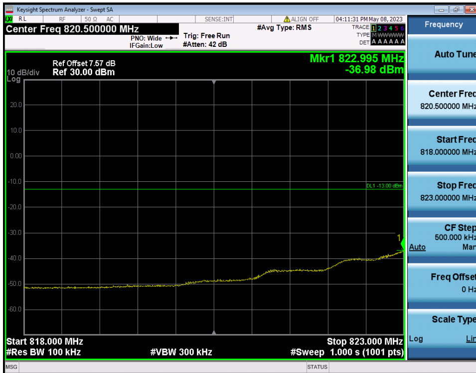
LTE Band 26(5) / 1.4MHz / QPSK - RB Size/Offset (6/0)
