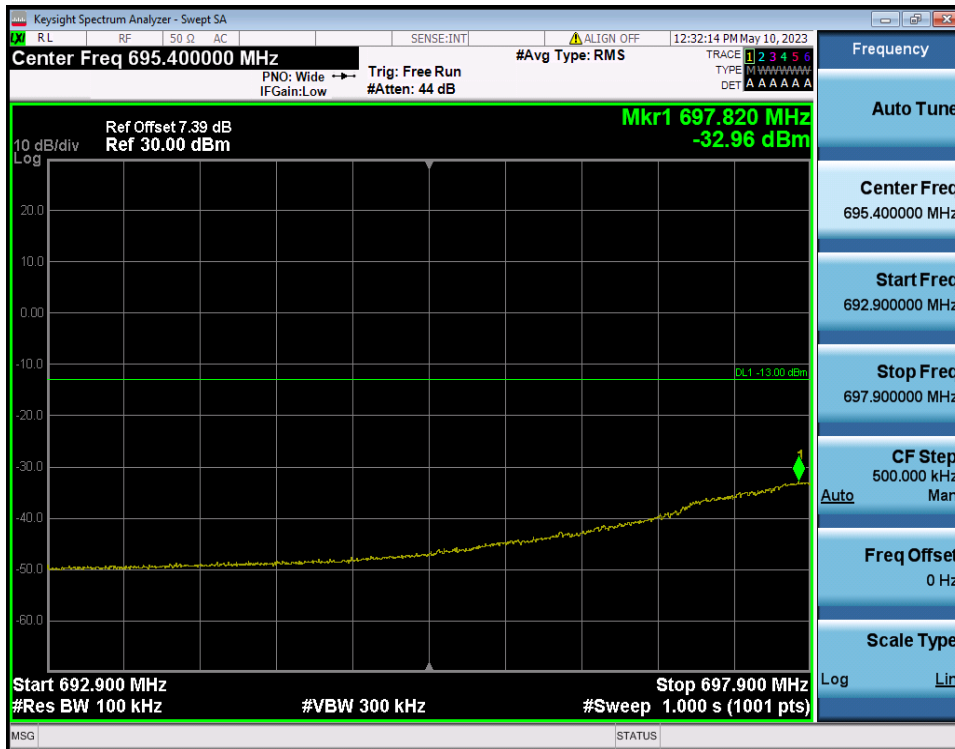
LTE Band 12(17) / 5MHz / 16QAM - RB Size/Offset (12/0)
