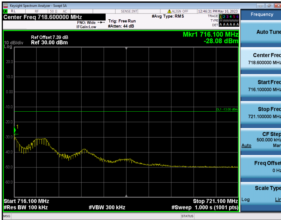
LTE Band 12(17) / 5MHz / 16QAM - RB Size/Offset (1/24)
