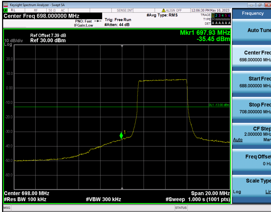
LTE Band 12(17) / 10MHz / 16QAM - RB Size/Offset (25/0)
