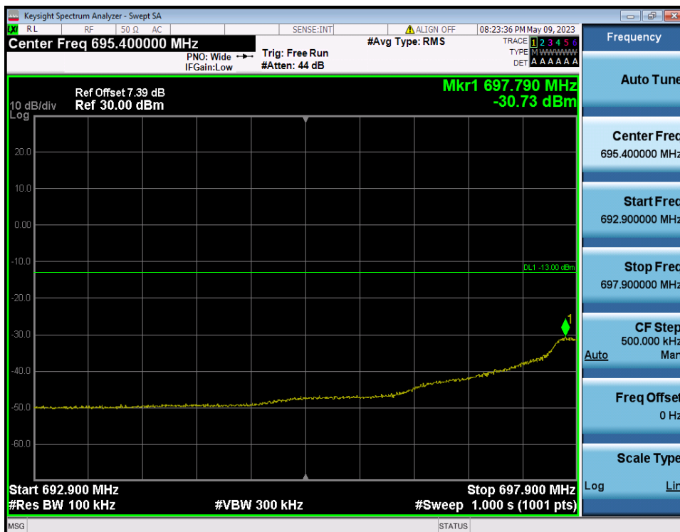
LTE Band 12 / 3MHz / QPSK - RB Size/Offset (8/0)
