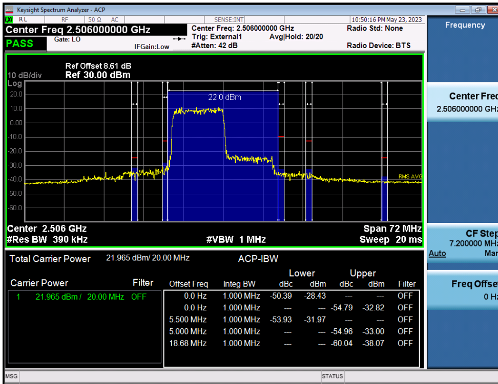
LTE Band 41(38) / 20MHz / QPSK - RB Size/Offset (50/0)
