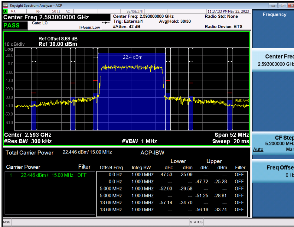
LTE Band 41(38) / 15MHz / QPSK - RB Size/Offset (75/0)
