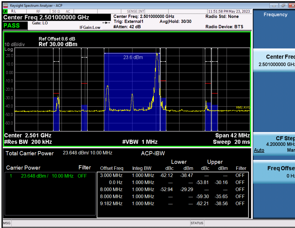
LTE Band 41(38) / 10MHz / QPSK - RB Size/Offset (1/49)
