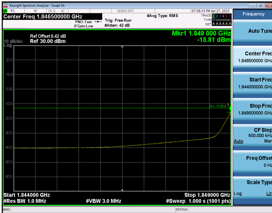
LTE Band 25(2) / 1.4MHz / 16QAM - RB Size/Offset (3/2)
