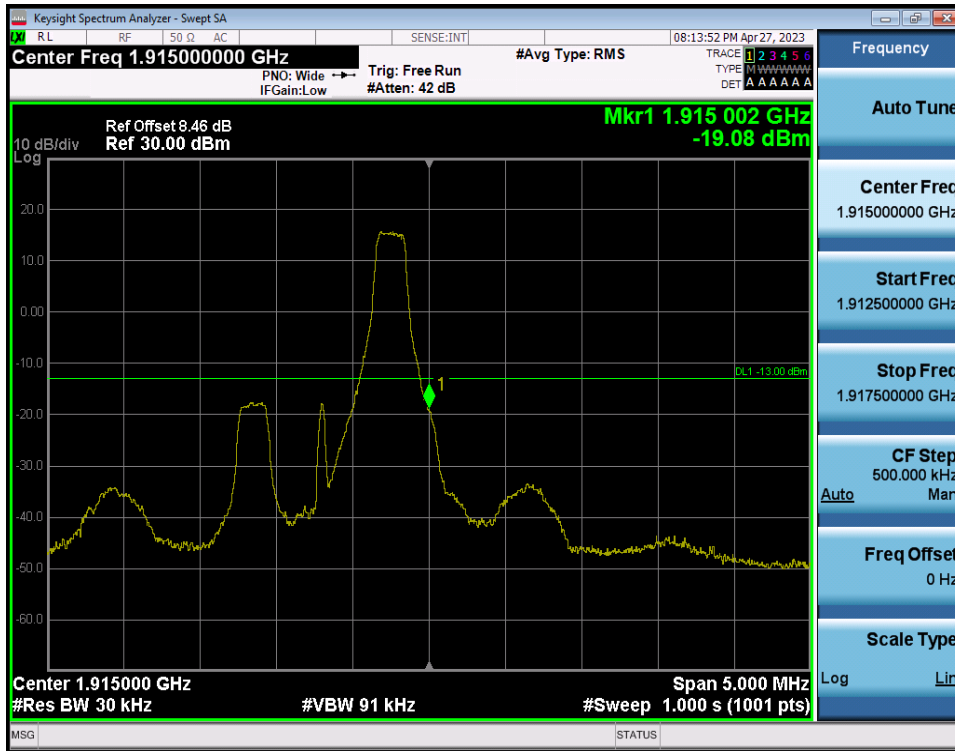
LTE Band 25(2) / 1.4MHz / 16QAM - RB Size/Offset (1/5)
