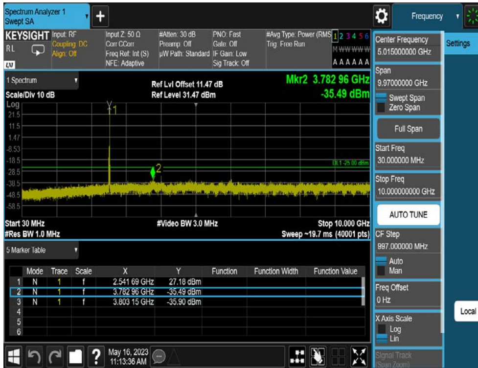
LTE Band 7 / 15MHz / 64QAM - RB Size/Offset (1/74) - Mid Channel
