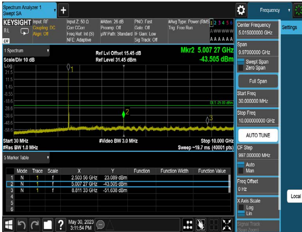
LTE Band 41(38) / 15MHz / QPSK - RB Size/Offset (1/36) - Low Channel
