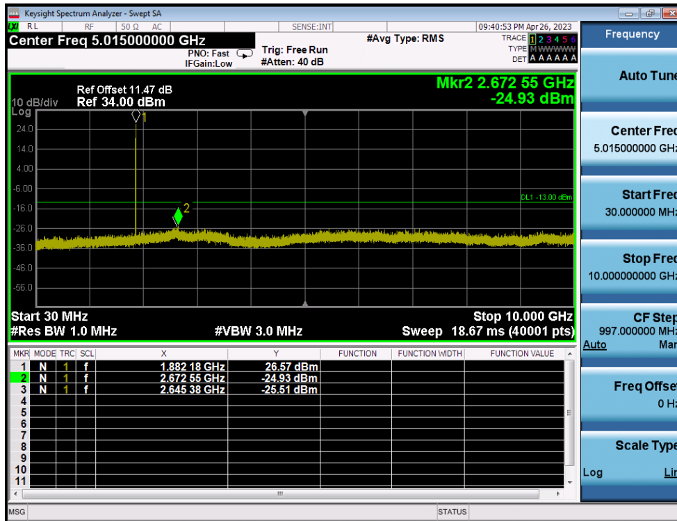
LTE Band 25(2) / 5MHz / QPSK - RB Size/Offset (12/6) - Mid Channel
