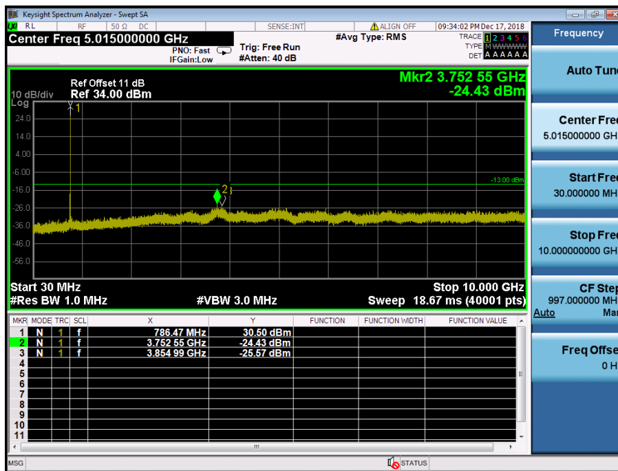
LTE Band 13 / 10MHz / 16QAM - RB Size/Offset (1/49) – Low Channel
