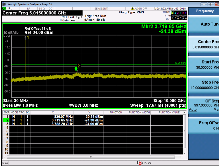
LTE Band 5 / 1.4MHz / 16QAM - RB Size/Offset (1/0) – Mid Channel
