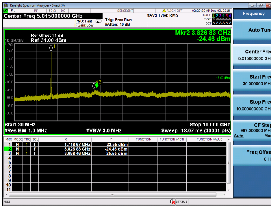
LTE Band 4 / 20MHz / QPSK - RB Size/Offset (50/25) –Low Channel
