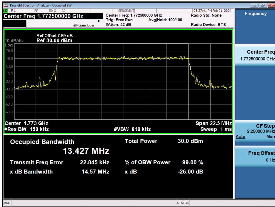
LTE Band 66 / 15MHz / 16QAM - RB Size 75
