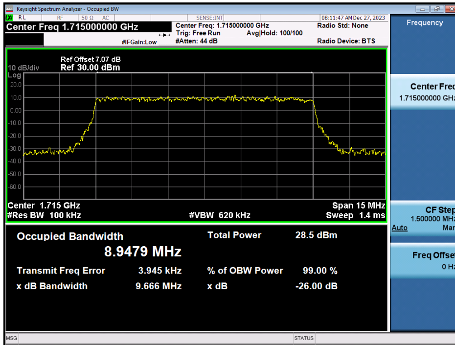
LTE Band 66 / 10MHz / 64QAM - RB Size 50
