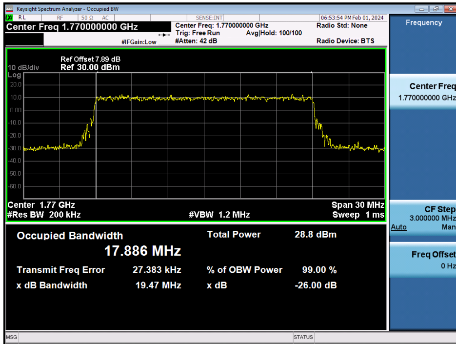
LTE Band 66 / 20MHz / 64QAM - RB Size 100
