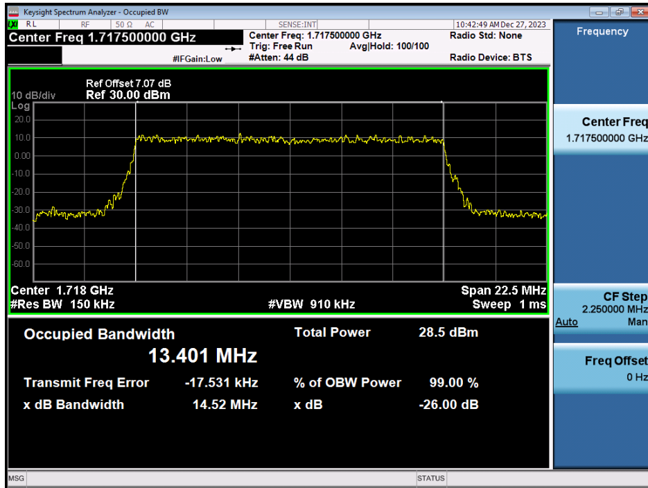
LTE Band 66 / 15MHz / 64QAM - RB Size 75
