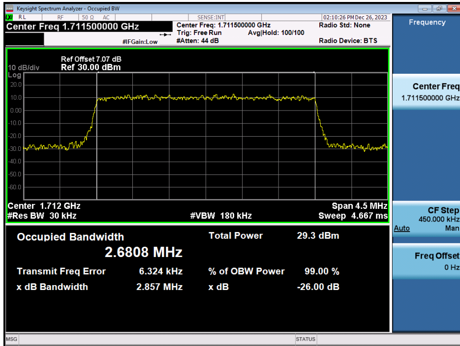
LTE Band 66 / 3MHz / 16QAM - RB Size 15
