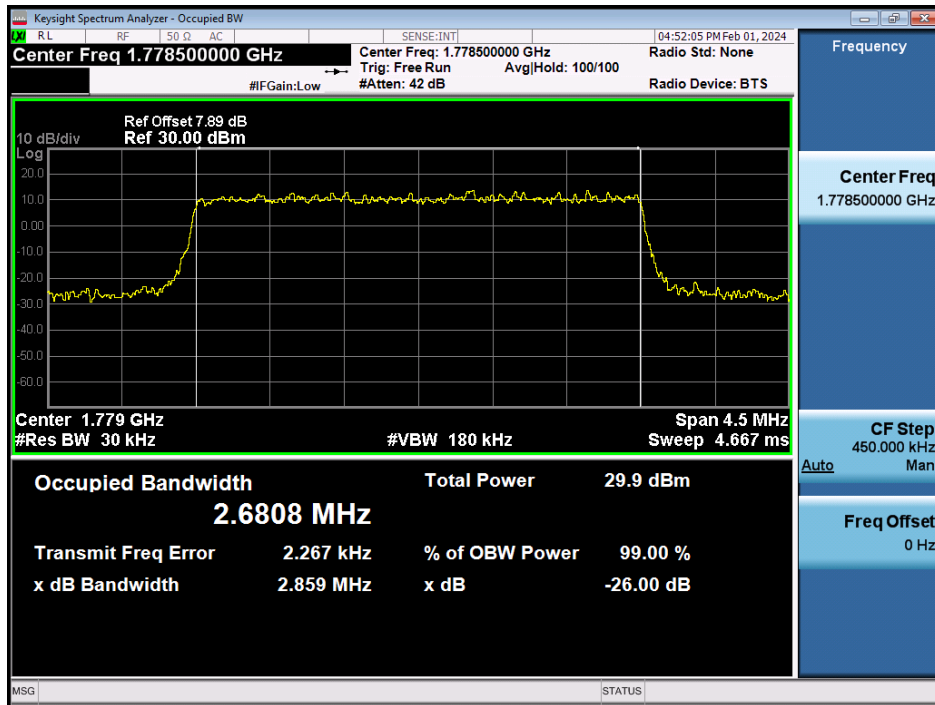
LTE Band 66 / 3MHz / QPSK - RB Size 15
