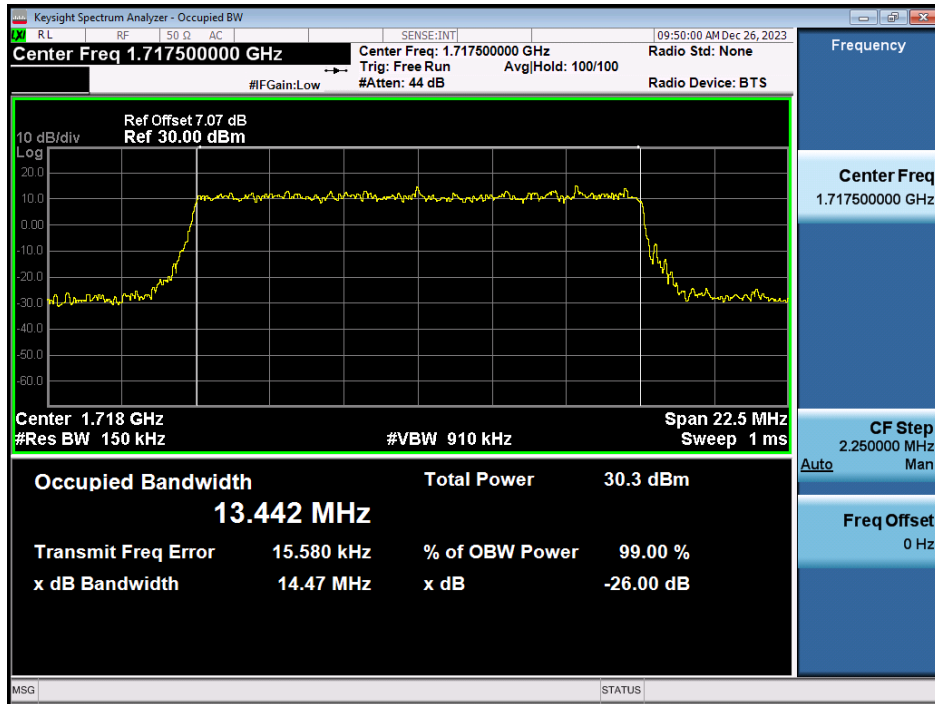
LTE Band 66 / 15MHz / QPSK - RB Size 75
