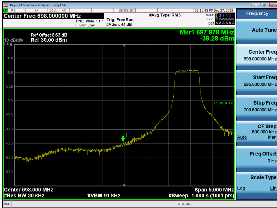
LTE Band 12 / 1.4MHz / 16QAM - RB Size/Offset (3/0)
