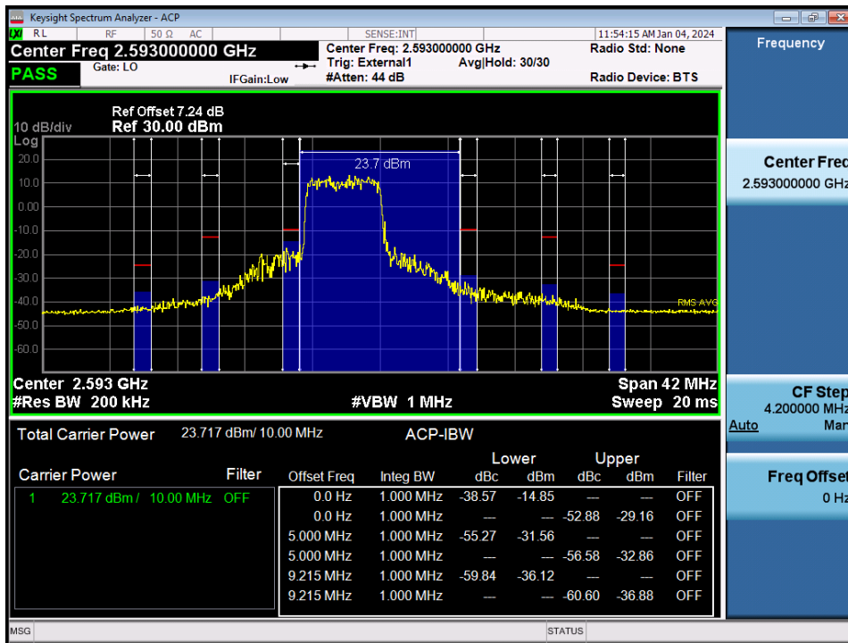
LTE Band 41 / 10MHz / QPSK - RB Size/Offset (25/0)
