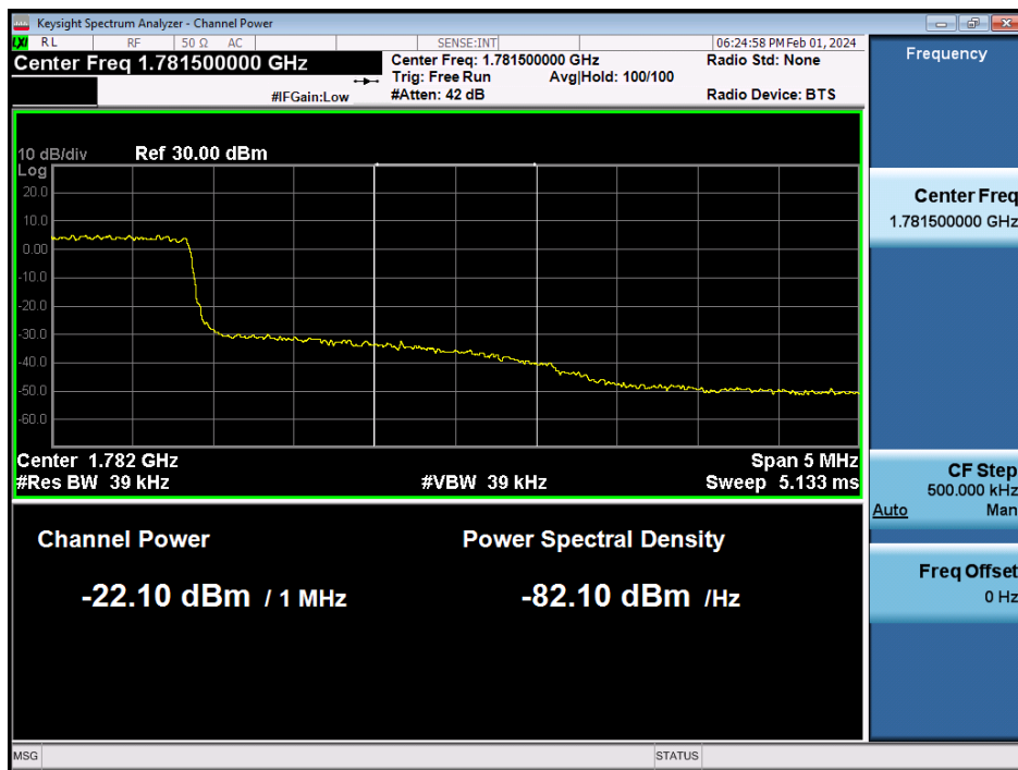
LTE Band 66 / 3MHz / 16QAM - RB Size/Offset (15/0)
