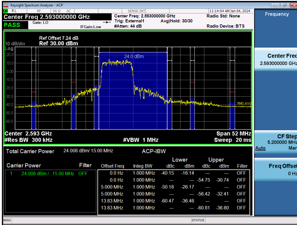
LTE Band 41 / 15MHz / QPSK - RB Size/Offset (36/0)
