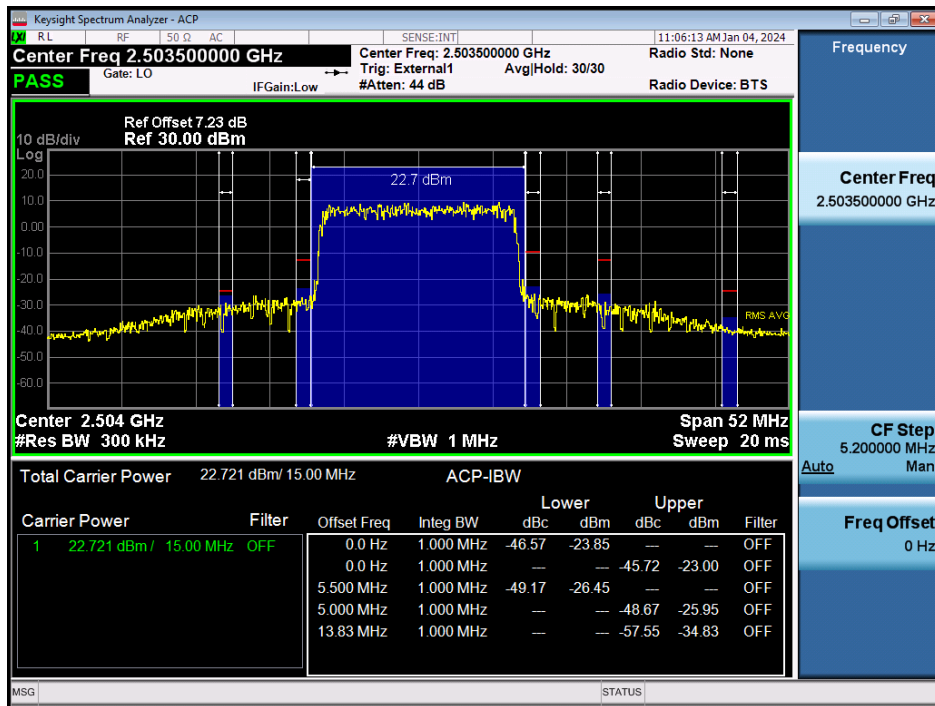
LTE Band 41 / 15MHz / QPSK - RB Size/Offset (75/0)
