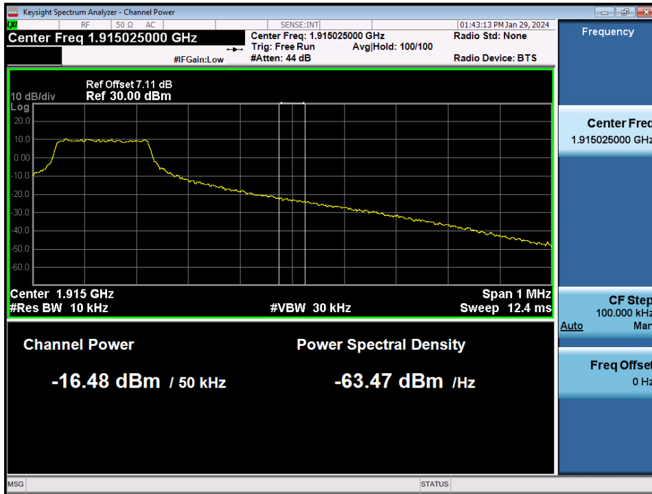
LTE Band 25 / 5MHz / 64QAM - RB Size/Offset (1/24)
