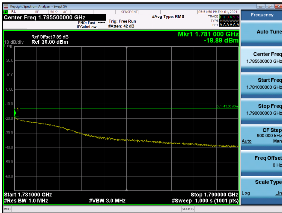
LTE Band 66 / 10MHz / 16QAM - RB Size/Offset (25/25)
