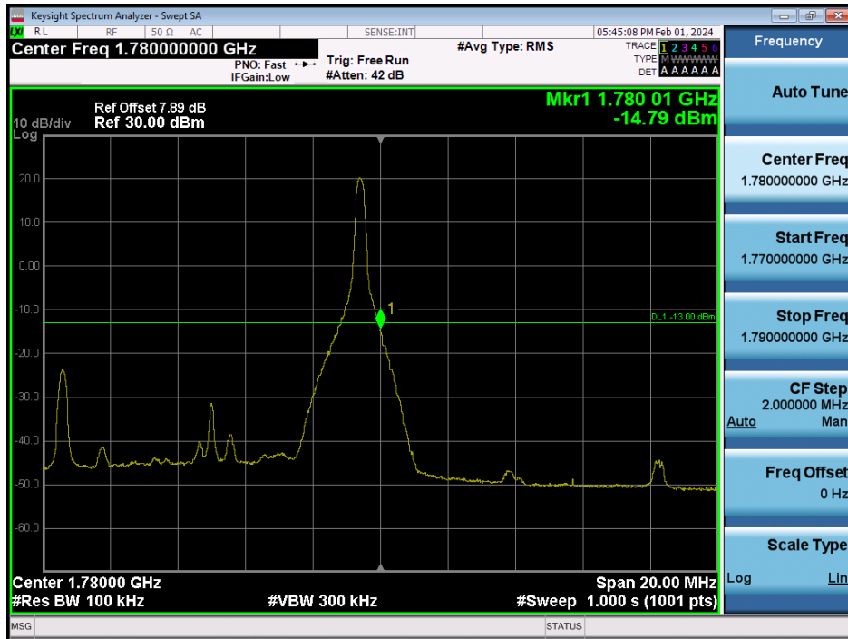
LTE Band 66 / 10MHz / 16QAM - RB Size/Offset (1/49)
