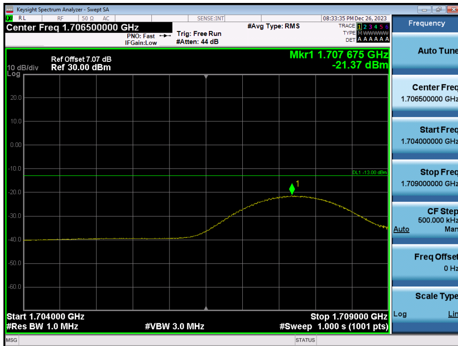
LTE Band 66 / 3MHz / 64QAM - RB Size/Offset (1/14)
