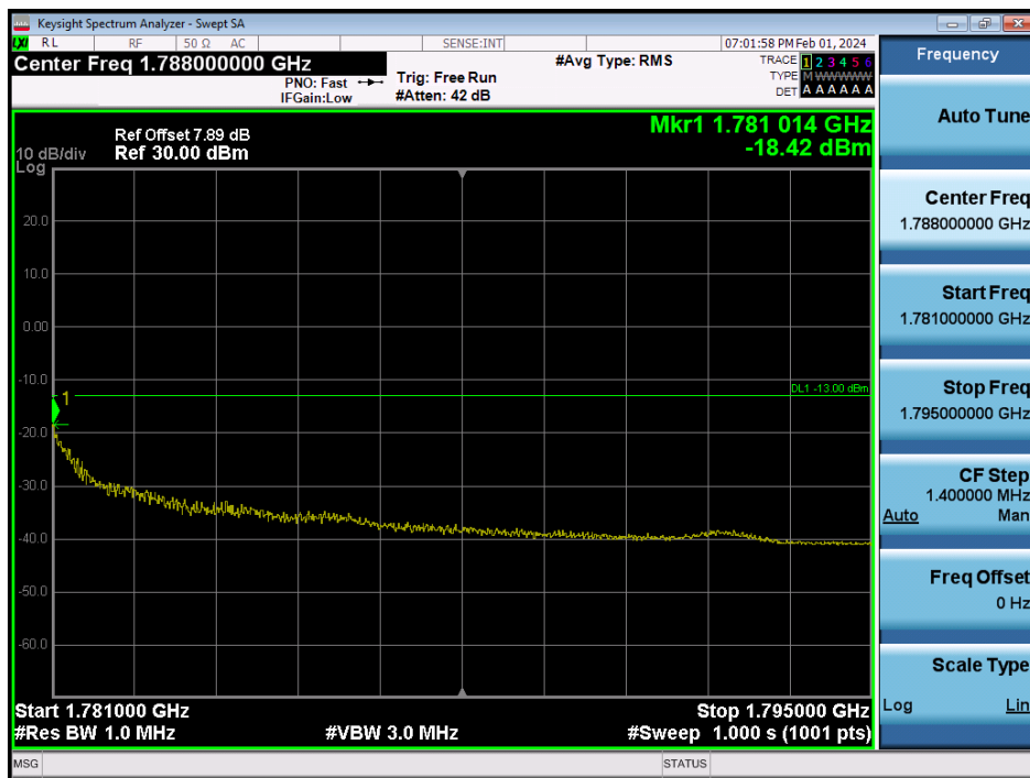
LTE Band 66 / 15MHz / 64QAM - RB Size/Offset (1/74)
