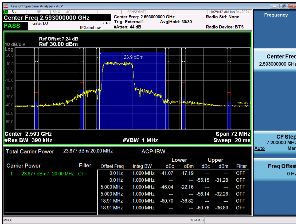
LTE Band 41 / 20MHz / QPSK - RB Size/Offset (50/0)
