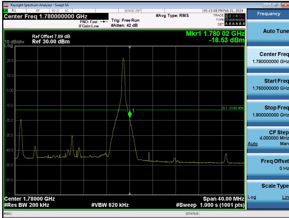
LTE Band 66 / 20MHz / 16QAM - RB Size/Offset (1/99)
