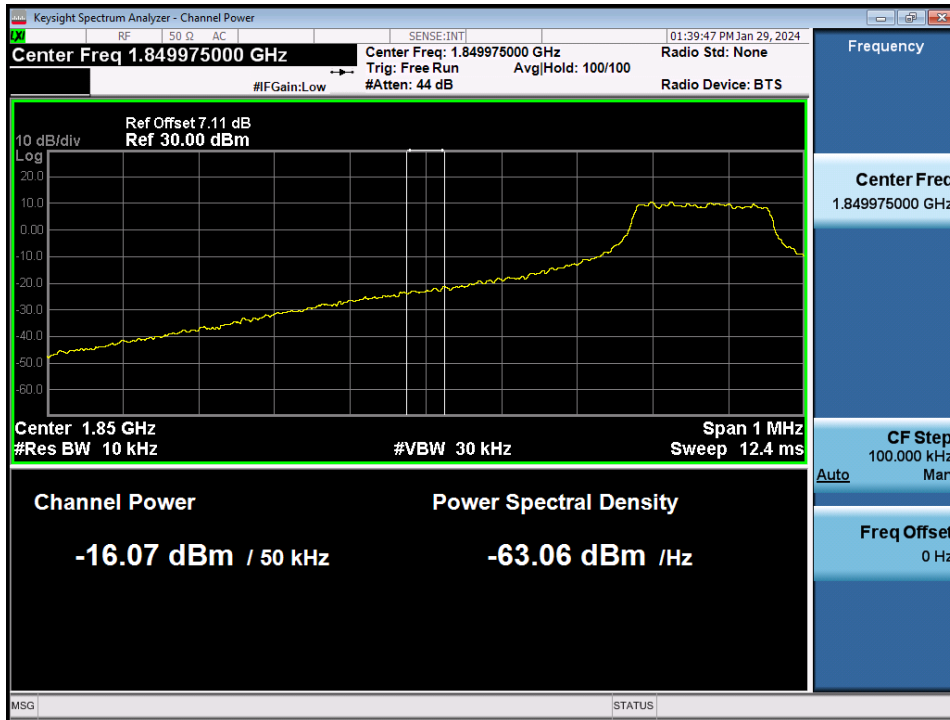
LTE Band 25 / 5MHz / 16QAM - RB Size/Offset (1/0)
