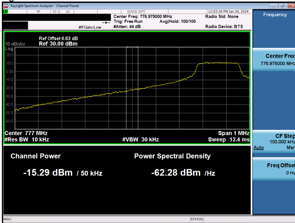
LTE Band 13 / 5MHz / QPSK - RB Size/Offset (1/0)
