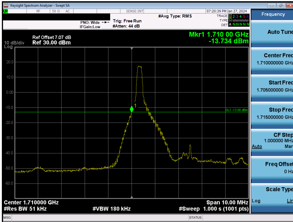
LTE Band 66 / 5MHz / 16QAM - RB Size/Offset (1/0)
