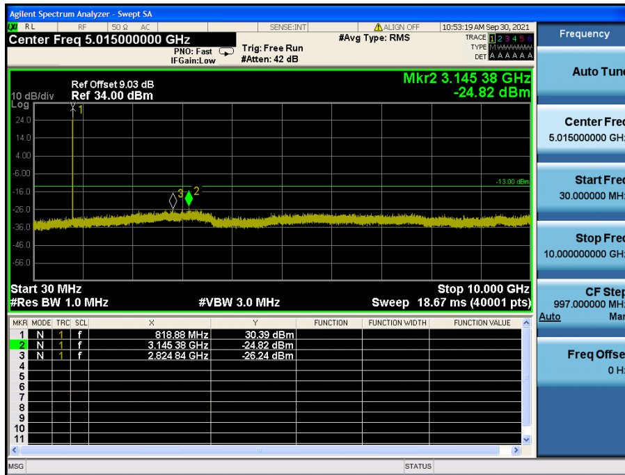
LTE Band 26 / 1.4MHz / 16QAM - RB Size/Offset (3/0) – Mid Channel
