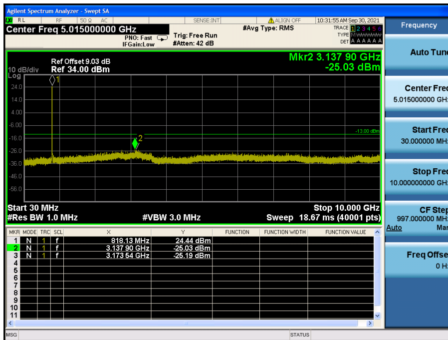
LTE Band 26 / 10MHz / QPSK - RB Size/Offset (25/12) - Low Channel
