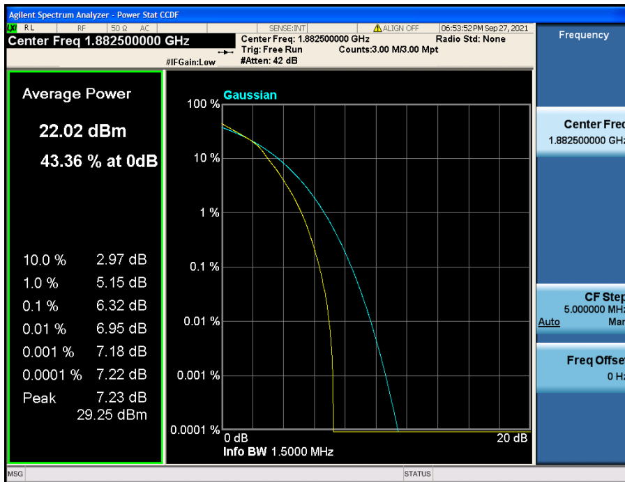
LTE Band 25(2) / 1.4 MHz / 16QAM - RB Size 6
