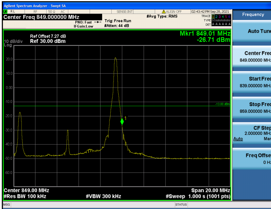
LTE Band 26(5) / 10 MHz / 16QAM - RB Size/Offset (1/49)
