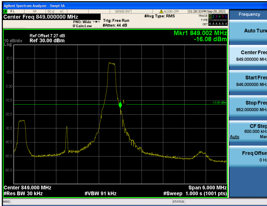
LTE Band 26(5) / 3 MHz / 16QAM - RB Size/Offset (1/14)
