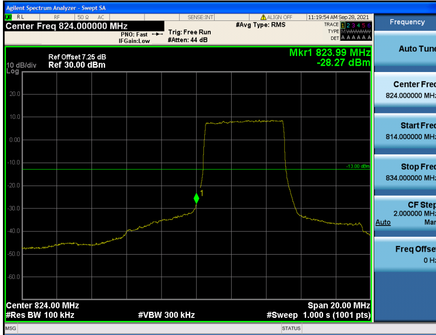
LTE Band 26(5) / 10 MHz / QPSK - RB Size/Offset (25/0)
