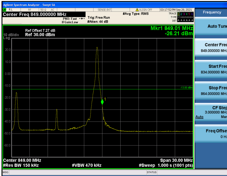
LTE Band 26 / 15 MHz / 16QAM - RB Size/Offset (1/74)
