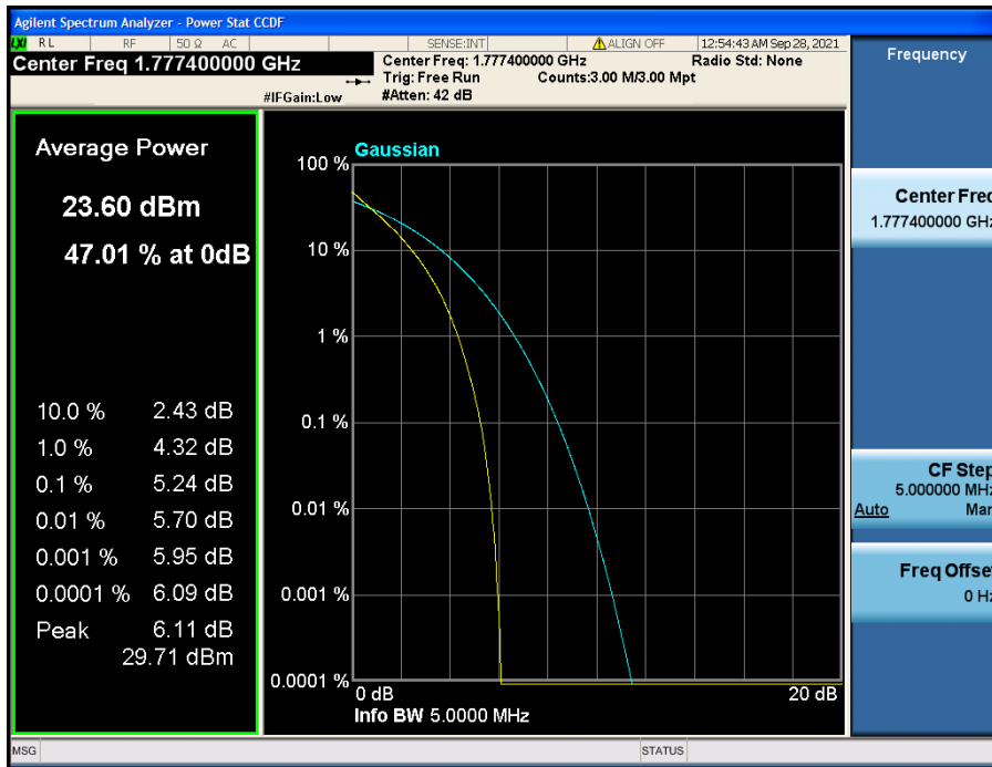
LTE Band 66(4) / 5 MHz / QPSK - RB Size 25
