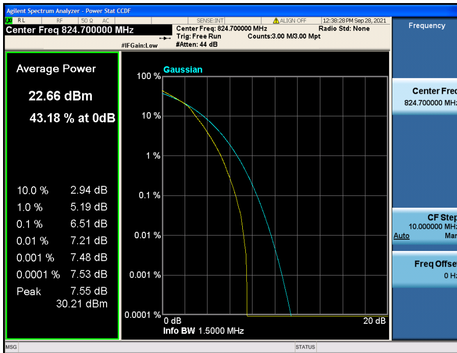
LTE Band 26(5) / 1.4 MHz / 16QAM - RB Size 6
