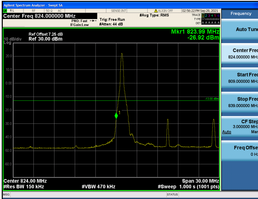
LTE Band 26 / 15 MHz / 16QAM - RB Size/Offset (1/0)
