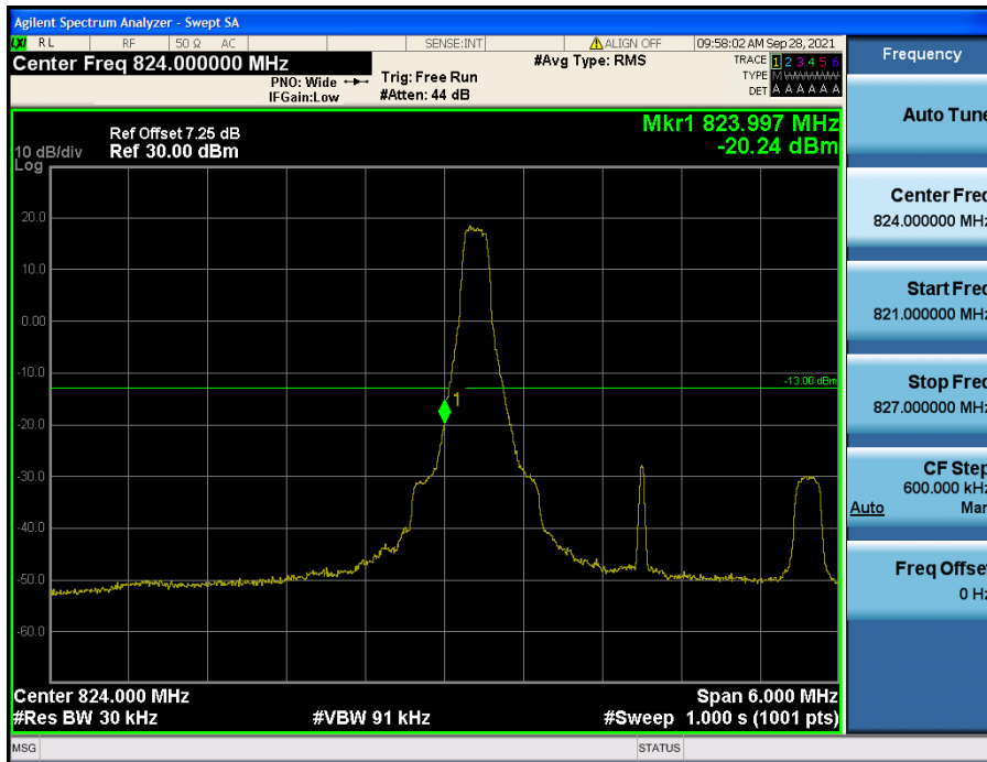
LTE Band 26(5) / 3 MHz / QPSK - RB Size/Offset (1/0)
