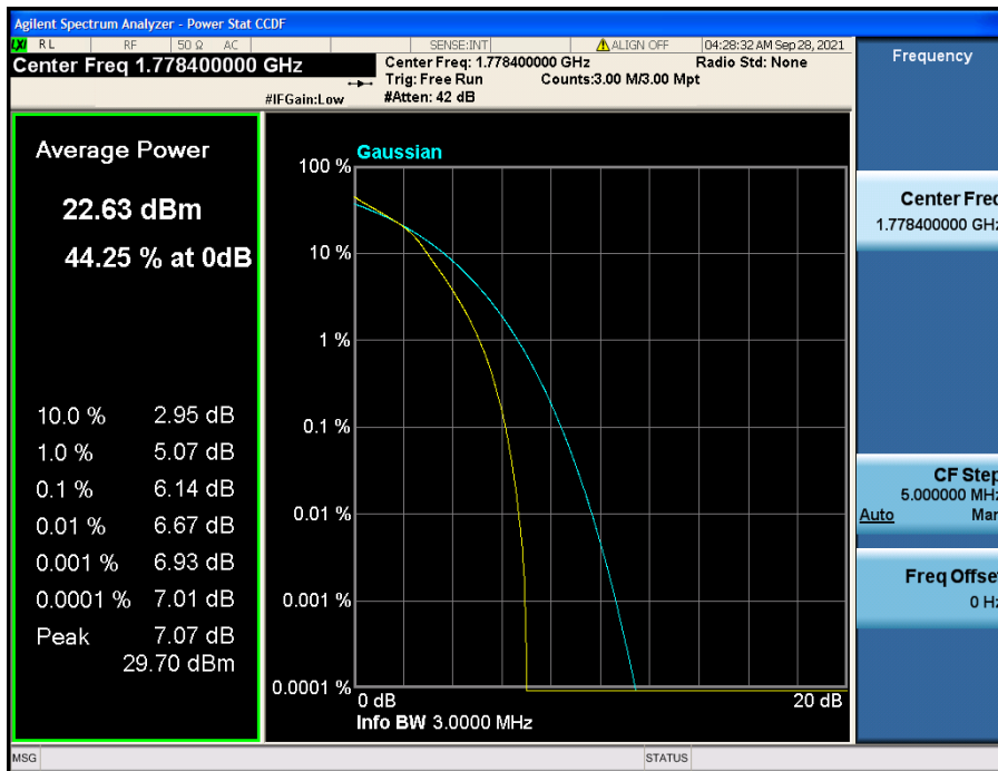
LTE Band 66(4) / 3 MHz / 16QAM - RB Size 15
