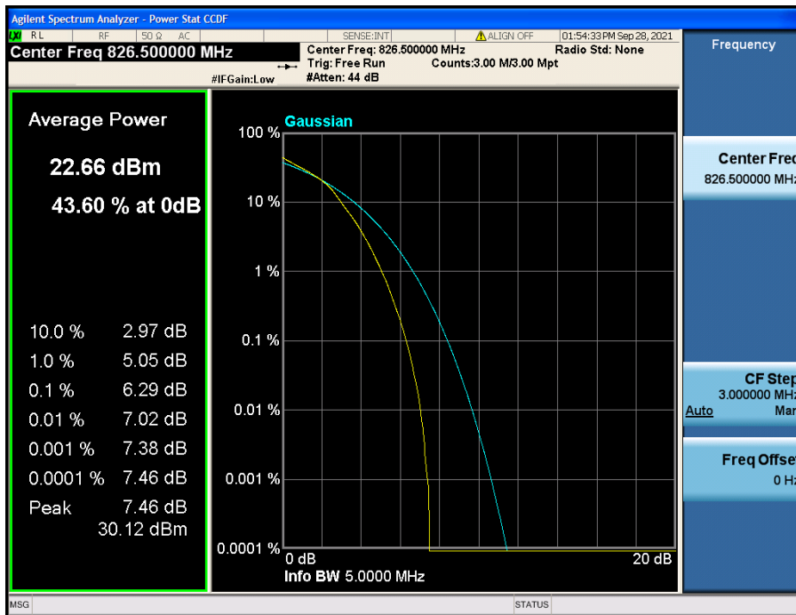
LTE Band 26(5) / 5 MHz / 16QAM - RB Size 25
