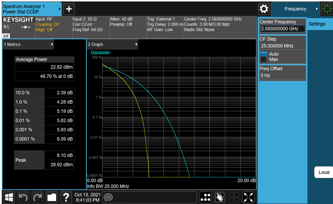
LTE Band 41(38) / 15 MHz / QPSK - RB Size 75
