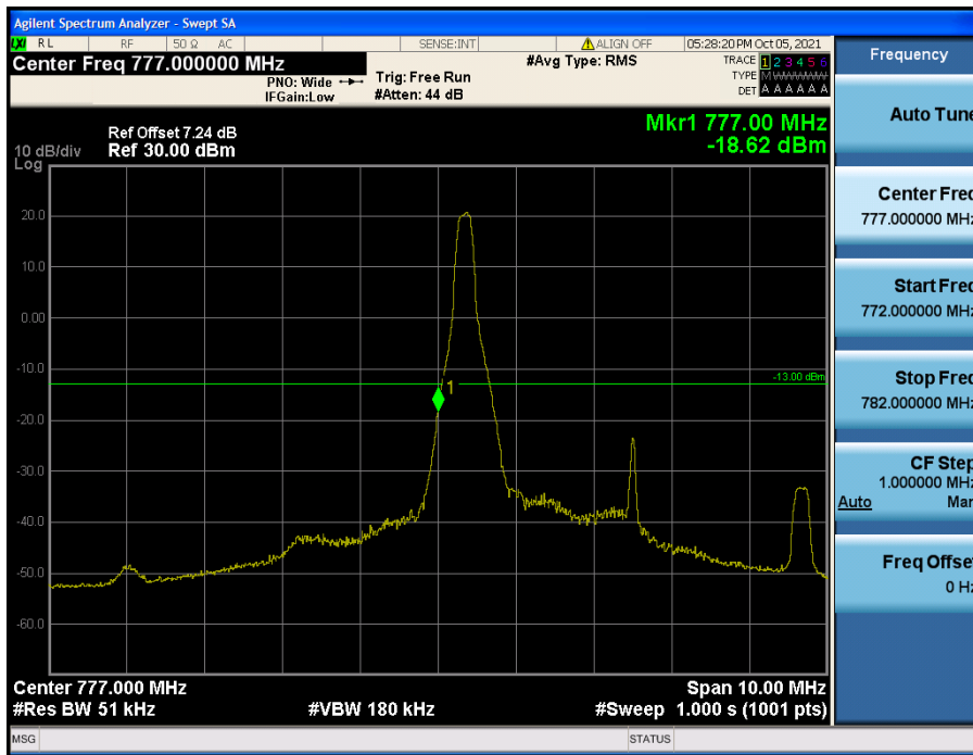
LTE Band 13 / 5 MHz / QPSK - RB Size/Offset (1/0)
