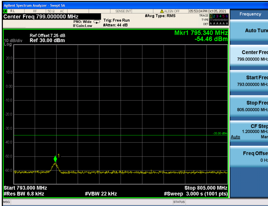
LTE Band 13 / 5 MHz / QPSK - RB Size/Offset (1/24)
