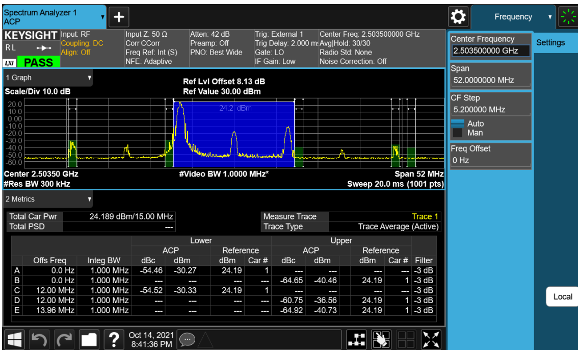
LTE Band 41(38) / 15 MHz / QPSK - RB Size/Offset (1/0)
