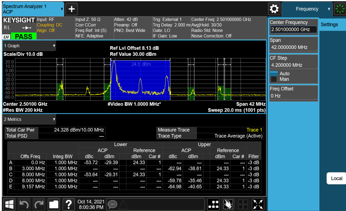
LTE Band 41(38) / 10 MHz / QPSK - RB Size/Offset (1/0)
