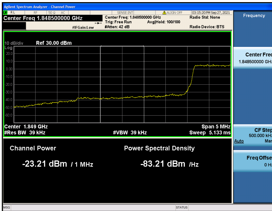
LTE Band 25(2) / 3 MHz / QPSK - RB Size/Offset (15/0)
