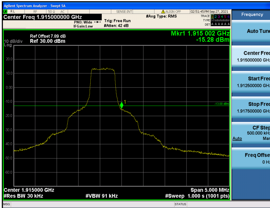
LTE Band 25(2) / 1.4 MHz / QPSK - RB Size/Offset (3/3)
