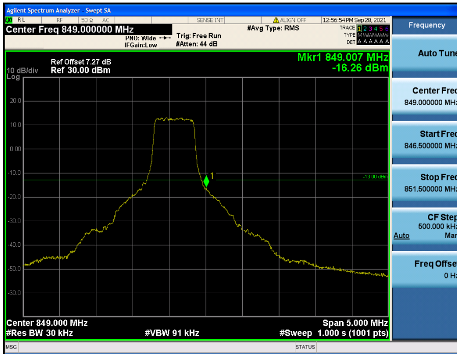
LTE Band 26(5) / 1.4 MHz / 16QAM - RB Size/Offset (3/3)
