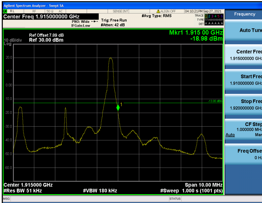
LTE Band 25(2) / 5 MHz / QPSK - RB Size/Offset (1/24)
