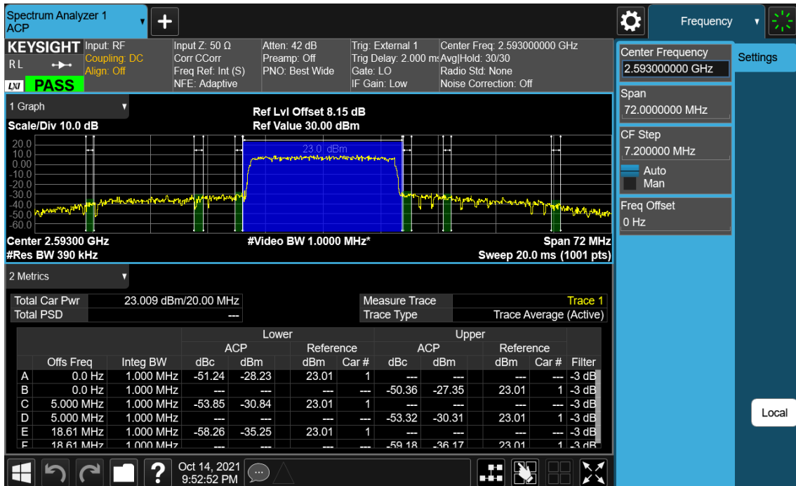
LTE Band 41(38) / 20 MHz / QPSK - RB Size/Offset (100/0)
