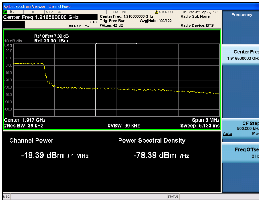
LTE Band 25(2) / 5 MHz / QPSK - RB Size/Offset (25/0)
