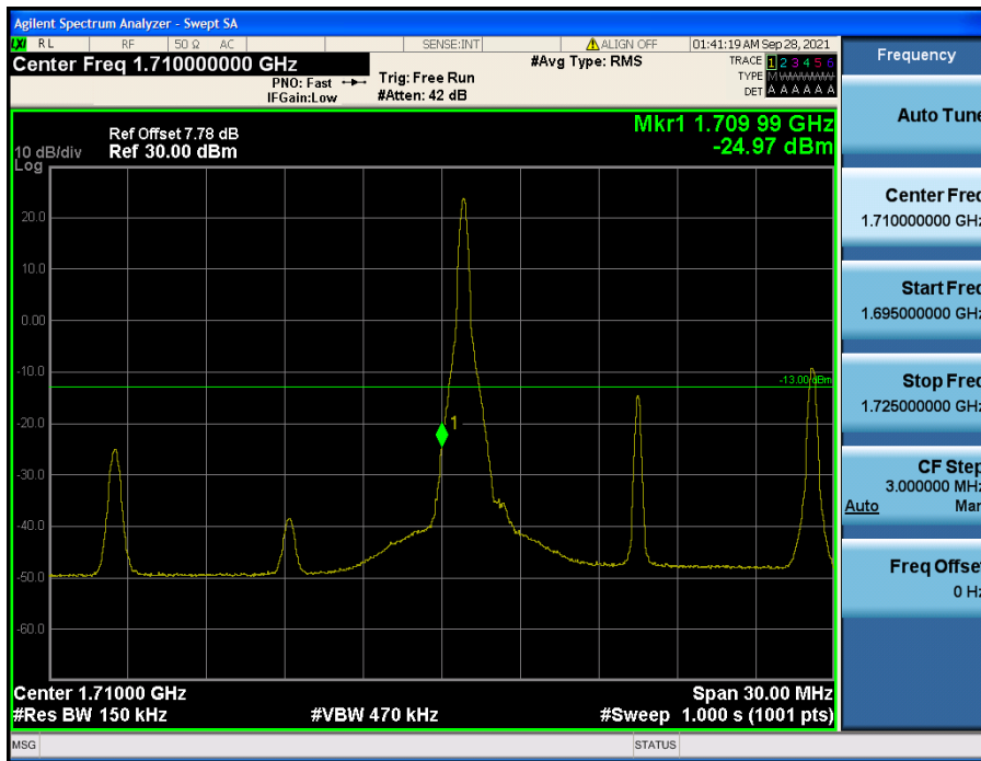
LTE Band 66(4) / 15 MHz / QPSK - RB Size/Offset (1/0)
