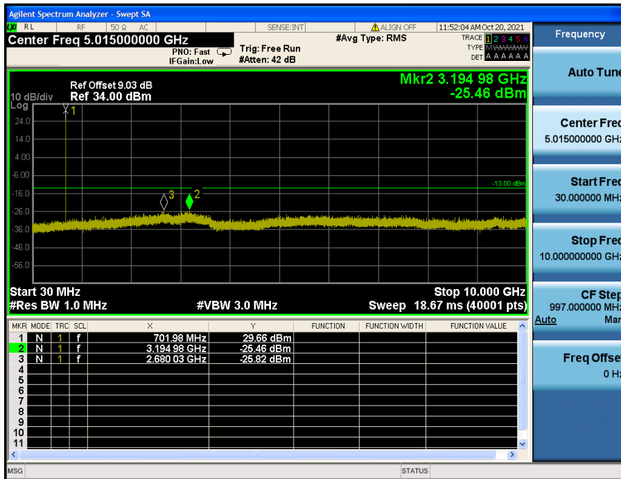
LTE Band 12 / 5 MHz / QPSK - RB Size/Offset (1/12) – Low Channel
