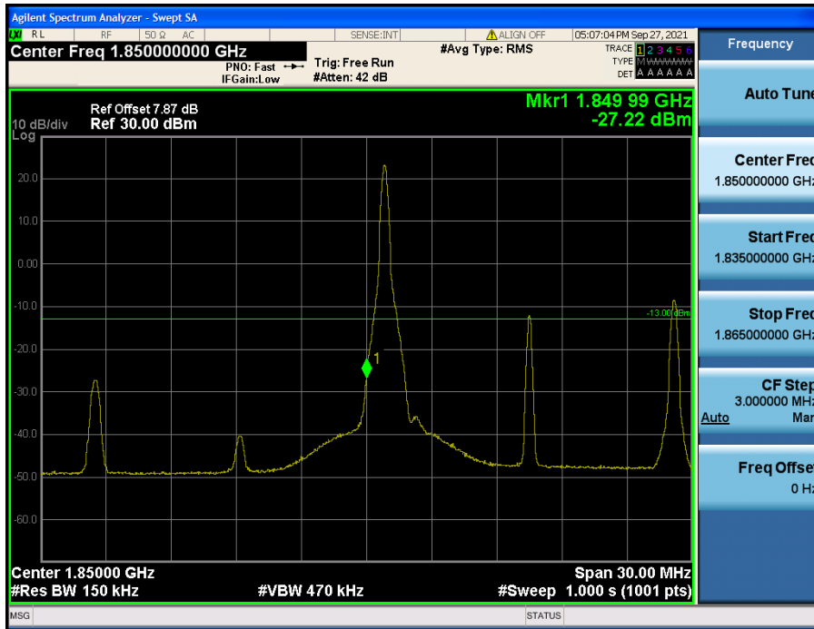
LTE Band 25(2) / 15 MHz / QPSK - RB Size/Offset (1/0)
