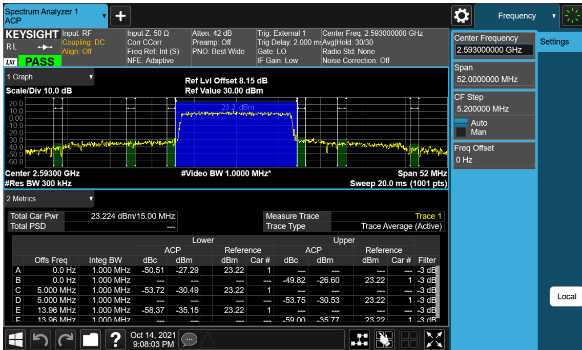
LTE Band 41(38) / 15 MHz / QPSK - RB Size/Offset (75/0)
