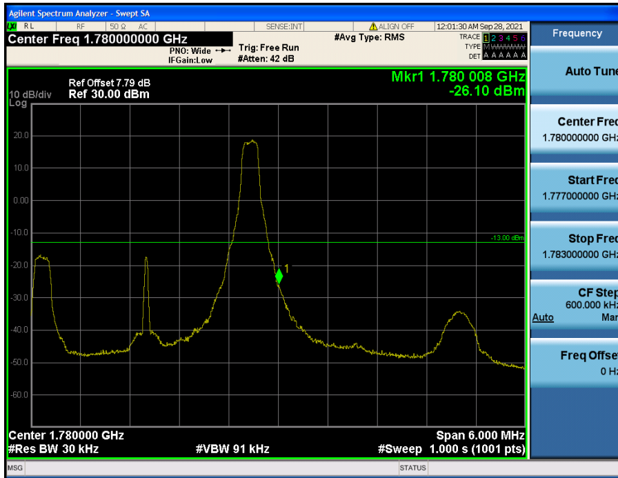
LTE Band 66(4) / 3 MHz / QPSK - RB Size/Offset (1/14)
