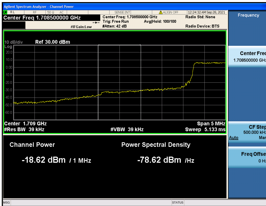
LTE Band 66(4) / 5 MHz / QPSK Offset/Size (12/0)
