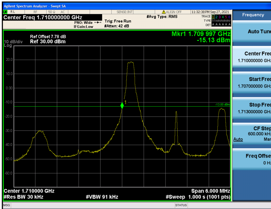
LTE Band 66(4) / 3 MHz / QPSK - RB Size/Offset (1/0)
