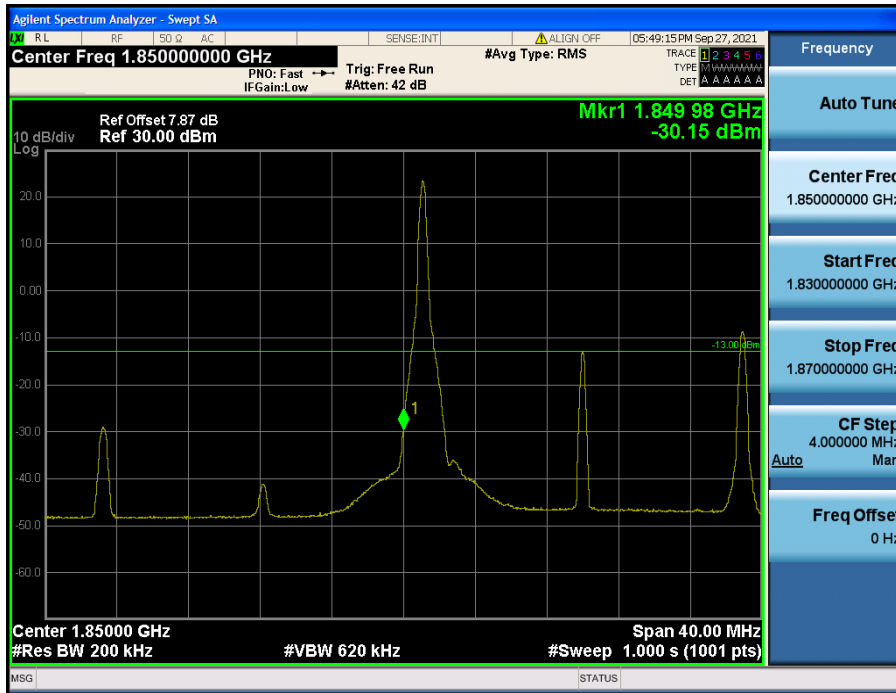
LTE Band 25(2) / 20 MHz / QPSK - RB Size/Offset (1/0)
