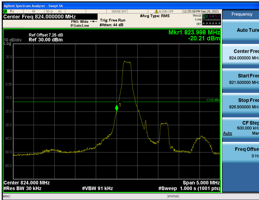
LTE Band 26(5) / 1.4 MHz / 16QAM - RB Size/Offset (1/0)
