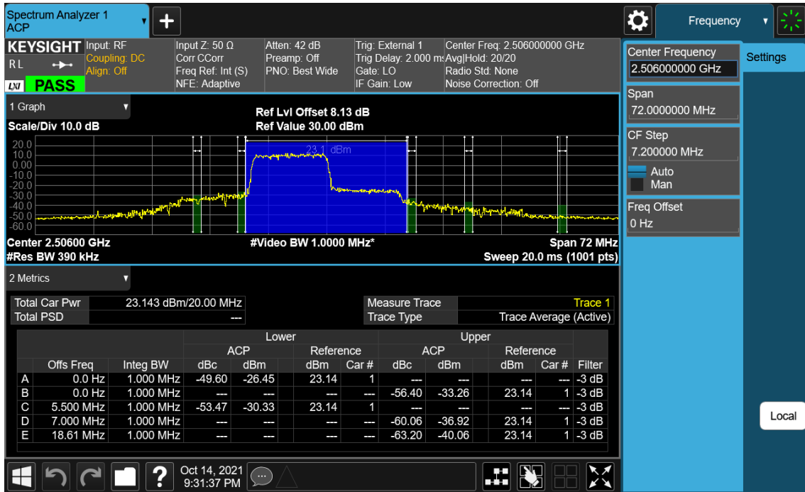
LTE Band 41(38) / 20 MHz / QPSK - RB Size/Offset (50/0)
