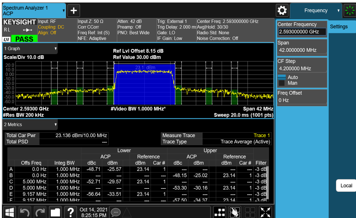
LTE Band 41(38) / 10 MHz / QPSK - RB Size/Offset (50/0)
