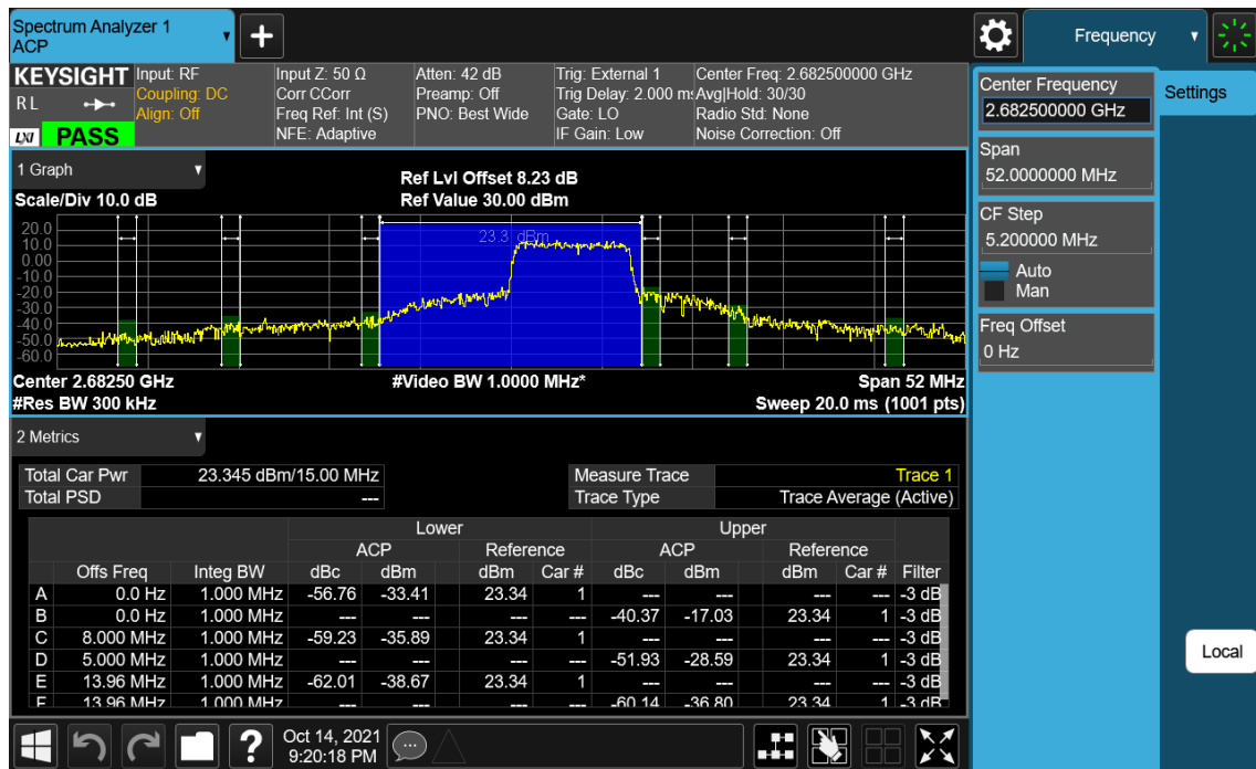
LTE Band 41(38) / 15 MHz / QPSK - RB Size/Offset (36/39)
