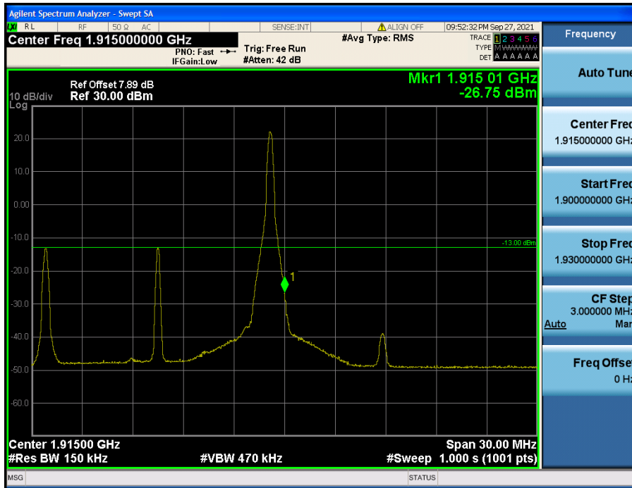
LTE Band 25(2) / 15 MHz / 16QAM - RB Size/Offset (1/74)
