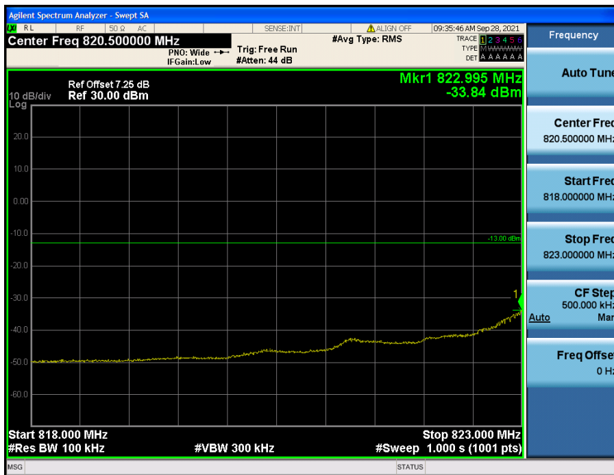
LTE Band 26(5) / 1.4 MHz / QPSK - RB Size/Offset (6/0)
