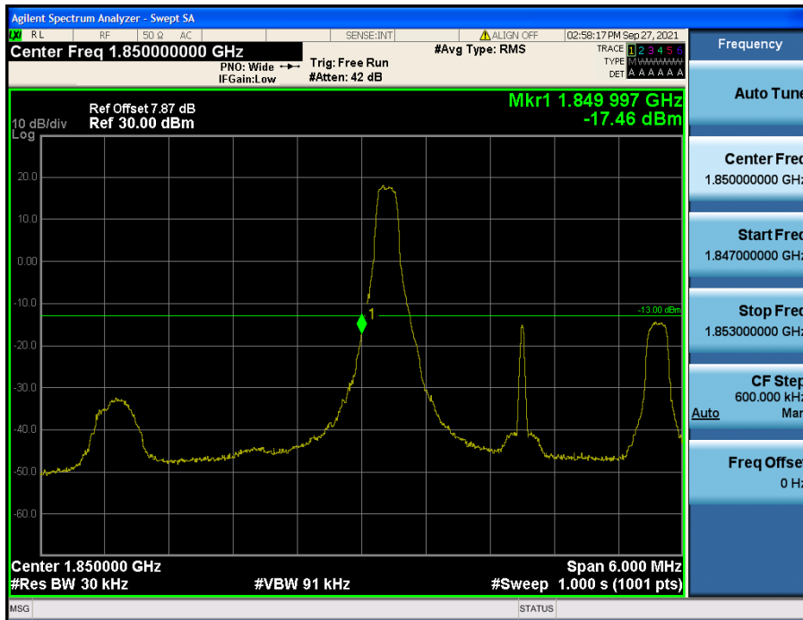
LTE Band 25(2) / 3 MHz / QPSK - RB Size/Offset (1/0)
