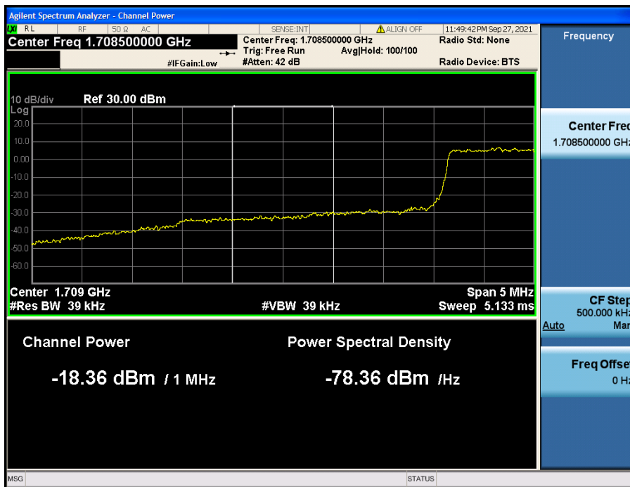
LTE Band 66(4) / 3 MHz / QPSK - RB Size/Offset (15/0)
