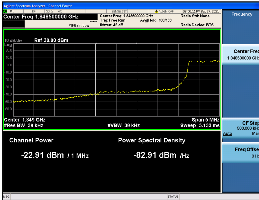
LTE Band 25(2) / 5 MHz / QPSK Offset/Size (12/0)
