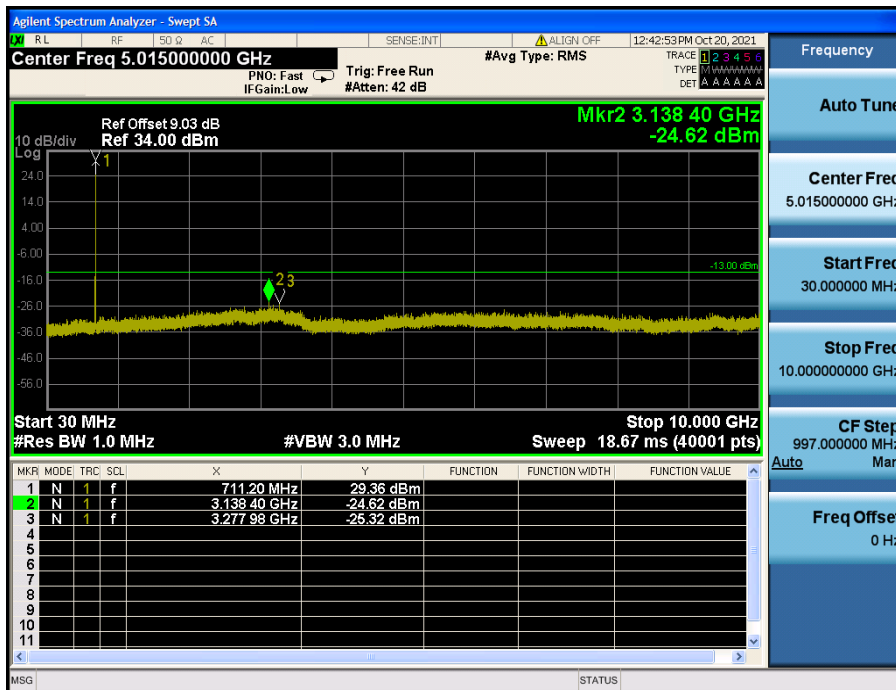
LTE Band 12 / 10 MHz / 16QAM - RB Size/Offset (1/25) – High Channel
