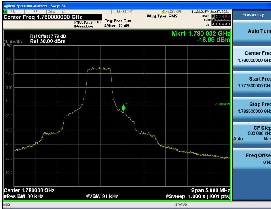
LTE Band 66(4) / 1.4 MHz / QPSK - RB Size/Offset (3/3)
