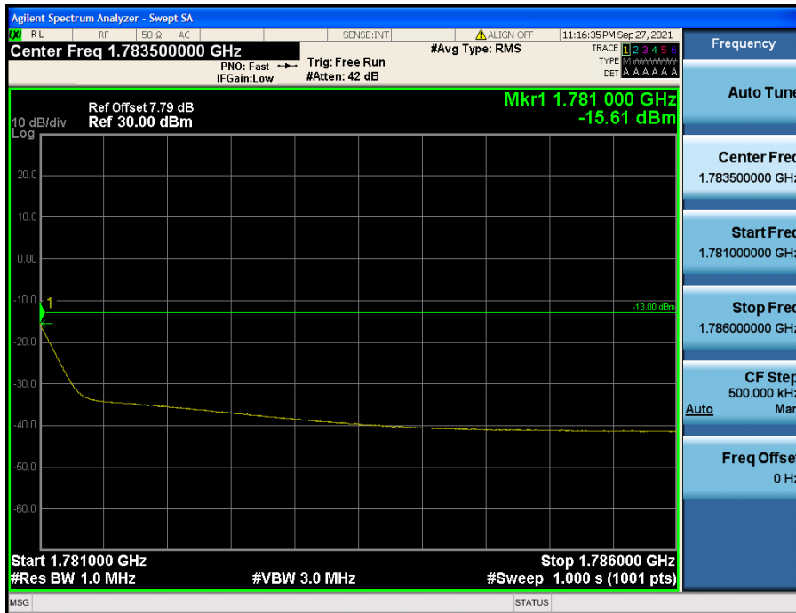
LTE Band 66(4) / 1.4 MHz / QPSK - RB Size/Offset (1/2)
