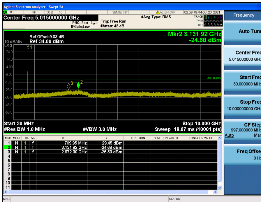
LTE Band 12 / 5 MHz / 16QAM - RB Size/Offset (1/24) – Mid Channel
