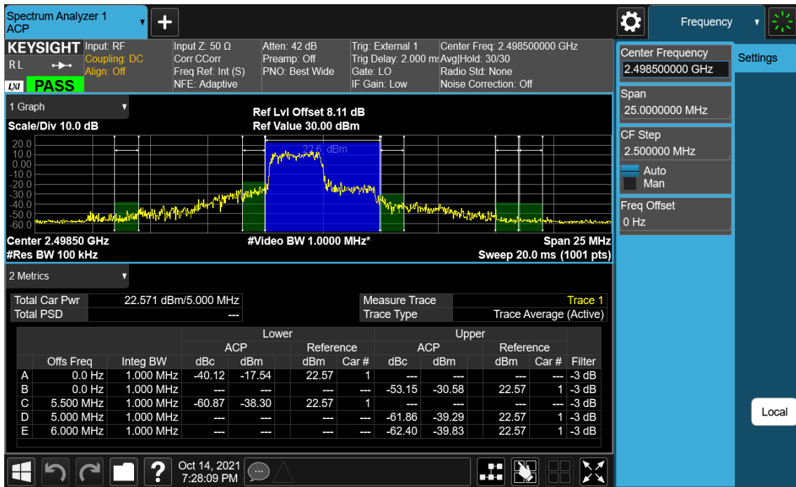
LTE Band 41(38) / 5 MHz / QPSK - RB Size/Offset (12/0)
