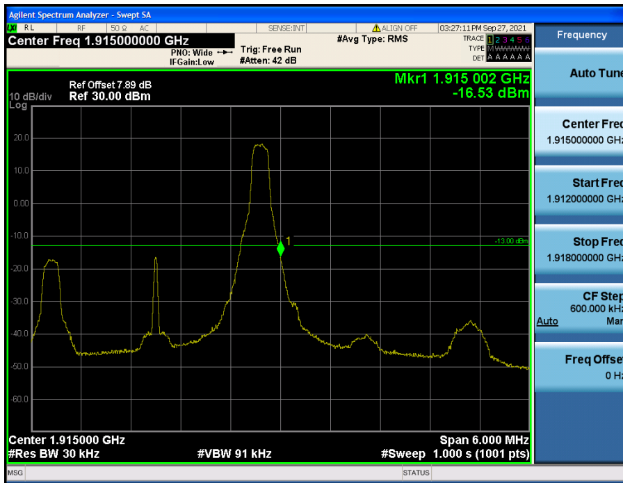
LTE Band 25(2) / 3 MHz / QPSK - RB Size/Offset (1/14)
