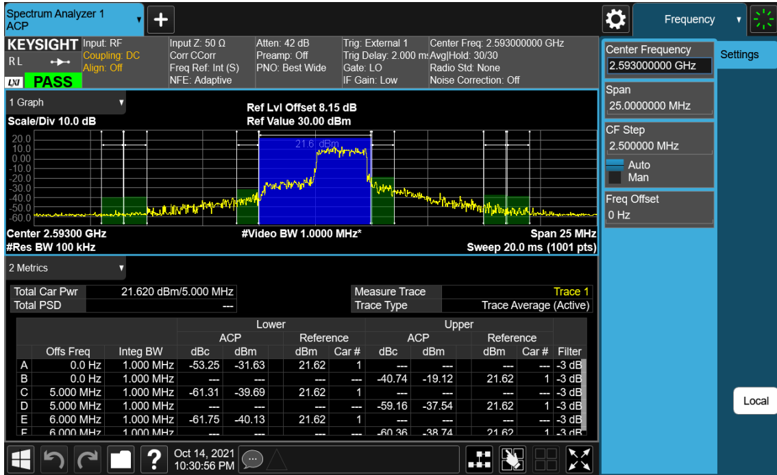
LTE Band 41(38) / 5 MHz / 16QAM - RB Size/Offset (12/13)
