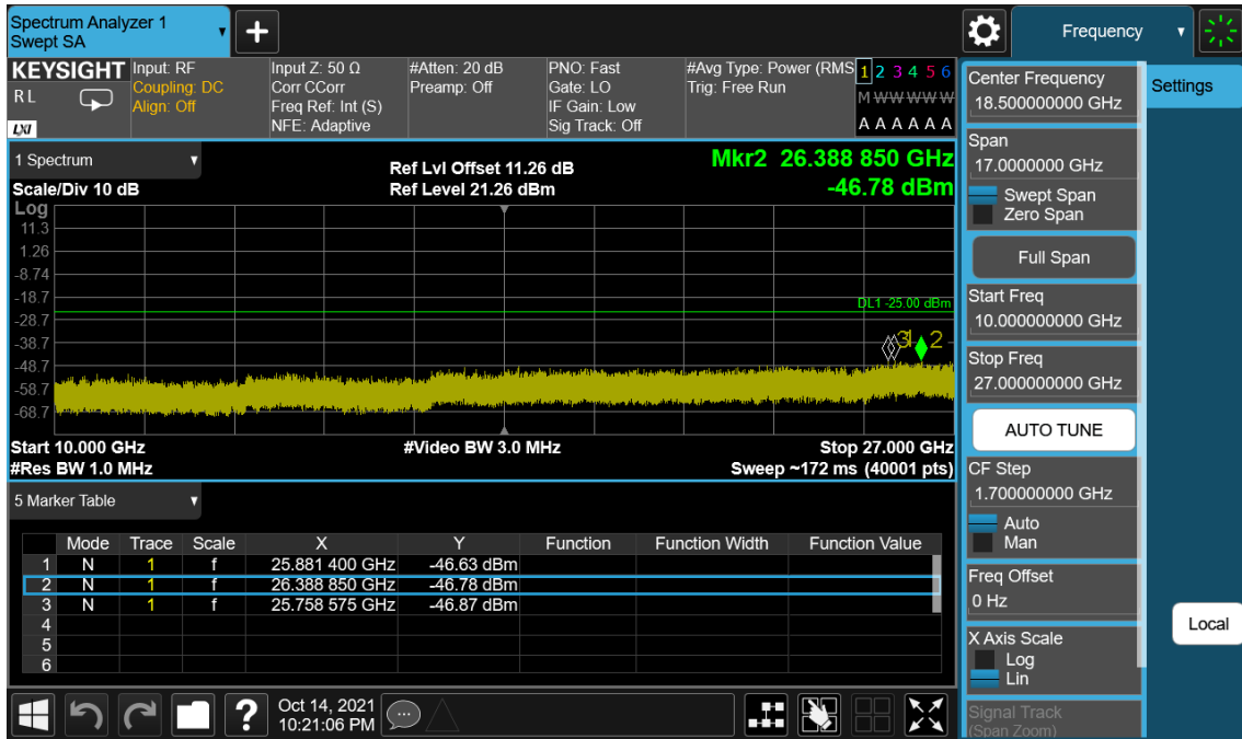
LTE Band 41(38) / 5 MHz / 16QAM - RB Size/Offset (25/0) – Low Channel
