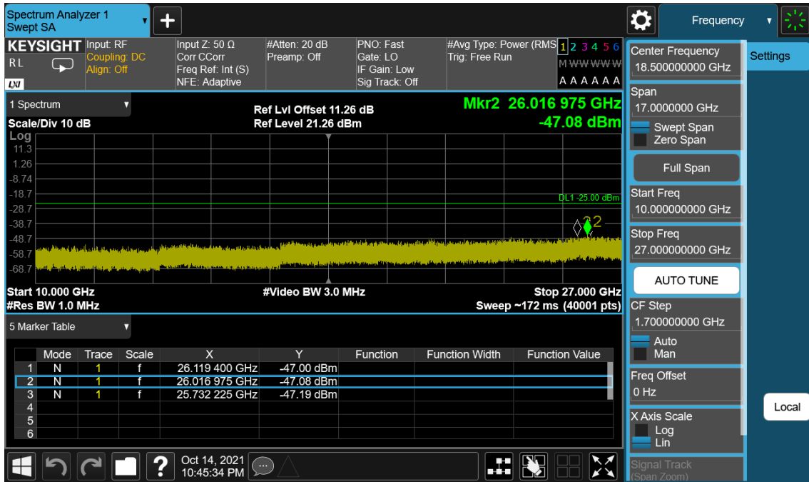
LTE Band 41(38) / 5 MHz / 16QAM - RB Size/Offset (25/0) – High Channel
