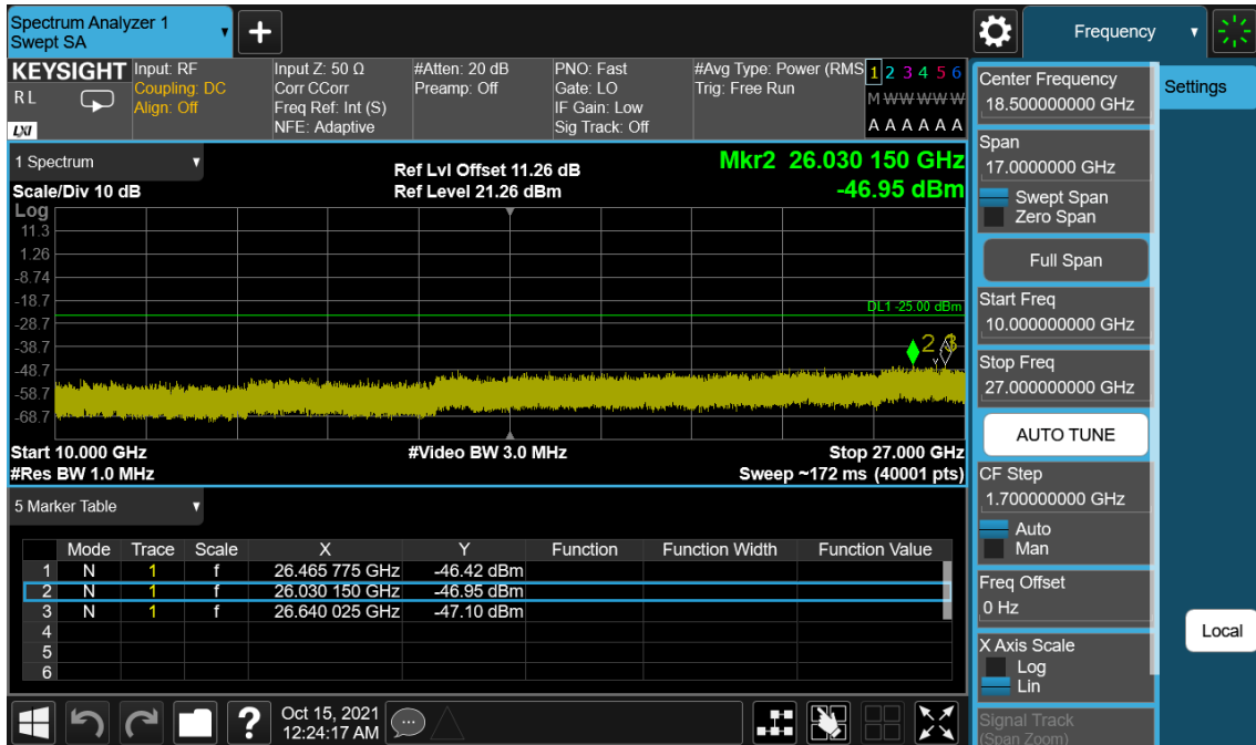
LTE Band 41(38) / 20 MHz / 16QAM - RB Size/Offset (50/50) –Low Channel
