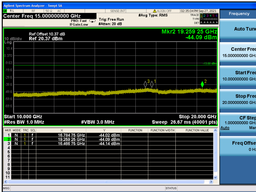
LTE Band 25(2) / 1.4 MHz / QPSK - RB Size/Offset (3/0) – Mid Channel
