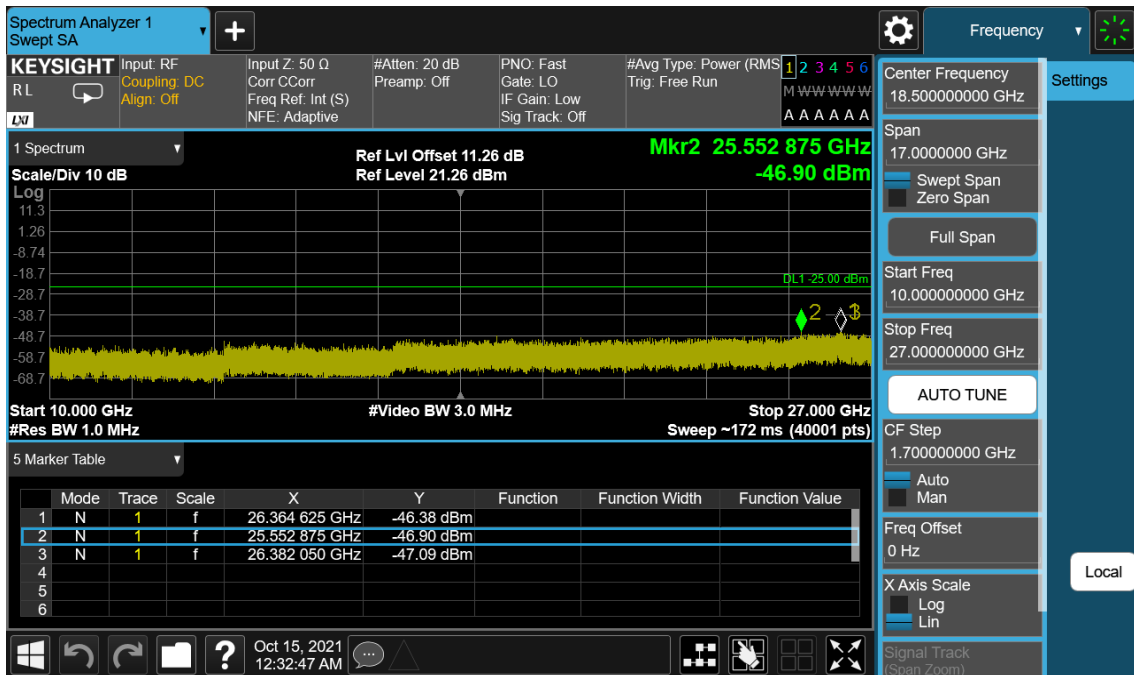
LTE Band 41(38) / 20 MHz / 16QAM - RB Size/Offset (1/99)–Mid Channel
