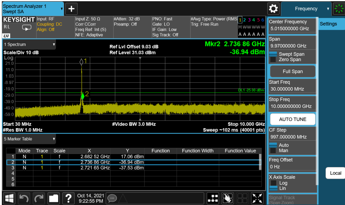
LTE Band 41(38) / 15 MHz / QPSK - RB Size/Offset (75/0) – High Channel
