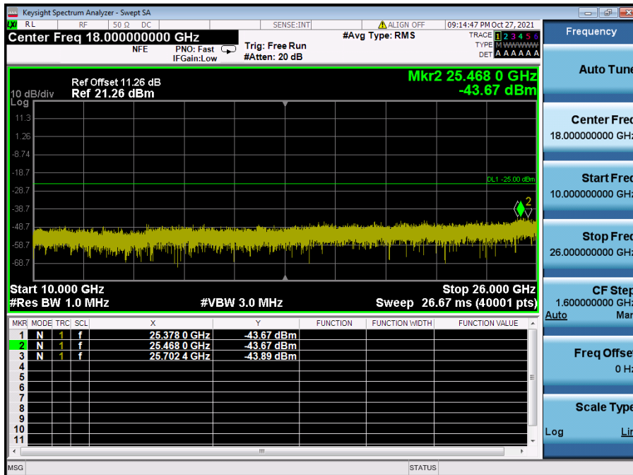
LTE Band 7 / 15 MHz / 16QAM - RB Size/Offset (36/18) – High Channel
