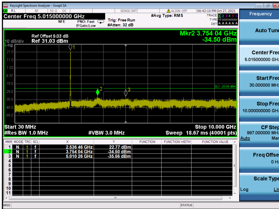
LTE Band 7 / 15 MHz / QPSK - RB Size/Offset (36/39) – Mid Channel
