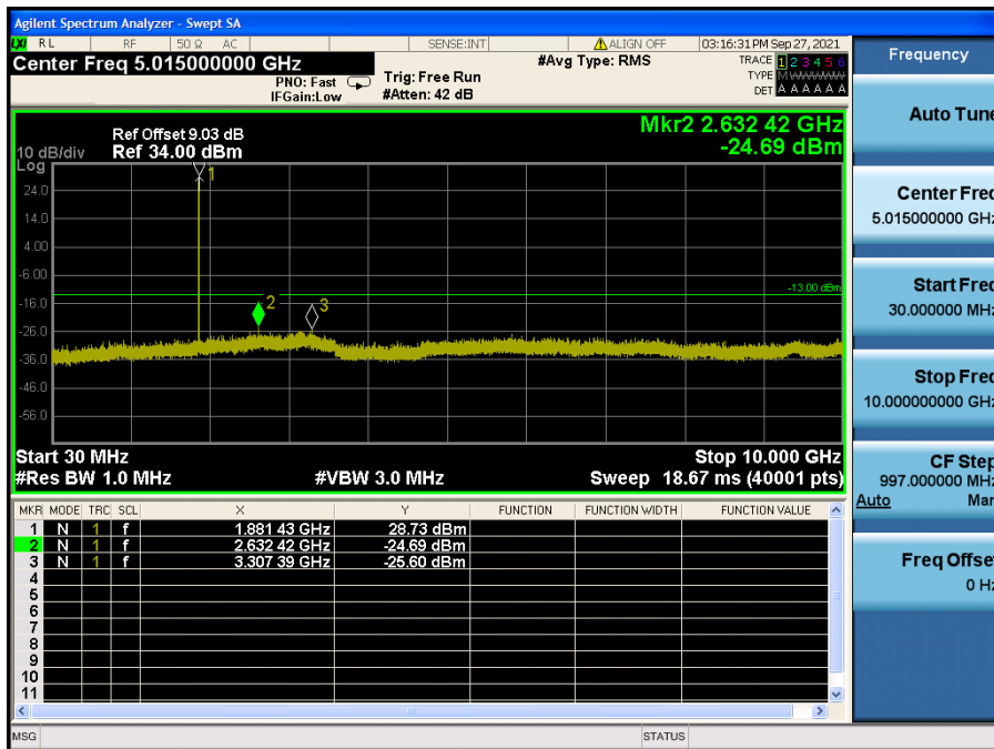
LTE Band 25(2) / 3 MHz / QPSK - RB Size/Offset (1/0) – Mid Channel
