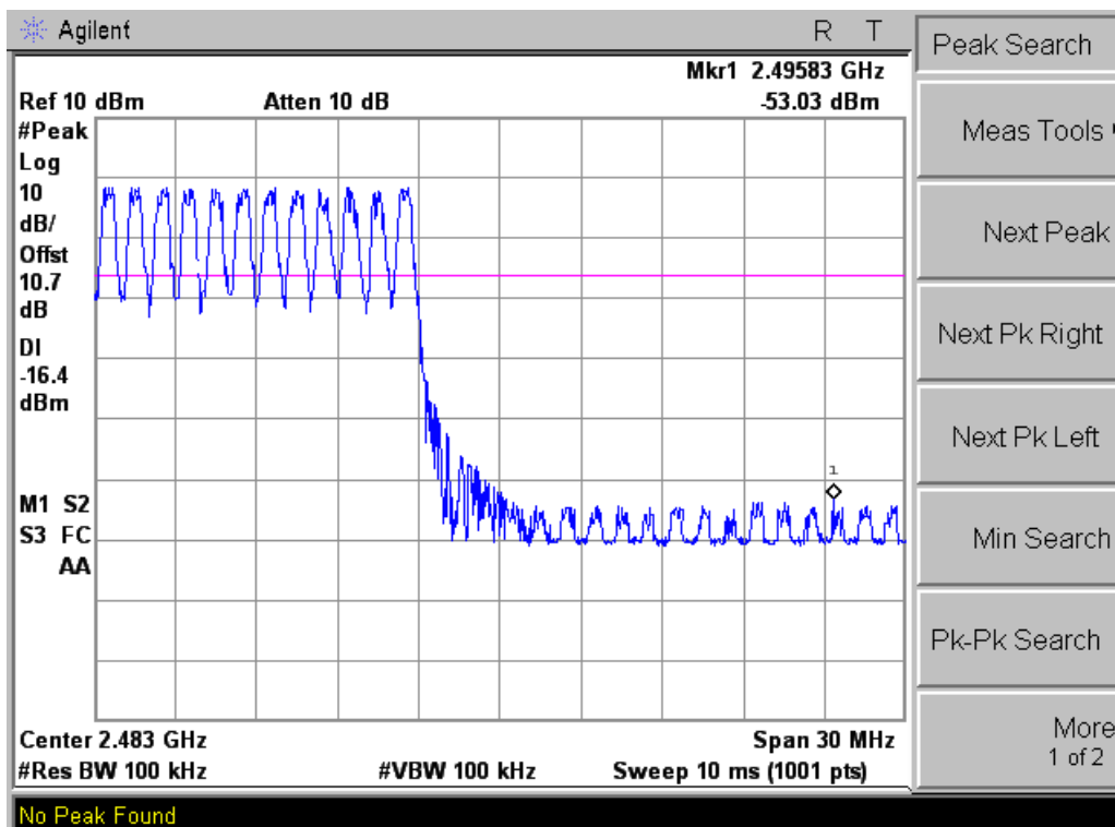
– Band edge higher side (GFSK) Hopping On–
