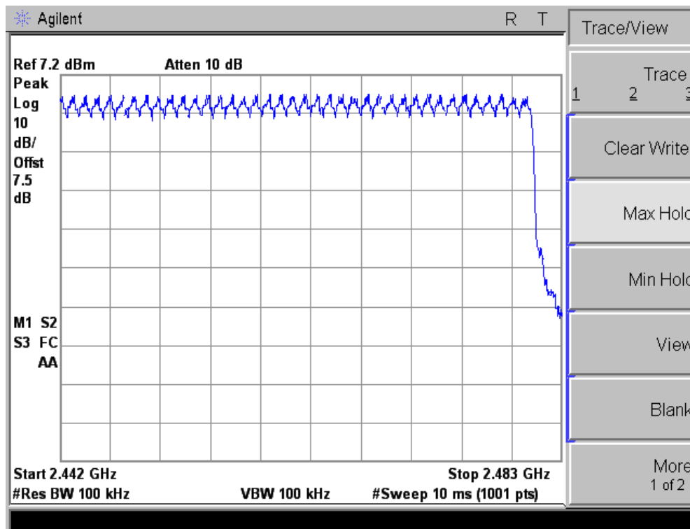
– Number of hopping channel (8DPSK) –
