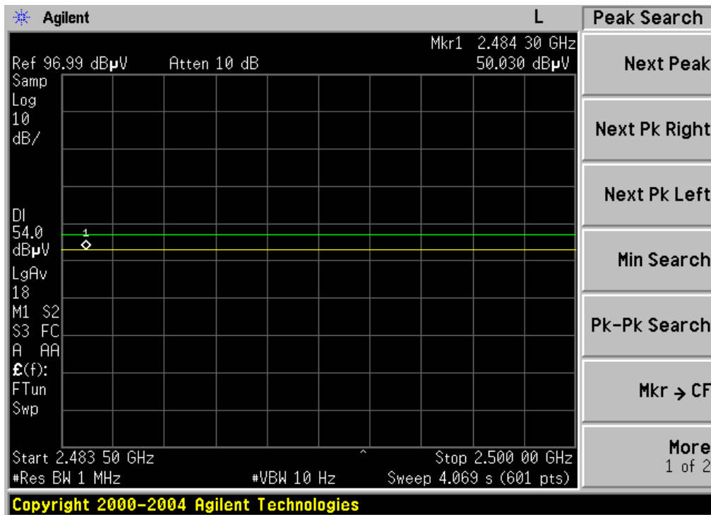
< Higher side band-edge GFSK_average detector >
