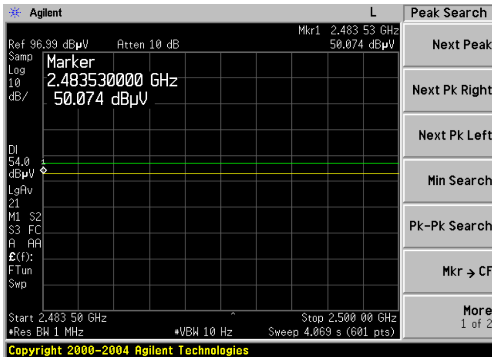
< Higher side band-edge 8DPSK_average detector >
