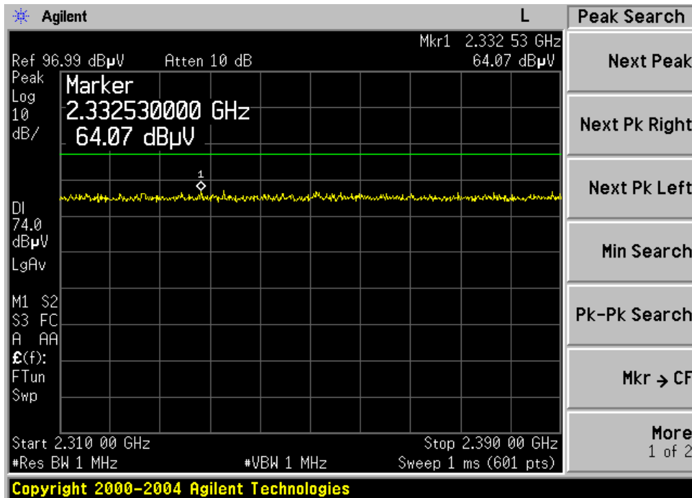
< Lower side band-edge GFSK_peak detector >
