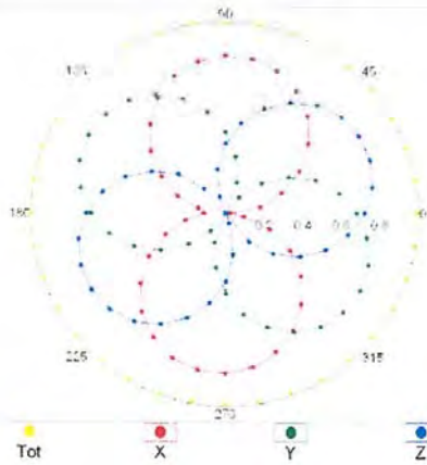
f=600 MHz,TEM
