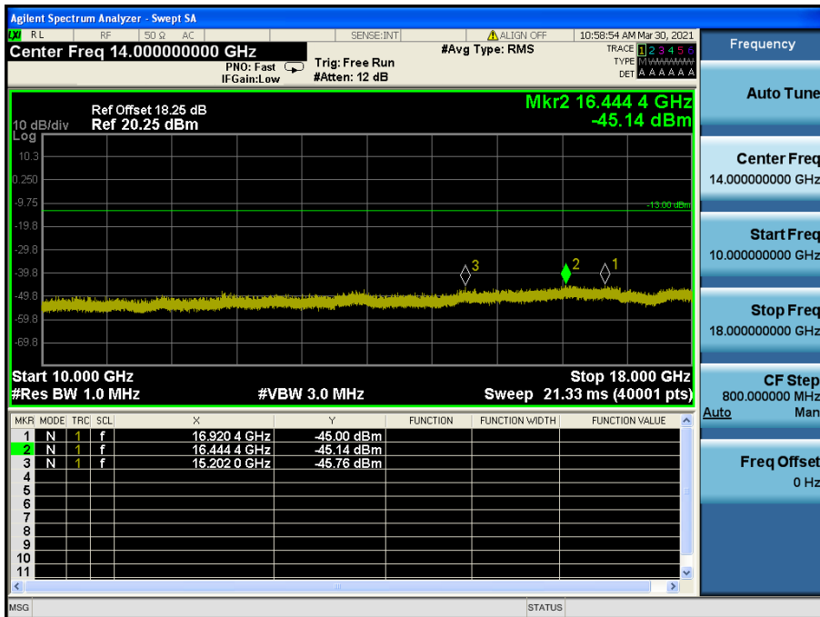
LTE Band 66(4) / 1.4 MHz / QPSK - RB Size/Offset (3/0) – Mid Channel
