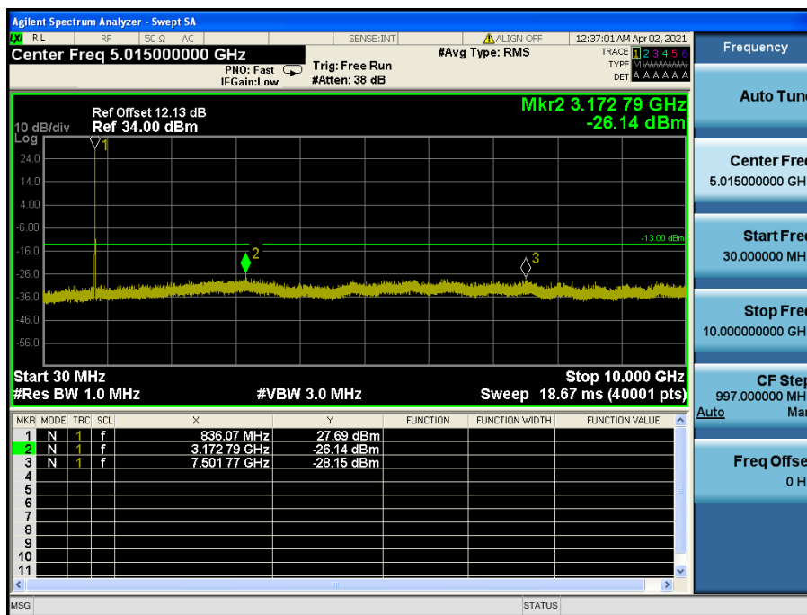
LTE Band 26(5) / 10 MHz / 16QAM - RB Size/Offset (25/12) – Mid Channel
