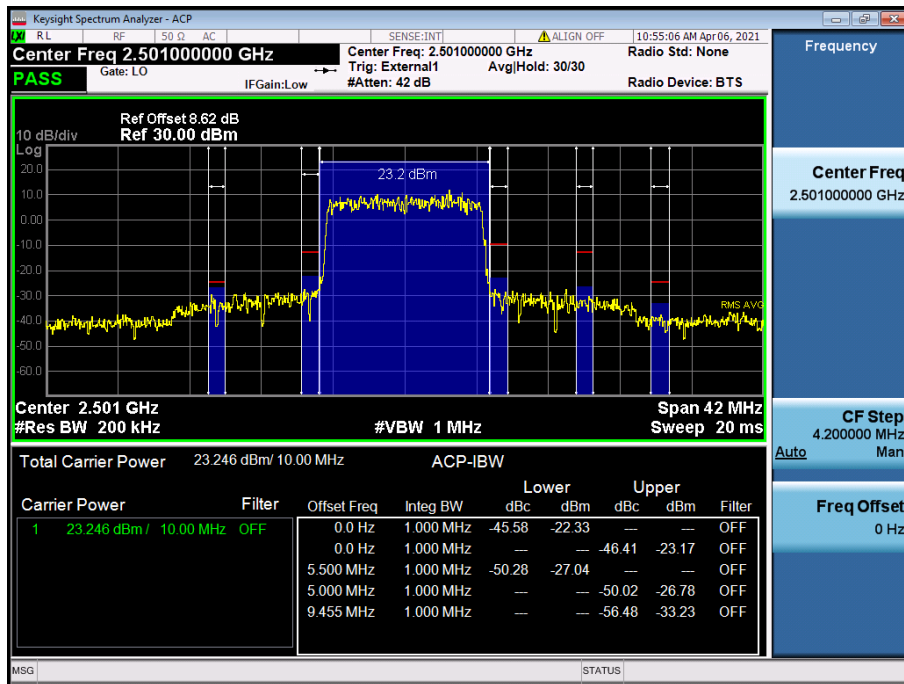
LTE Band 41(38) / 10 MHz / QPSK - RB Size/Offset (50/0)
