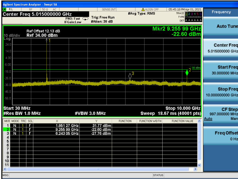
LTE Band 25(2) / 20 MHz / 16QAM - RB Size/Offset (1/0) –Low Channel
