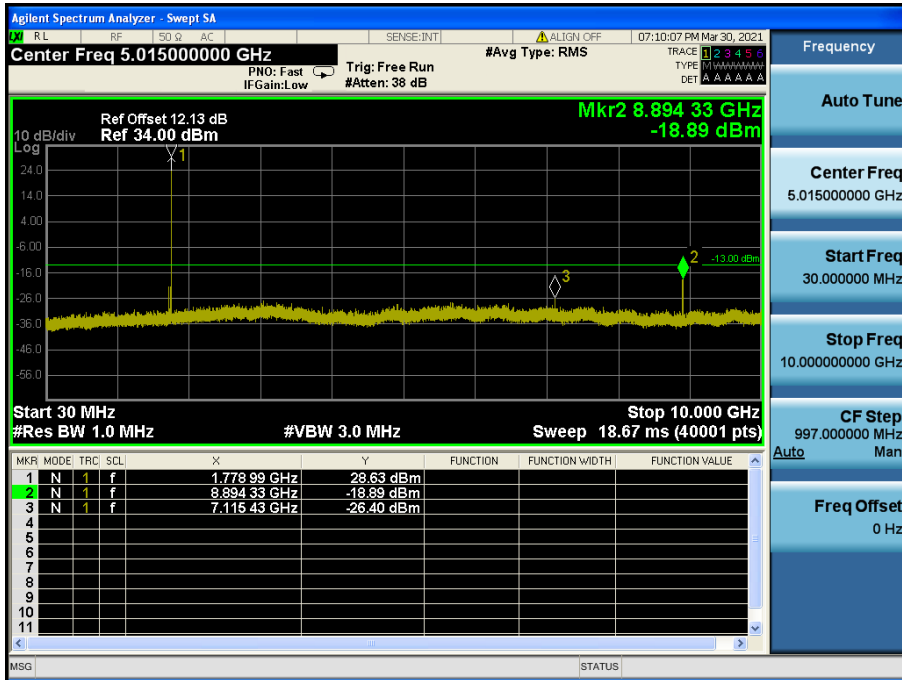
LTE Band 66(4) / 20 MHz / 16QAM - RB Size/Offset (1/99) – High Channel
