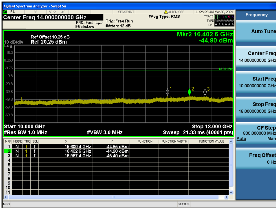
LTE Band 66(4) / 3 MHz / QPSK - RB Size/Offset (1/7) – Low Channel
