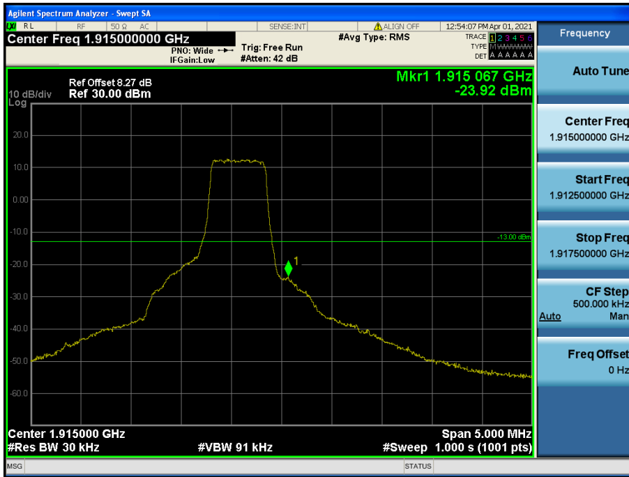
LTE Band 25(2) / 1.4 MHz / 16QAM - RB Size/Offset (3/3)
