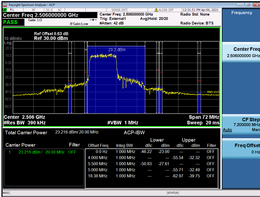
LTE Band 41(38) / 20 MHz / QPSK - RB Size/Offset (50/0)
