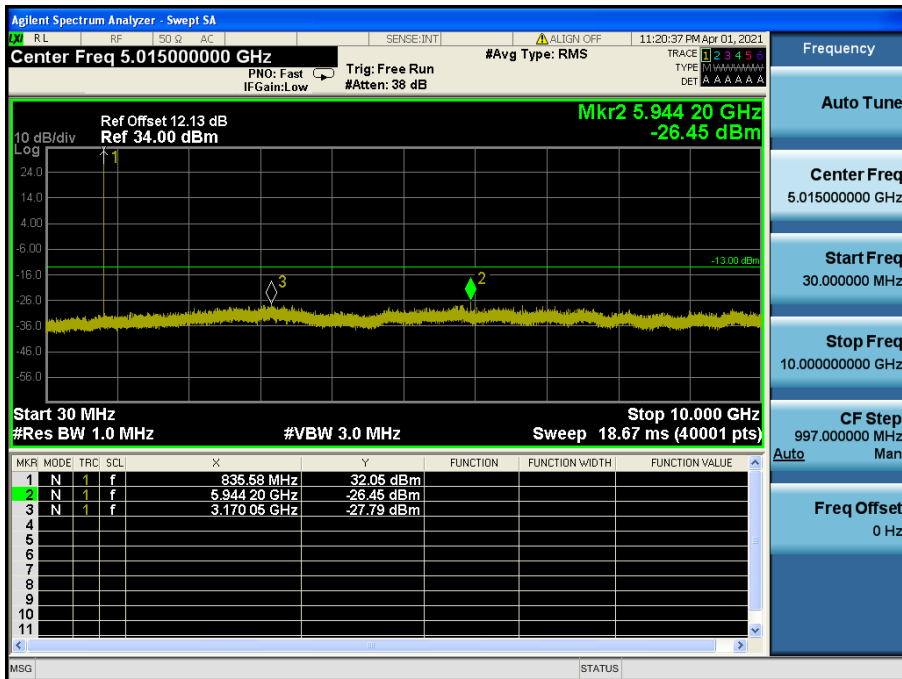
LTE Band 26(5) / 3 MHz / 16QAM - RB Size/Offset (1/0) – Mid Channel
