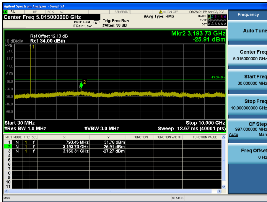
LTE Band 14 / 5 MHz / 16QAM - RB Size/Offset (1/0) – High Channel
