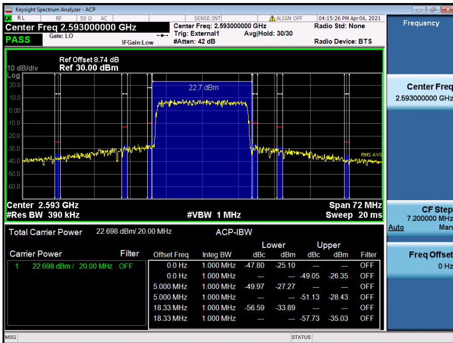
LTE Band 41(38) / 20 MHz / 16QAM - RB Size/Offset (100/0)
