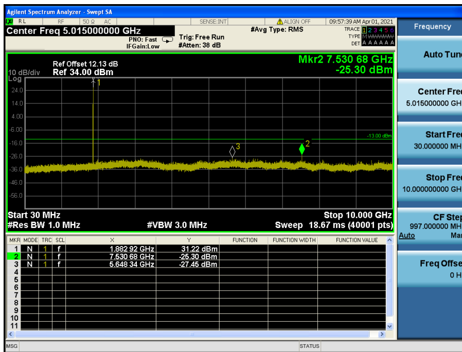
LTE Band 25(2) / 20 MHz / QPSK - RB Size/Offset (1/50)–Mid Channel
