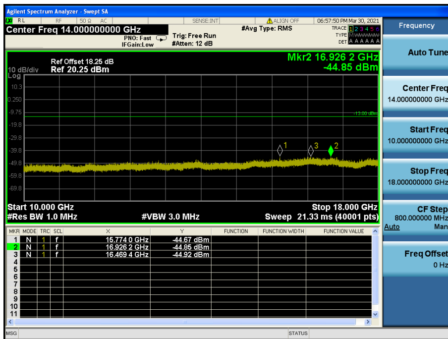
LTE Band 66(4) / 20 MHz / 16QAM - RB Size/Offset (50/0)–Mid Channel
