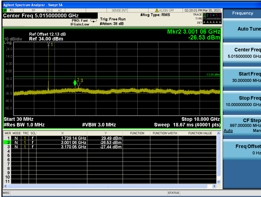
LTE Band 66(4) / 20 MHz / QPSK - RB Size/Offset (1/99) –Low Channel
