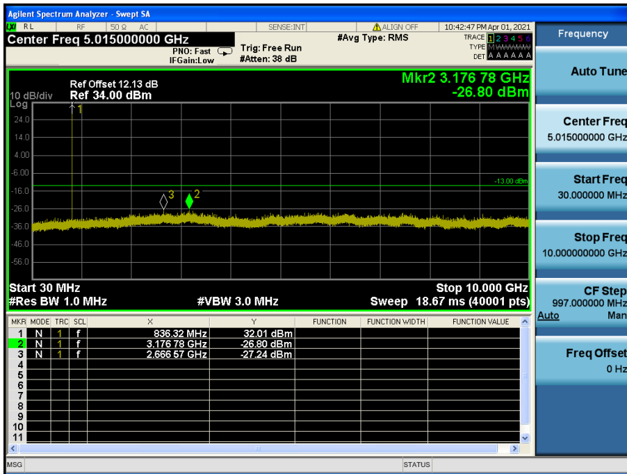
LTE Band 26(5) / 1.4 MHz / 16QAM - RB Size/Offset (1/0) – Mid Channel
