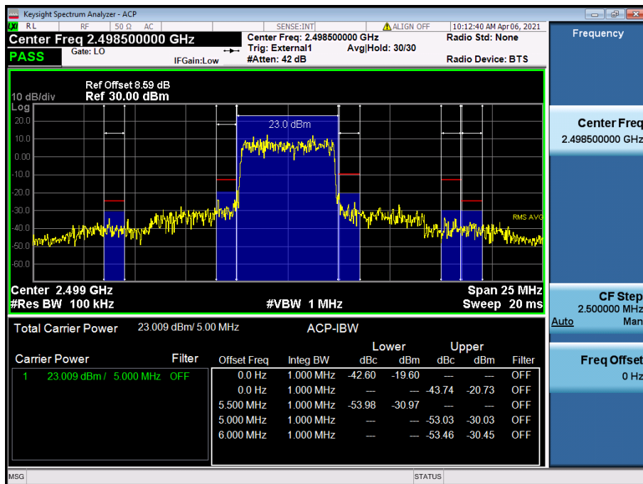
LTE Band 41(38) / 5 MHz / QPSK - RB Size/Offset (25/0)
