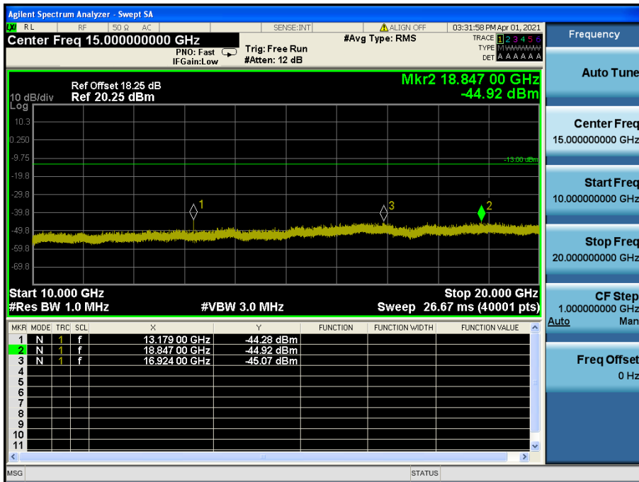
LTE Band 25(2) / 5 MHz / 16QAM - RB Size/Offset (1/12) – Mid Channel
