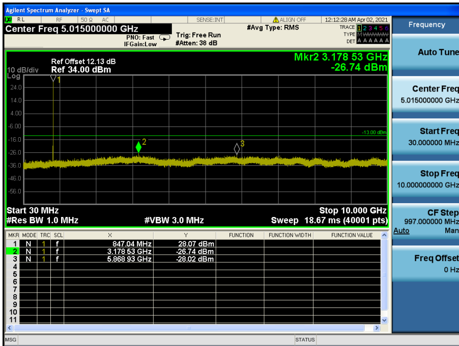
LTE Band 26(5) / 5 MHz / 16QAM - RB Size/Offset (12/6) – High Channel
