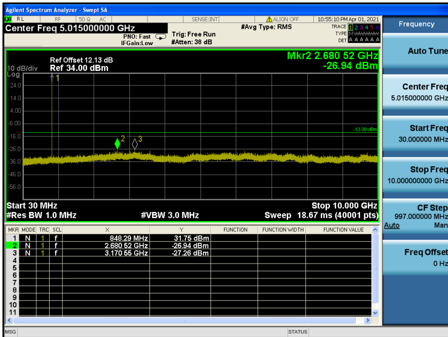
LTE Band 26(5) / 1.4 MHz / 16QAM- RB Size/Offset (3/0) – High Channel
