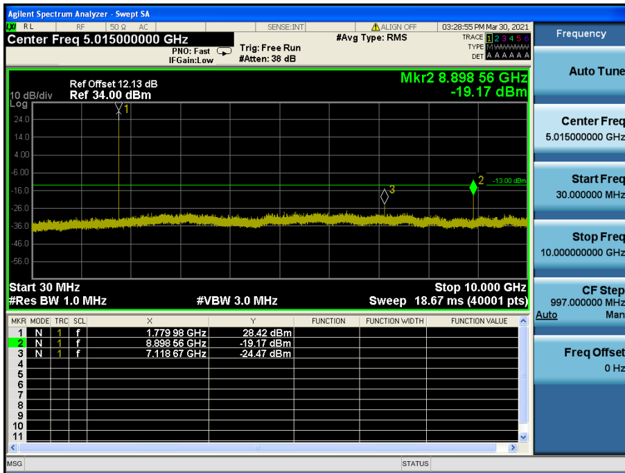
LTE Band 66(4) / 1.4 MHz / 16QAM - RB Size/Offset (1/5) – High Channel
