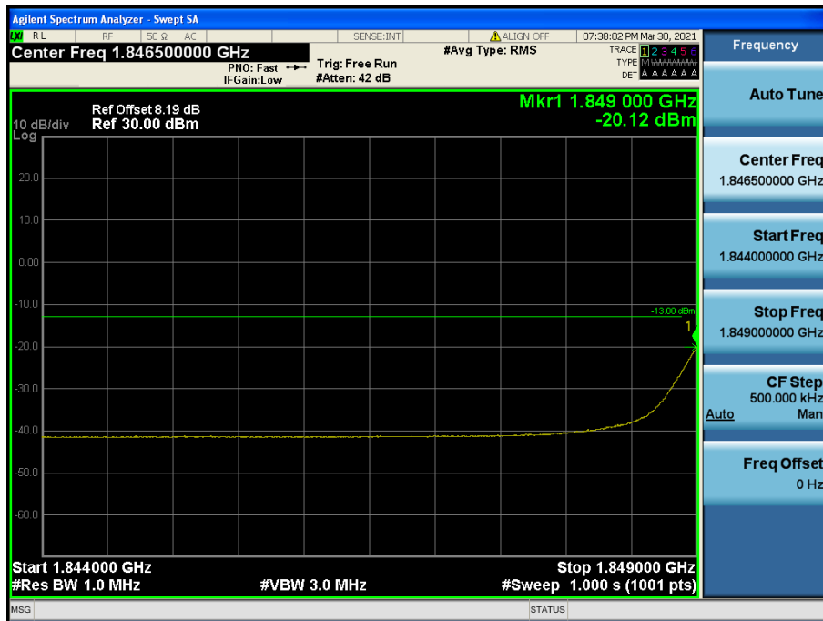
LTE Band 25(2) / 1.4 MHz / QPSK - RB Size/Offset (3/2)
