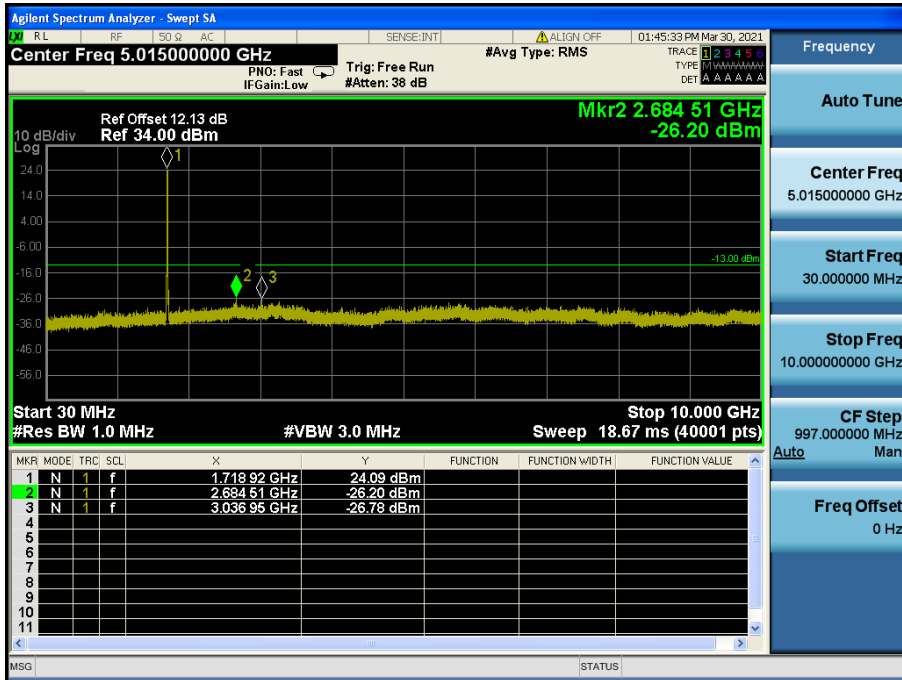
LTE Band 66(4) / 15 MHz / QPSK - RB Size/Offset (36/39)–Low Channel
