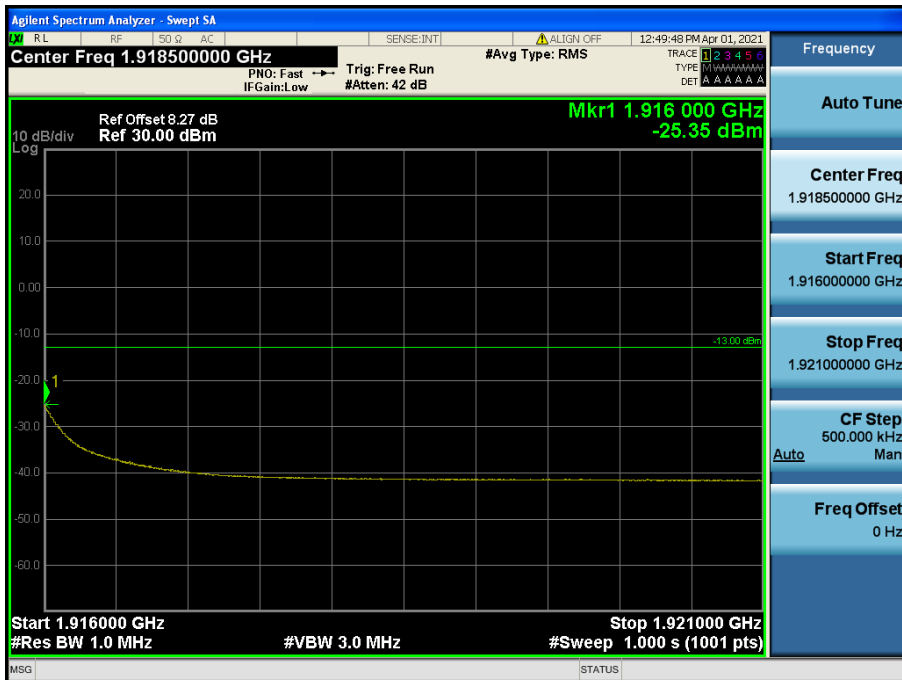
LTE Band 25(2) / 1.4 MHz / 16QAM - RB Size/Offset (3/0)
