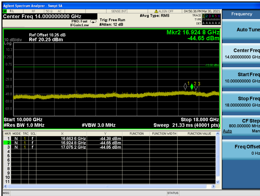
LTE Band 66(4) / 5 MHz / 16QAM - RB Size/Offset (1/24) – High Channel
