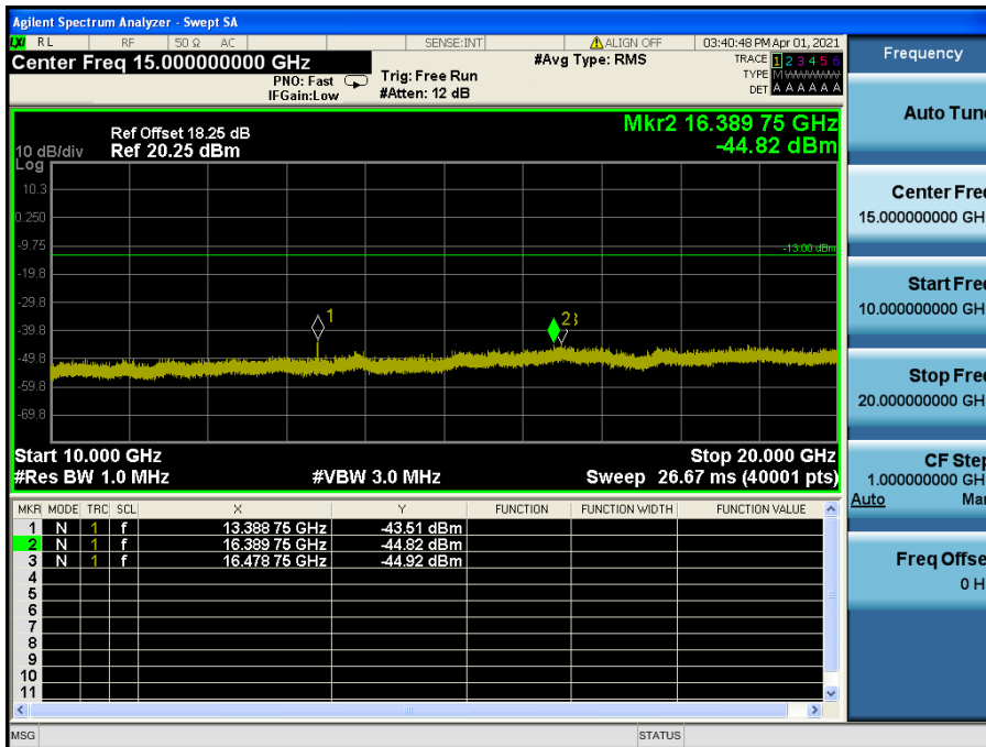
LTE Band 25(2) / 5 MHz / 16QAM - RB Size/Offset (1/12) – High Channel
