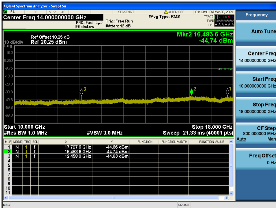
LTE Band 66(4) / 3 MHz / 16QAM - RB Size/Offset (1/14) – High Channel
