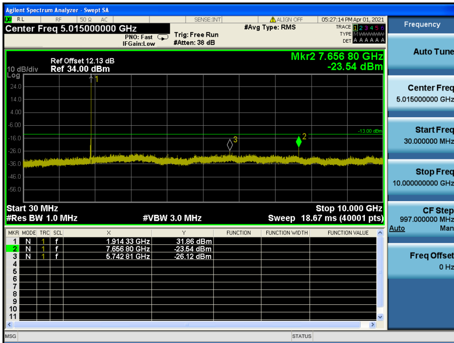
LTE Band 25(2) / 15 MHz / 16QAM - RB Size/Offset (1/74) – High Channel
