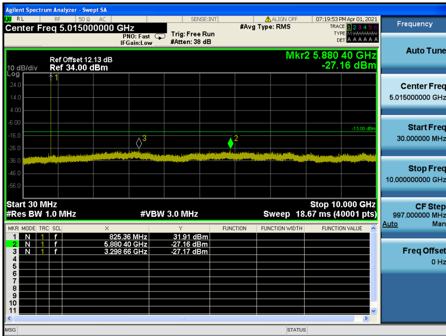
LTE Band 26(5) / 1.4 MHz / QPSK - RB Size/Offset (1/5) – Low Channel
