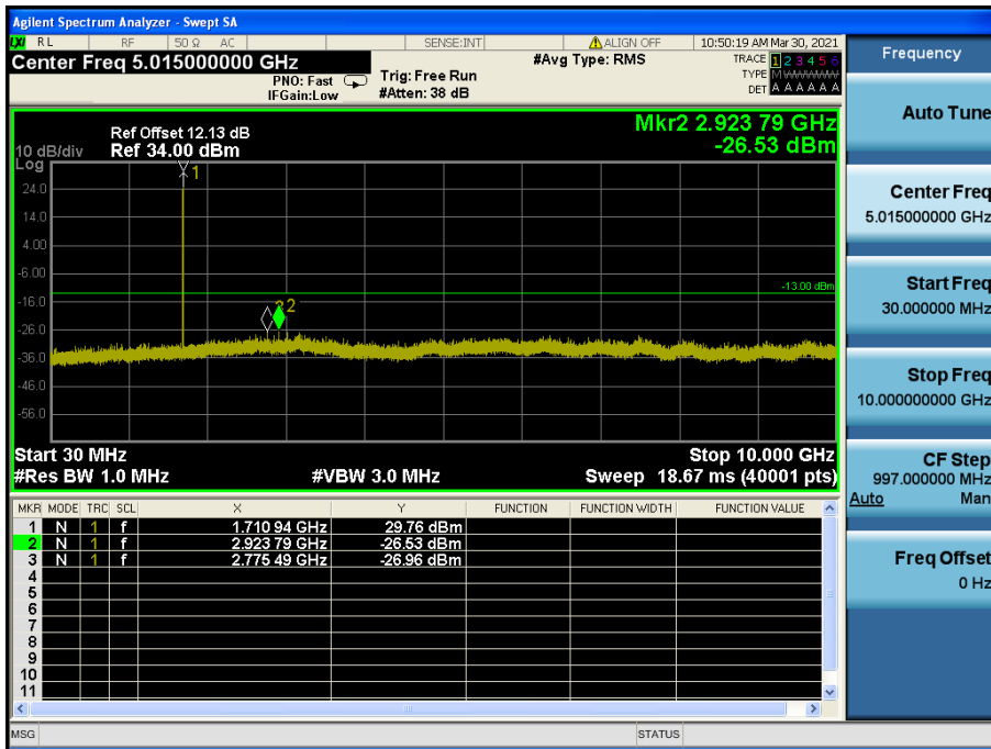
LTE Band 66(4) / 1.4 MHz / QPSK - RB Size/Offset (3/2) – Low Channel
