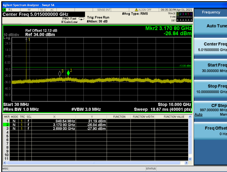
LTE Band 26(5) / 10 MHz / QPSK - RB Size/Offset (1/49) – High Channel
