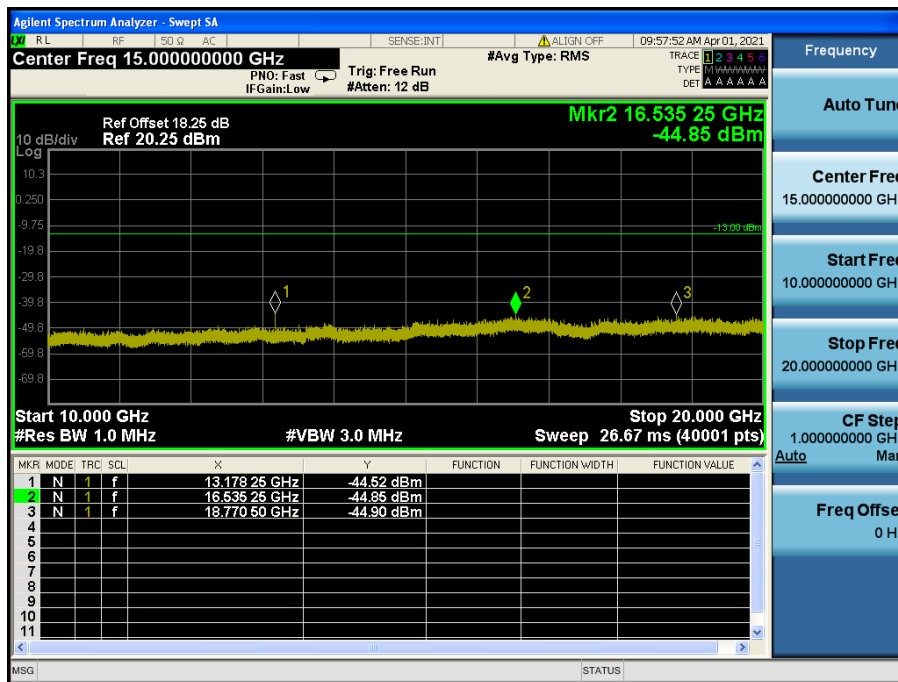
LTE Band 25(2) / 20 MHz / QPSK - RB Size/Offset (1/50)–Mid Channel
