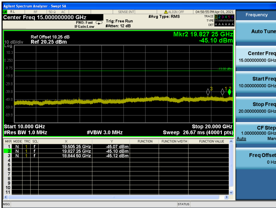
LTE Band 25(2) / 15 MHz / 16QAM- RB Size/Offset (1/0)–Low Channel
