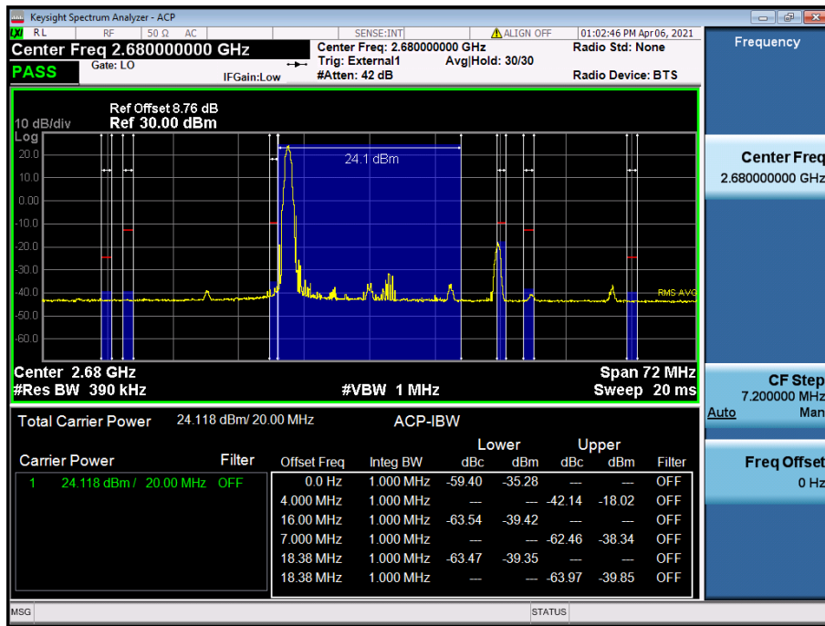
LTE Band 41(38) / 20 MHz / QPSK - RB Size/Offset (1/0)
