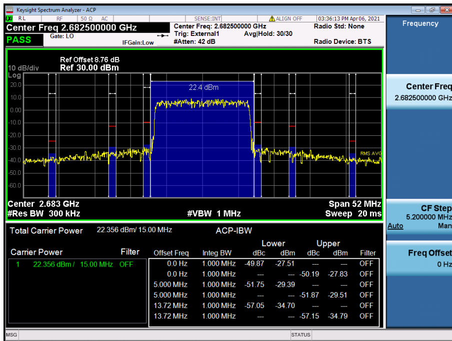
LTE Band 41(38) / 15 MHz / 16QAM - RB Size/Offset (75/0)
