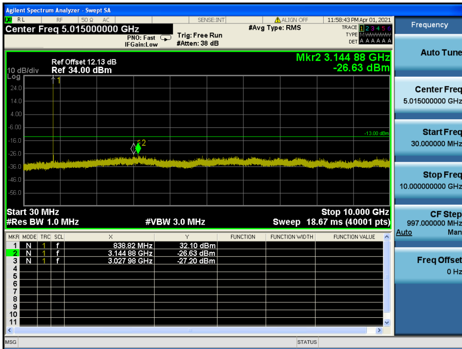
LTE Band 26(5) / 5 MHz / 16QAM - RB Size/Offset (1/24) – Mid Channel
