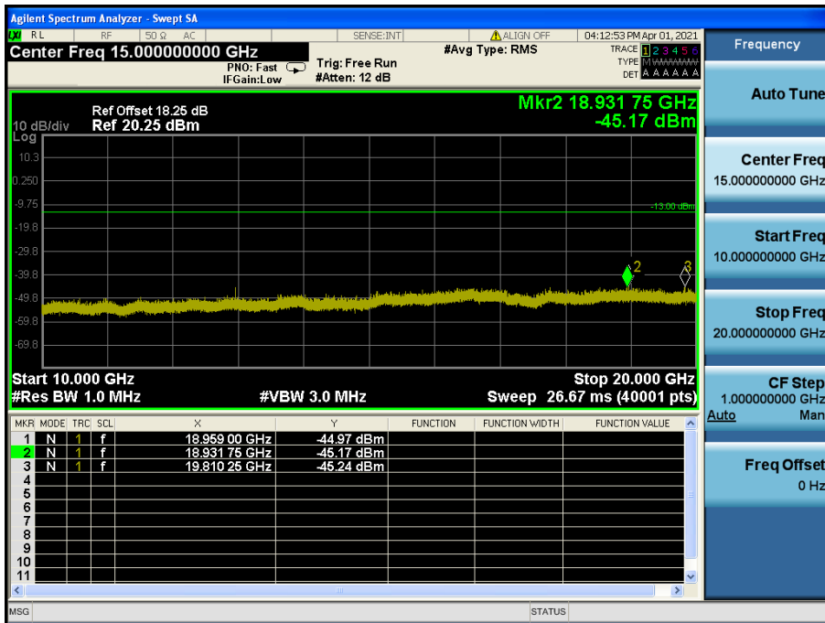
LTE Band 25(2) / 10 MHz / 16QAM - RB Size/Offset (1/0) – Low Channel
