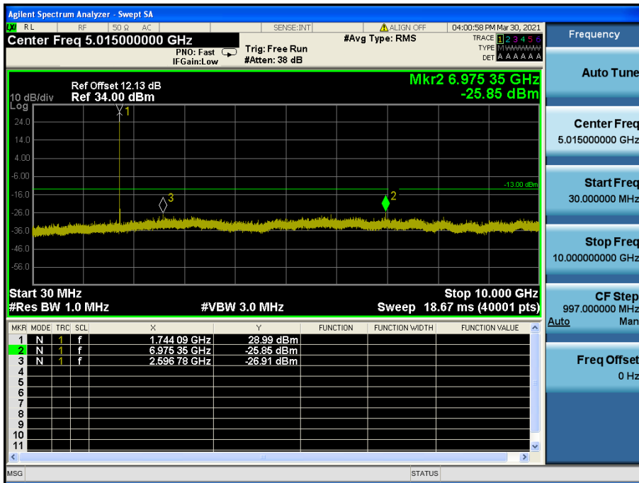
LTE Band 66(4) / 3 MHz / 16QAM - RB Size/Offset (1/0) – Mid Channel
