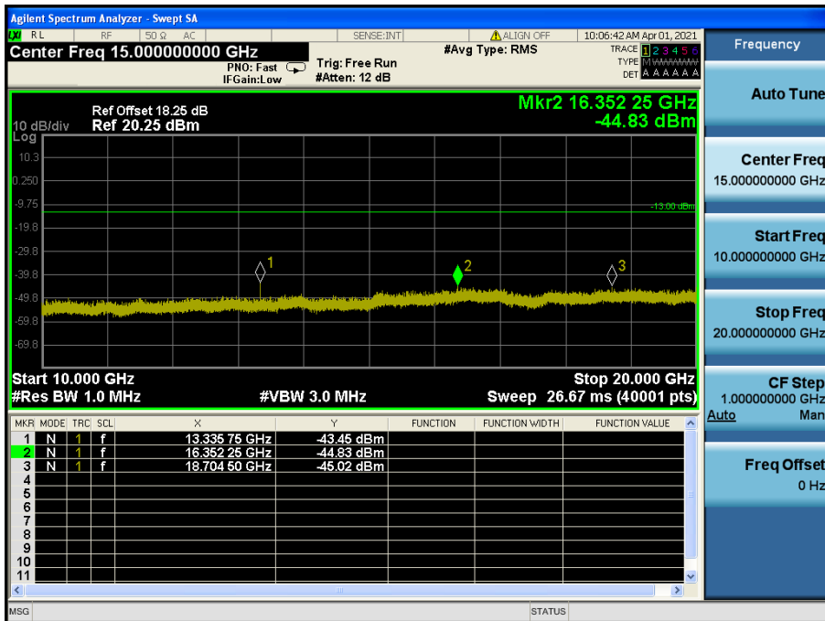
LTE Band 25(2) / 20 MHz / QPSK - RB Size/Offset (1/50) – High Channel
