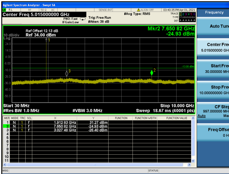
LTE Band 25(2) / 5 MHz / 16QAM - RB Size/Offset (1/12) – High Channel
