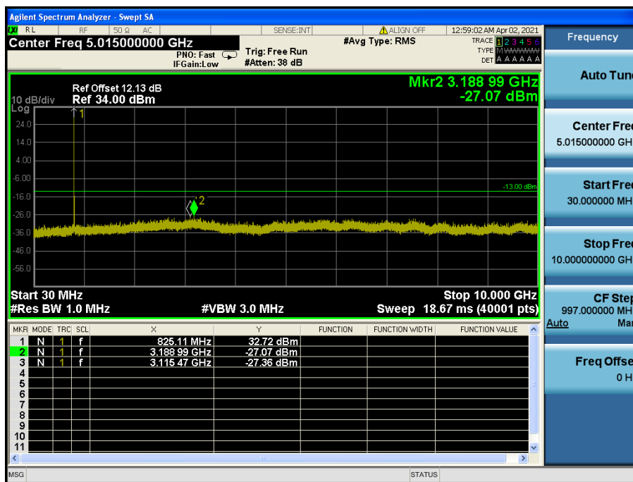
LTE Band 26 / 15 MHz / 16QAM - RB Size/Offset (1/0) – High Channel
