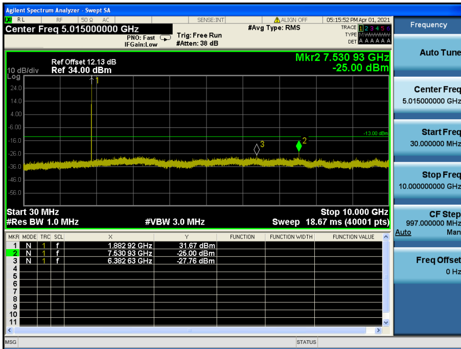
LTE Band 25(2) / 15 MHz / 16QAM - RB Size/Offset (1/36) – Mid Channel
