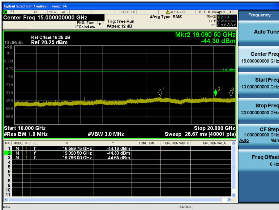
LTE Band 25(2) / 10 MHz / 16QAM - RB Size/Offset (1/25) – Mid Channel
