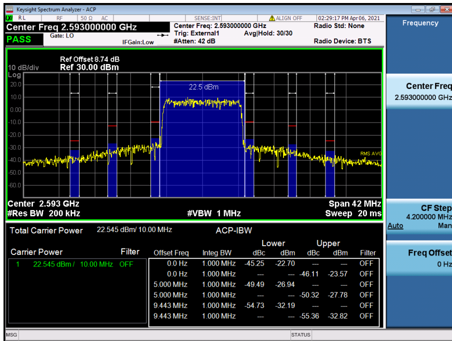
LTE Band 41(38) / 10 MHz / 16QAM - RB Size/Offset (50/0)
