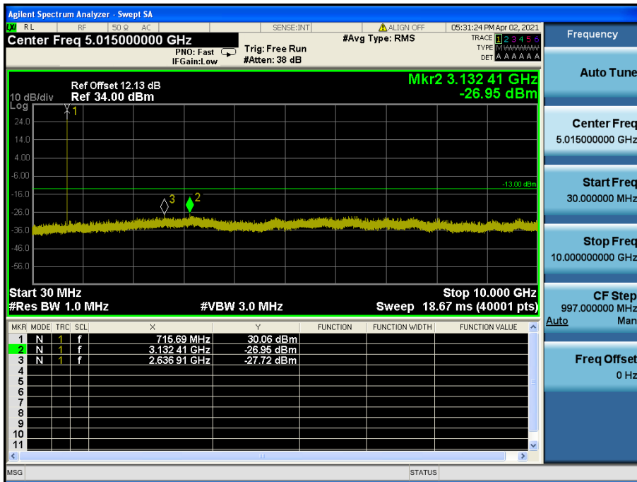
LTE Band 12 / 1.4 MHz / 16QAM - RB Size/Offset (6/0) – High Channel
