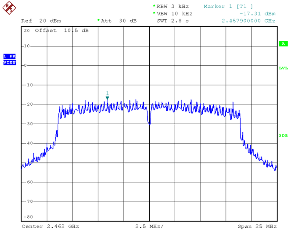
802.11n20 - Channel 11
