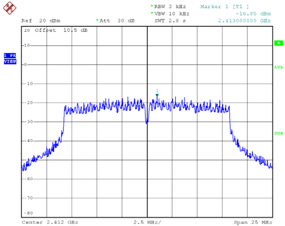
802.11g - Channel 1
