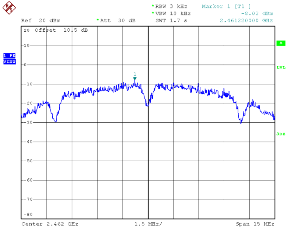
802.11b - Channel 11
