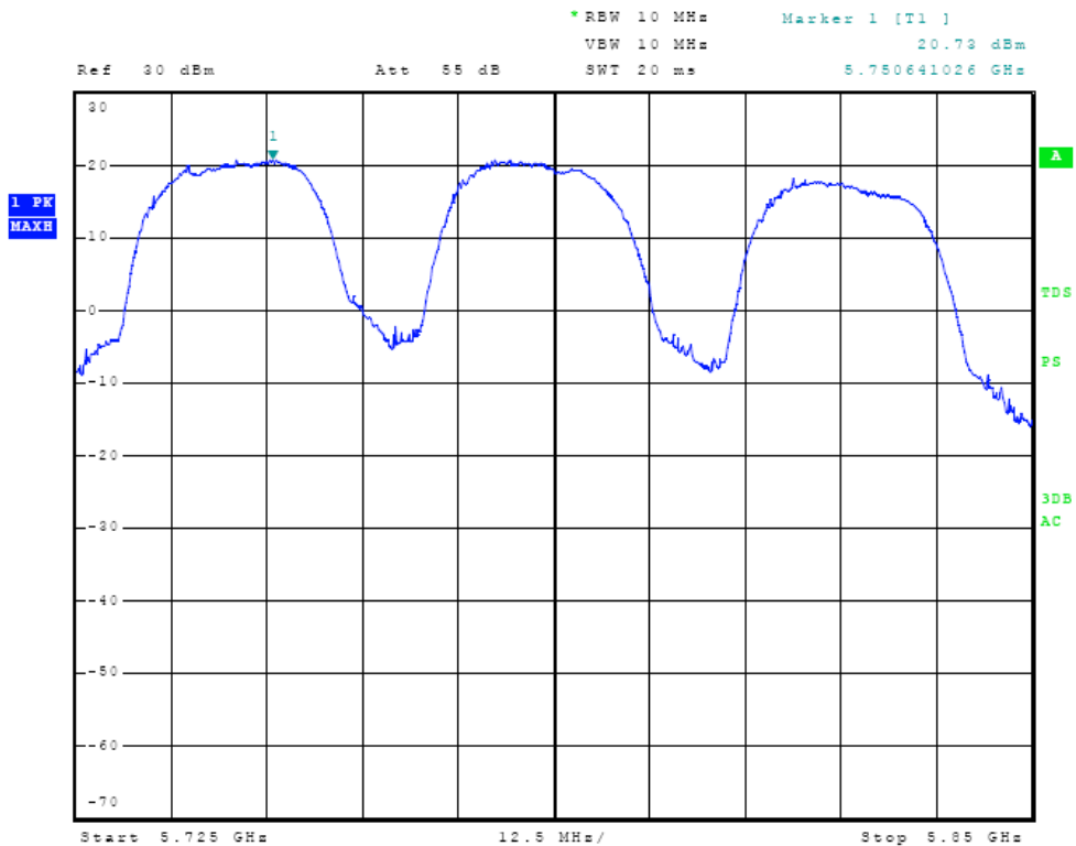
Figure Sixteen Plot of Power Output Across Operational Band
