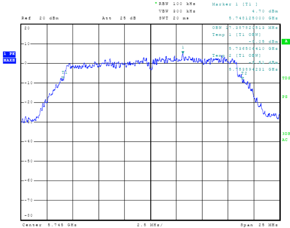
Figure Seventeen Plot of 6 dB Band width
