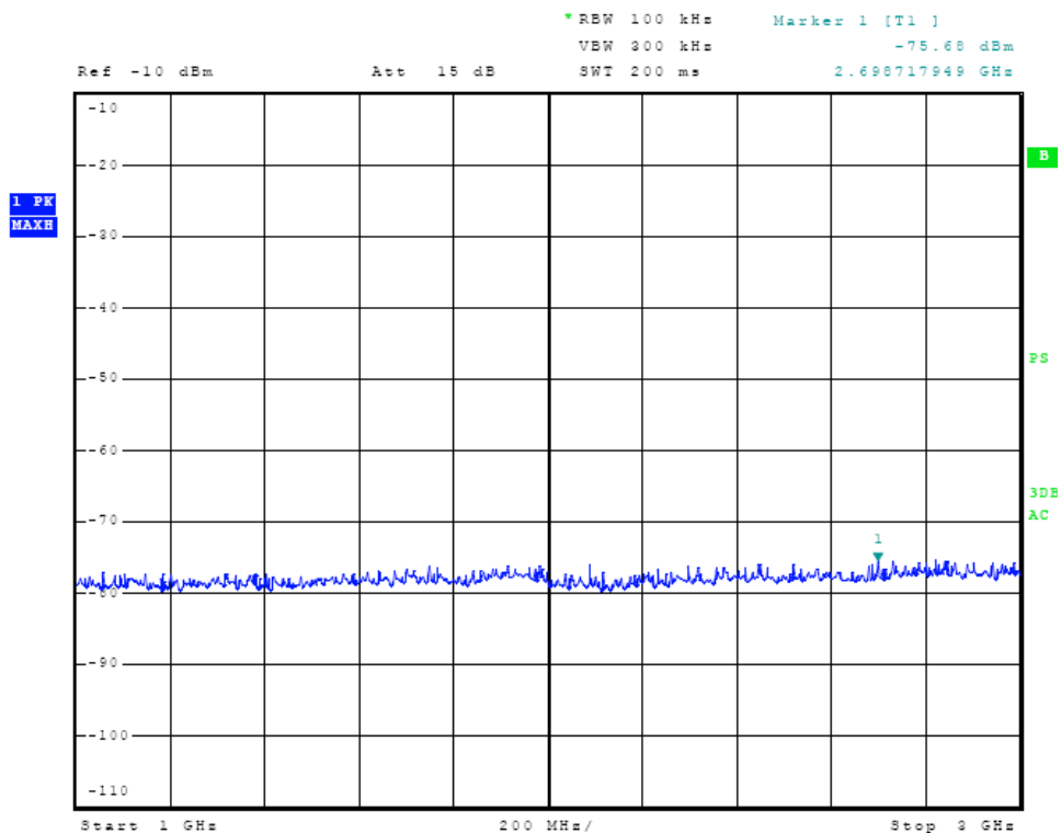
Figure Twenty-five Receiver Antenna Port Conducted Emissions
