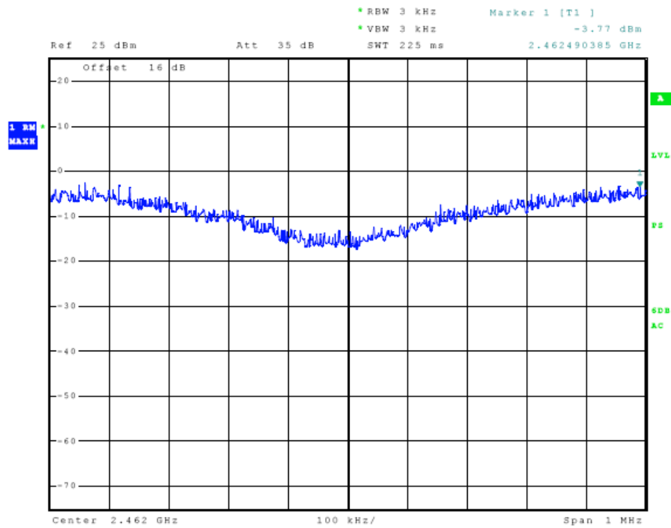
Figure Twenty-three Plot of Power Spectral Density
