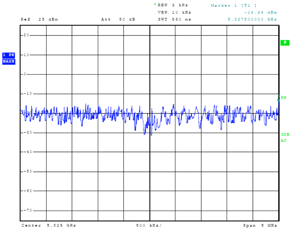
Figure Twenty-two Plot of Power Spectral Density
