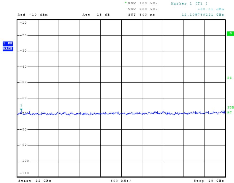
Figure Twenty-eight Receiver Antenna Port Conducted Emissions
