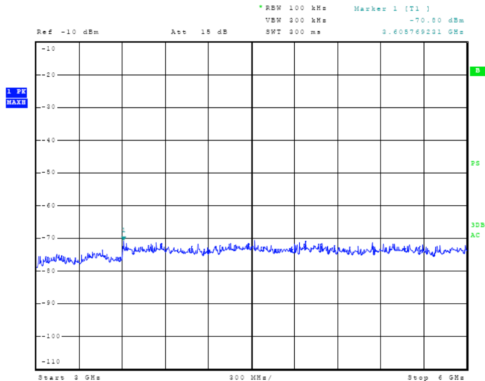
Figure Twenty-six Receiver Antenna Port Conducted Emissions
