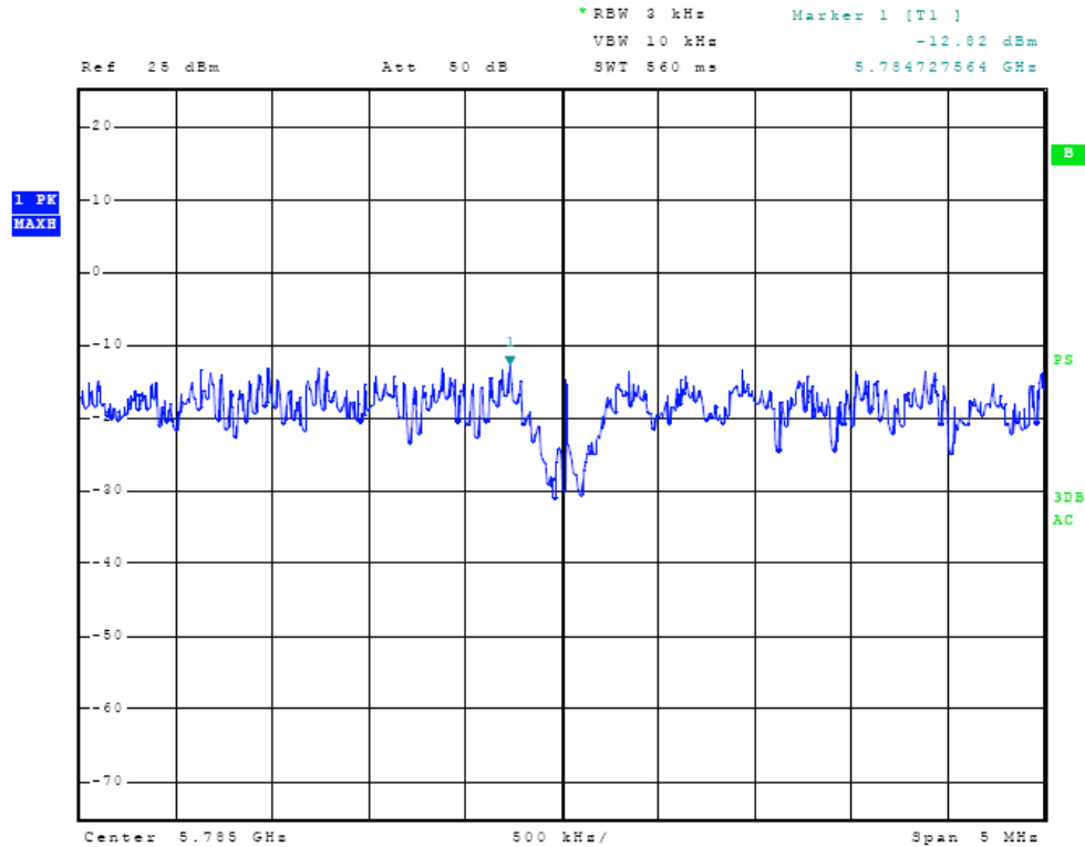
Figure Twenty-one Plot of Power Spectral Density
