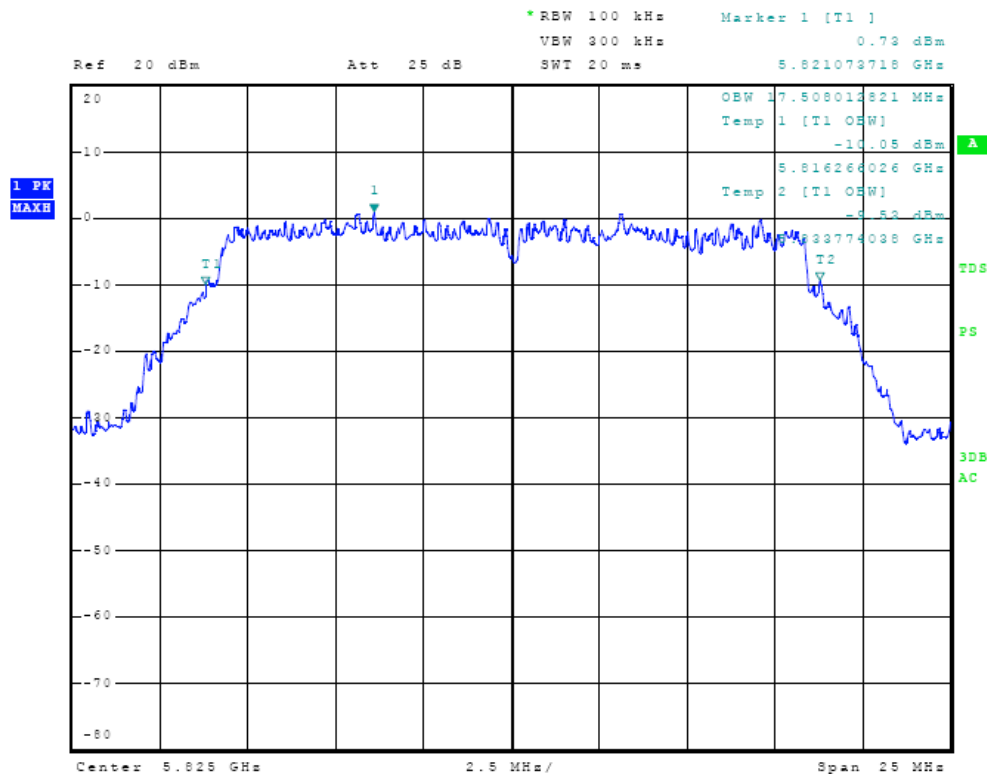
Figure Nineteen Plot of 6 dB Band width
