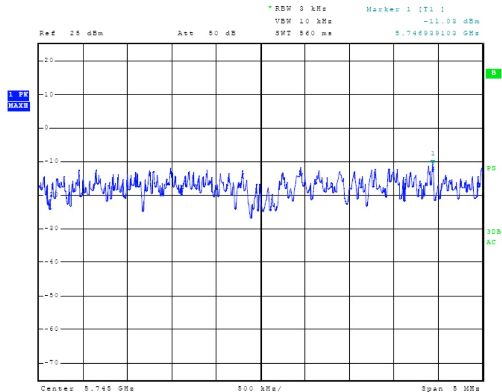
Figure Twenty Plot of Power Spectral Density
