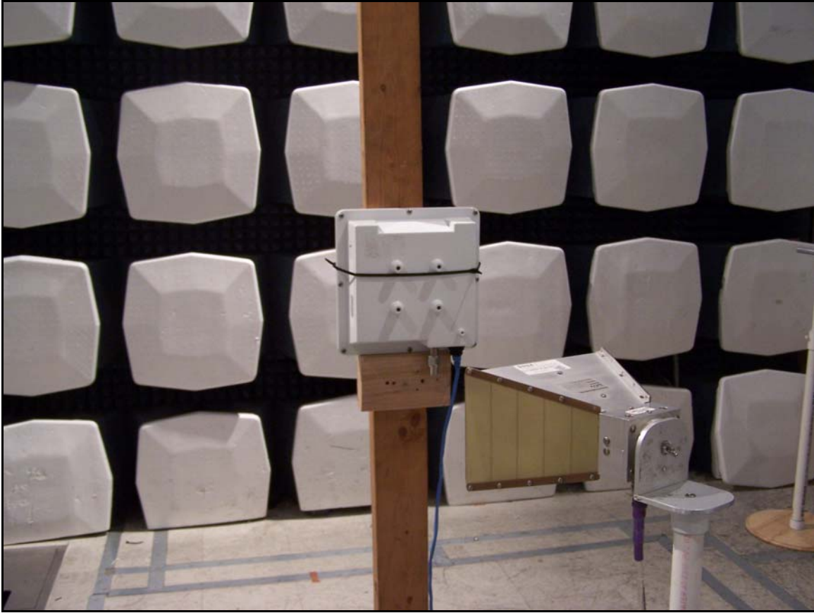
Photograph 4. Spurious Radiated Emissions, Test Setup
