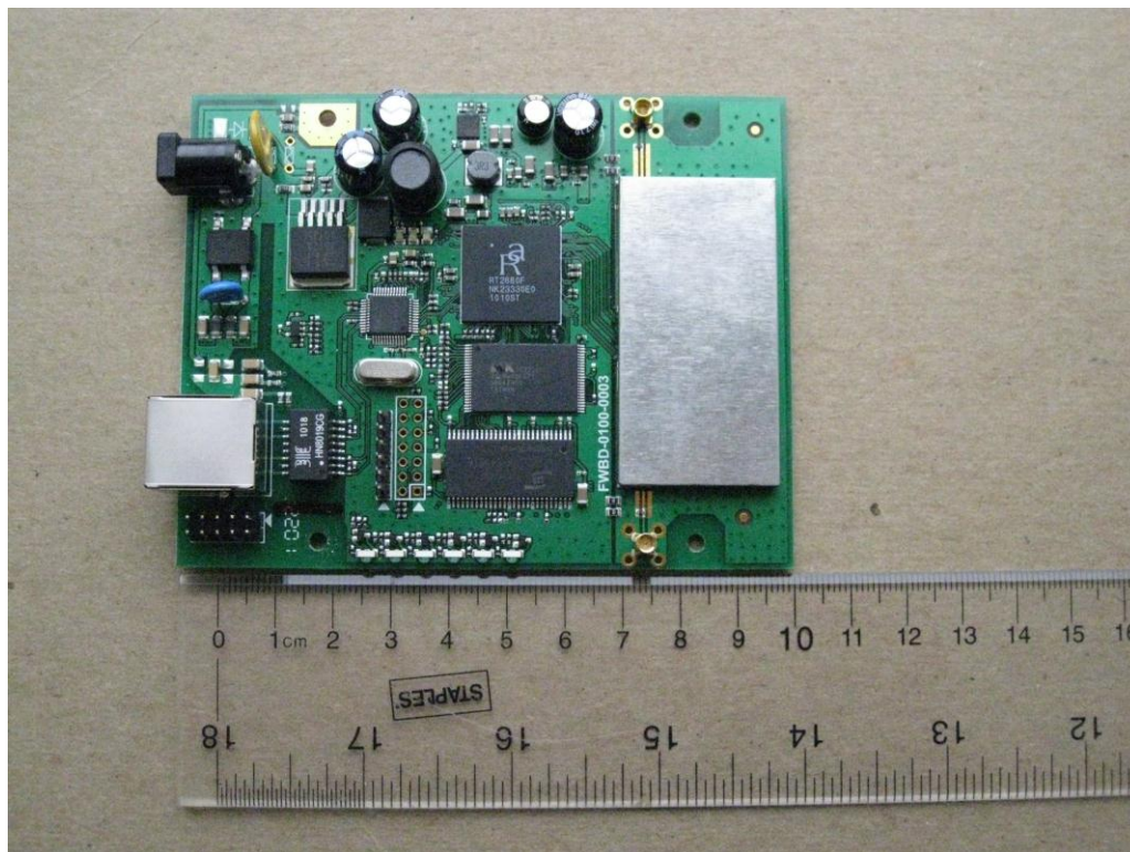
Printed Circuit board with cover
