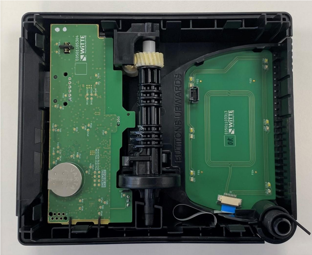
flinkey CAN enclosure lower part without keybed
