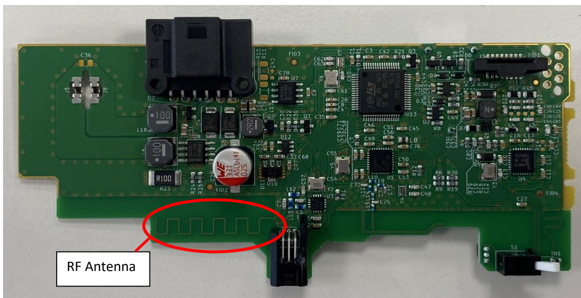
flinkey CAN Main PCB bottom side
