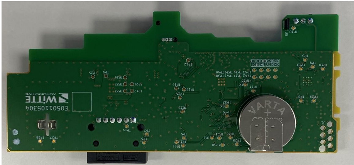
flinkey CAN Main PCB top side
