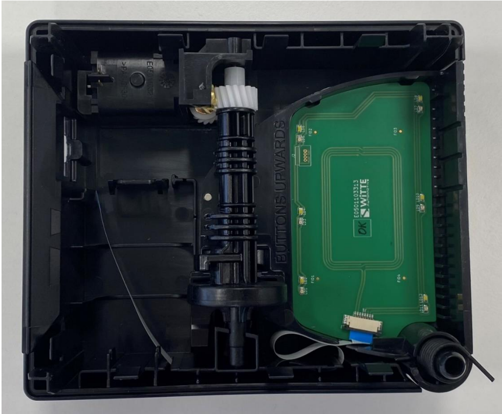
Flinkey CAN lower part without main PCB
