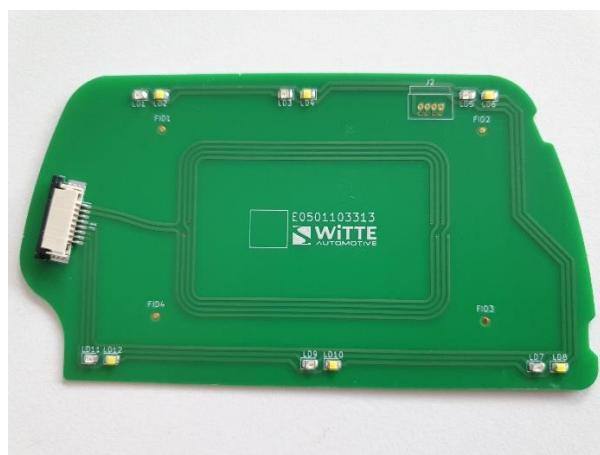
flinkey CAN Keybed PCB top side
