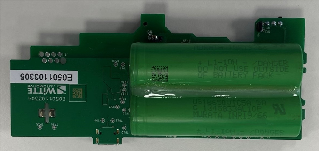
flinkey CAN Main PCB top side
