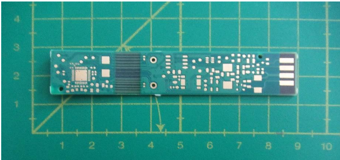
Photograph 2: PCB of the EUT, bottom view
