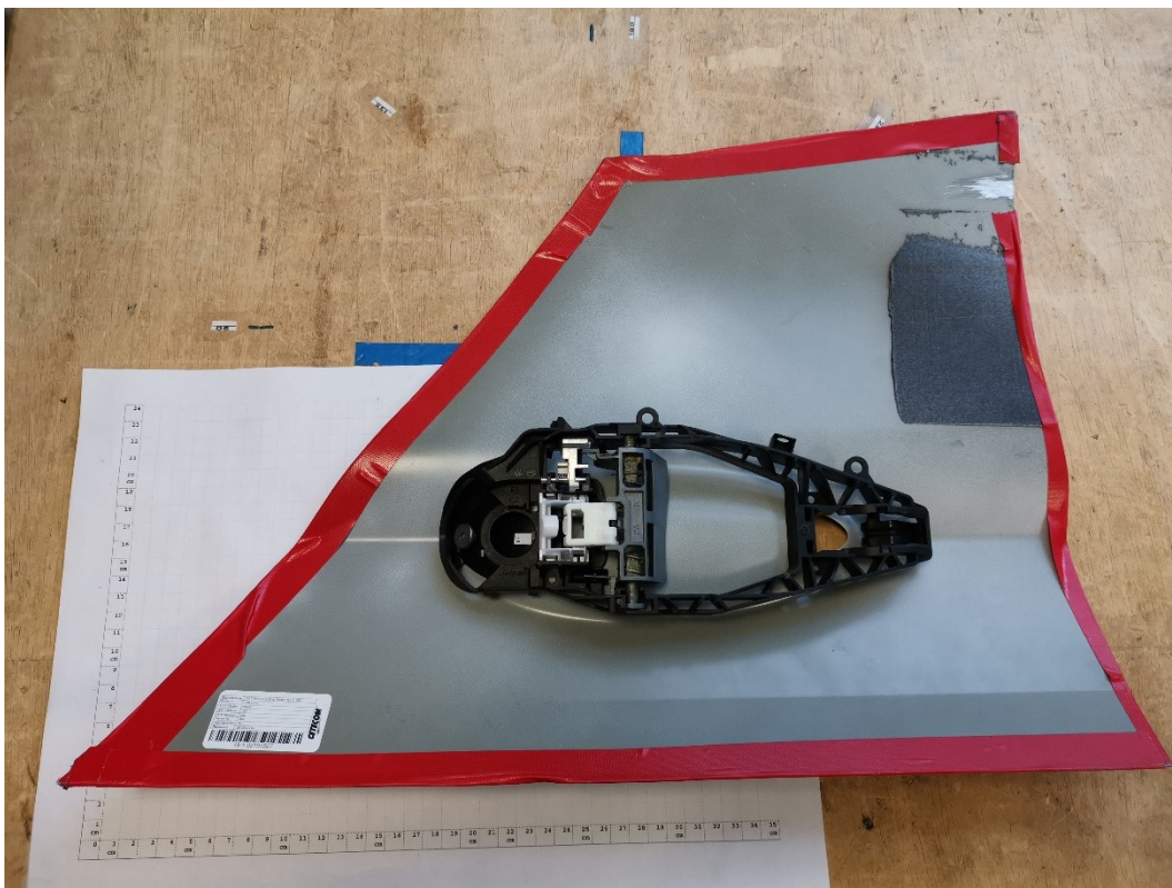
Photograph 6: AE 1, rear view
