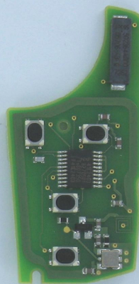
4 Button 433.92MHz
