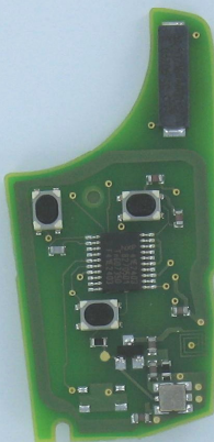
3 Button 433.92MHz
