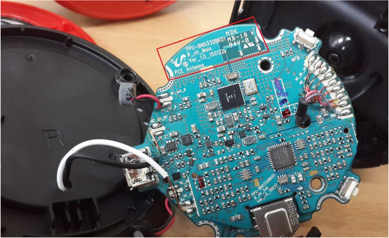
BT Antenna
