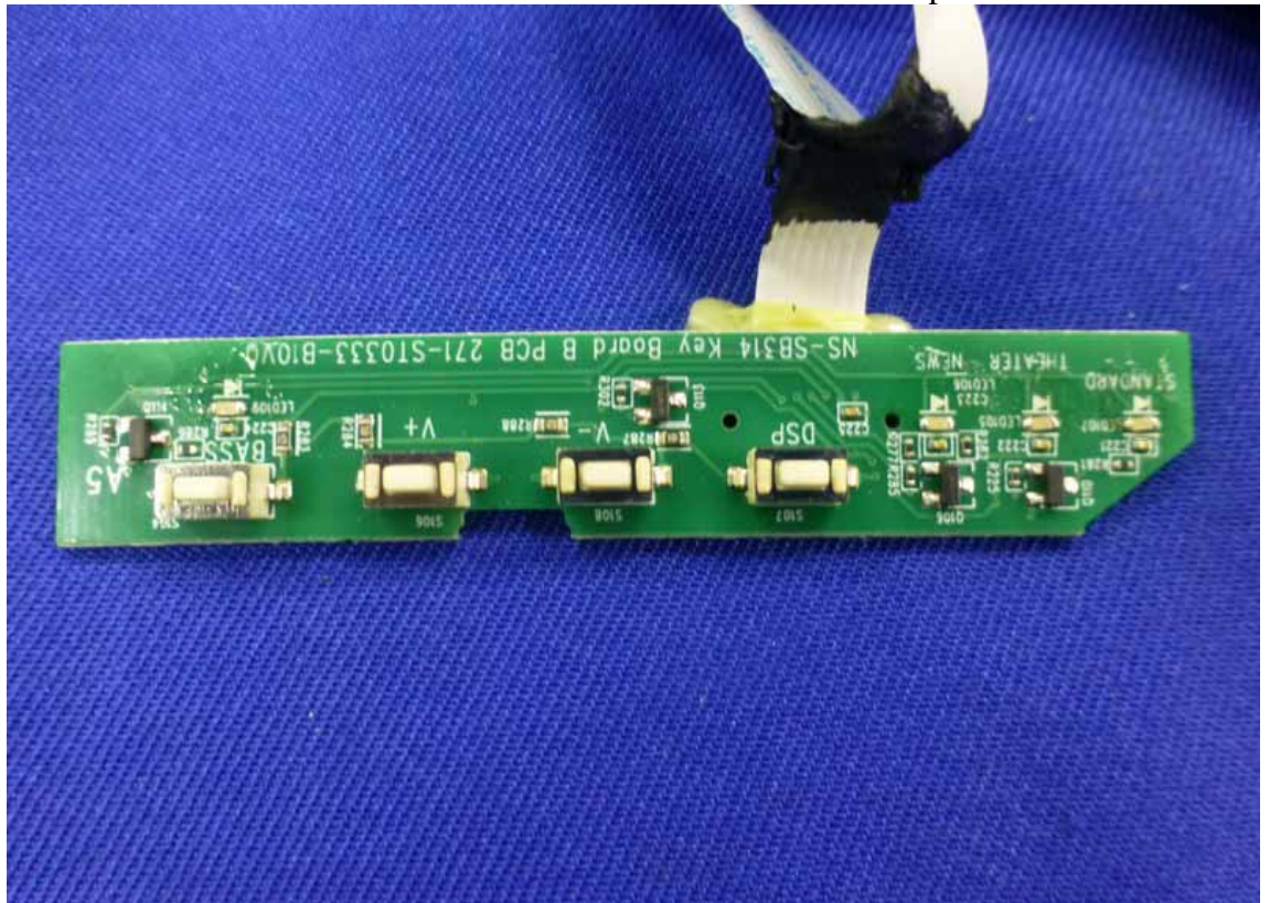
Figure 16 Component of the PCB Board
