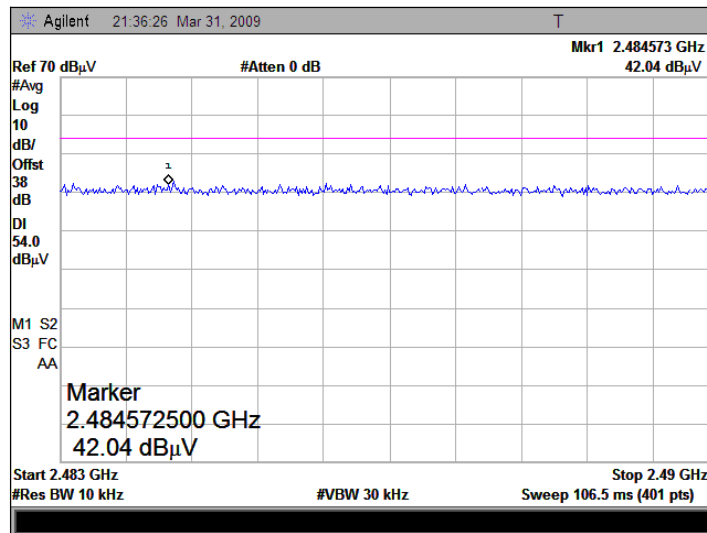
(Plot B2: Channel = 78 AVERAGE)
