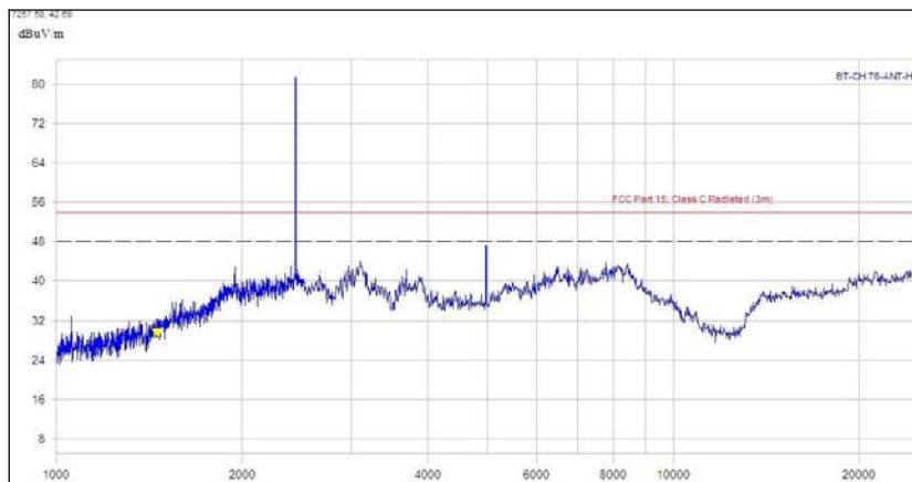
(Plot C.3: Antenna Horizontal, 1GHz to 25GHz)
