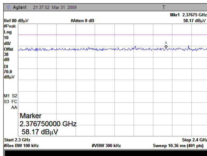
(Plot A1: Channel = 0 PEAK)
