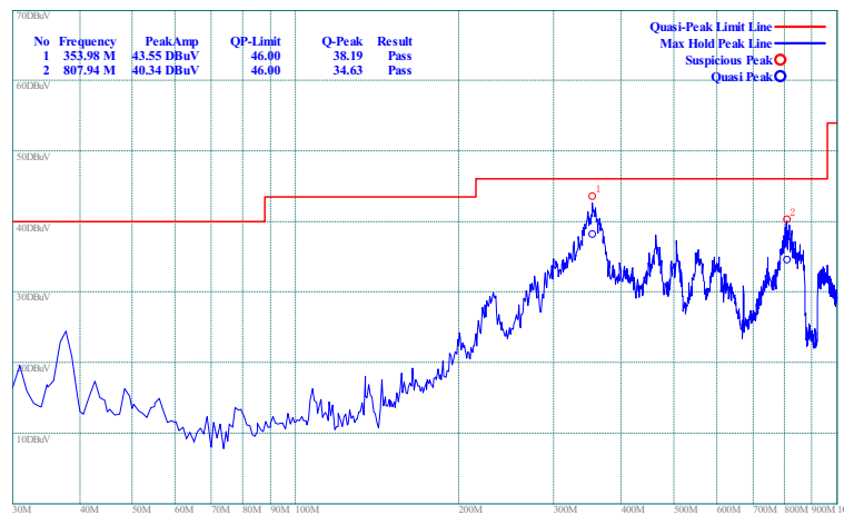
(Plot C.4: Antenna Vertical, 30MHz to 1GHz)
