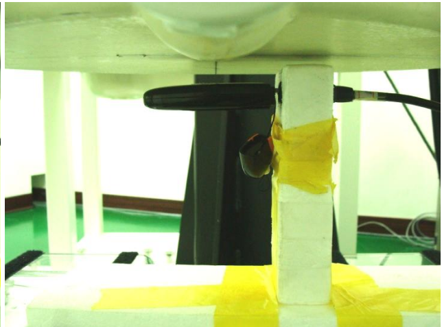
USB Configuration 2 with Cable (Horizontal Down with Phantom 1.5 cm Gap)
