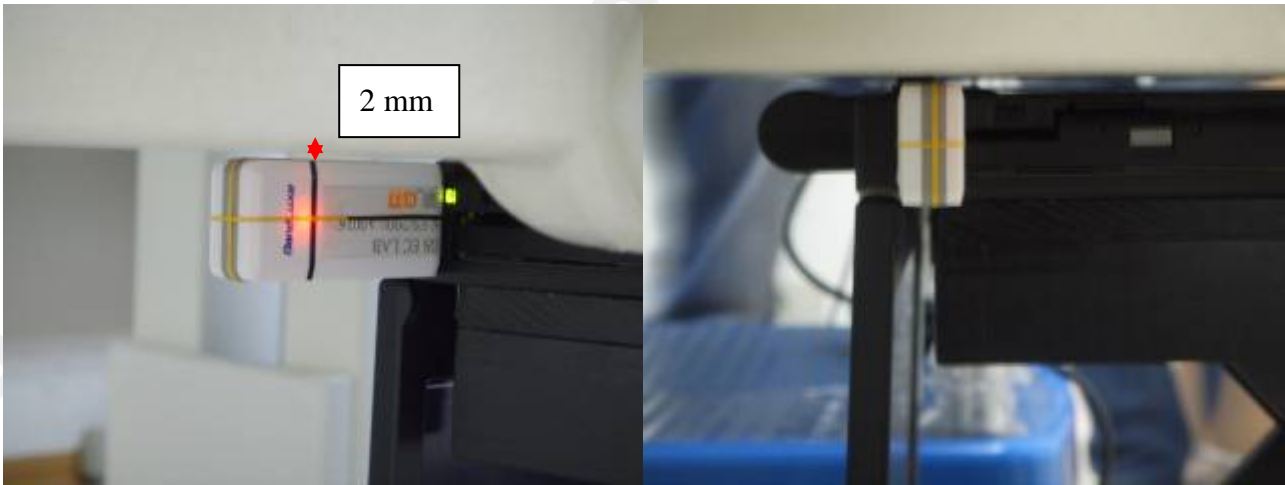
Fig 6 : Bottom side of the Notebook is paralleled and contacted with flat phantom, and right side of the EUT is paralleled with flat phantom.
