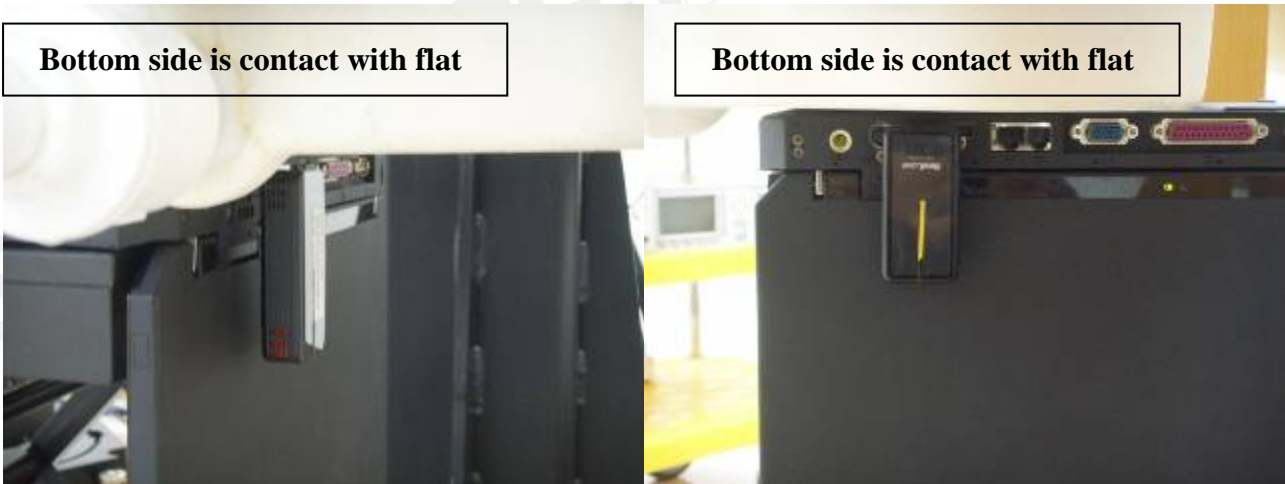
Fig7 : Bottom side of the Notebook is paralleled and contacted with flat phantom.
